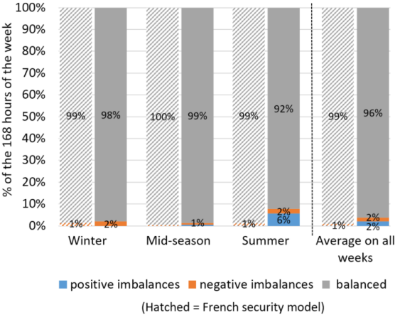
Figure 33: Average distribution of the week according to the sign of the aggregated imbalances of all BRPs after the intraday market for each type of week
