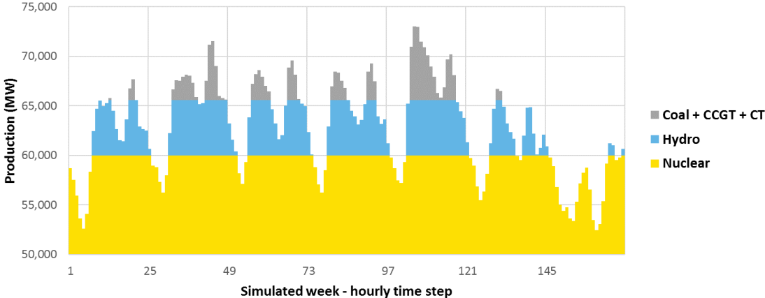
Figure 83: Illustration of the simplified merit-order without considering technical constraints for one winter week
