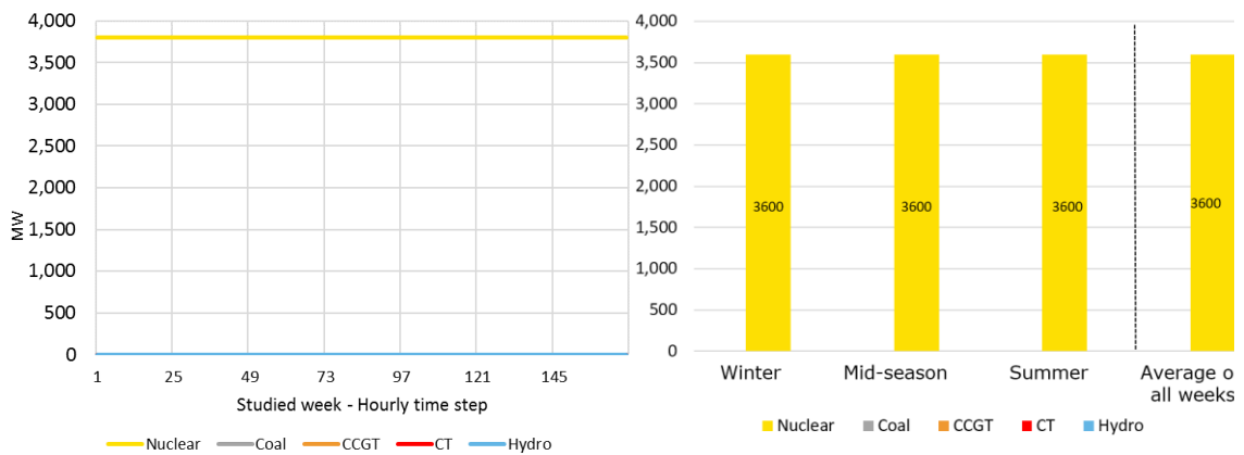
Figure 86: Technology identified to provide downward RR for one winter week Figure 87: Average procured downward RR for each technology and each type of weeks
