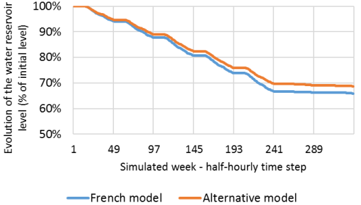
Figure 99: Evolution of the water reservoir level for one summer week
