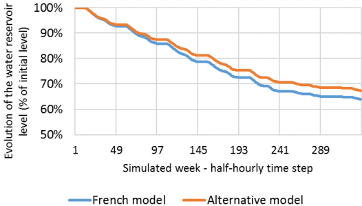
Figure 97: Evolution of the water reservoir level for one mid-season week
