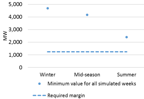
Figure 90 : Minimum downward margins for each type of weeks
