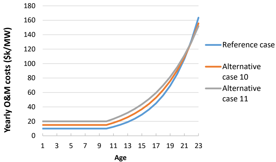
Figure 75: O&M costs considered for the alternative cases 10 and 11
