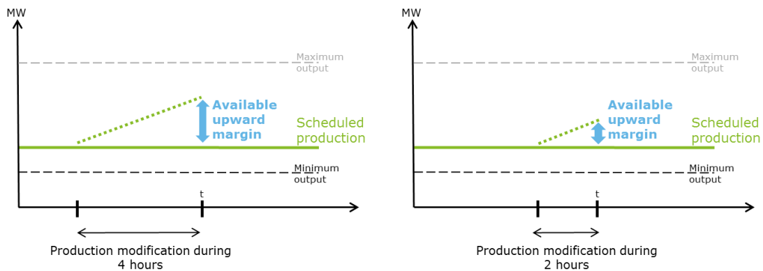
Figure 7: Evolution of the available upward margin when approaching real time - illustration
