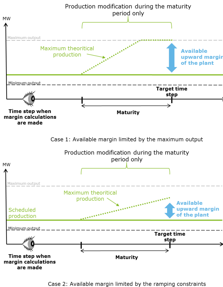
Figure 17: Illustration of the available upward margin for an online plant in two cases
