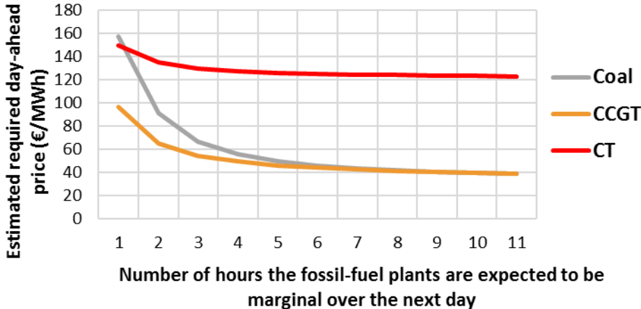
Figure 84: Simplified estimation of the required day-ahead prices for thermal plants depending on the numbers of hours they are expected to be marginal over the next day. Approximate values are shown in figure 84 for the three fossil-fuel technologies. It can be read as follows: if fossil-fuel plants are expected to be marginal during one hour for the next day, a CCGT plant will require the day-ahead price to be around 100€/MWh
