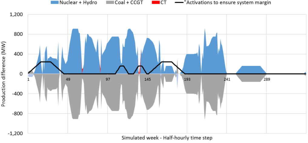
Figure 94: Production difference for one mid-season week
