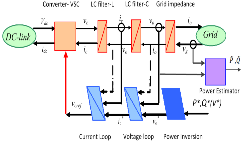
Figure A.4: EMR and Inversion Based Control Strategy
