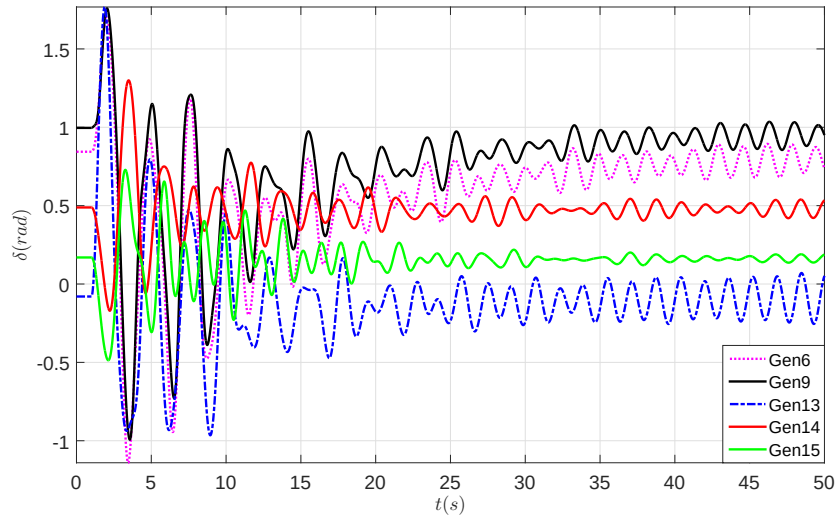
Figure 4.4: Example Case 4: Simulation of Rotor Angles' Dynamics of the New England New York 16-Machine 5-Area System
