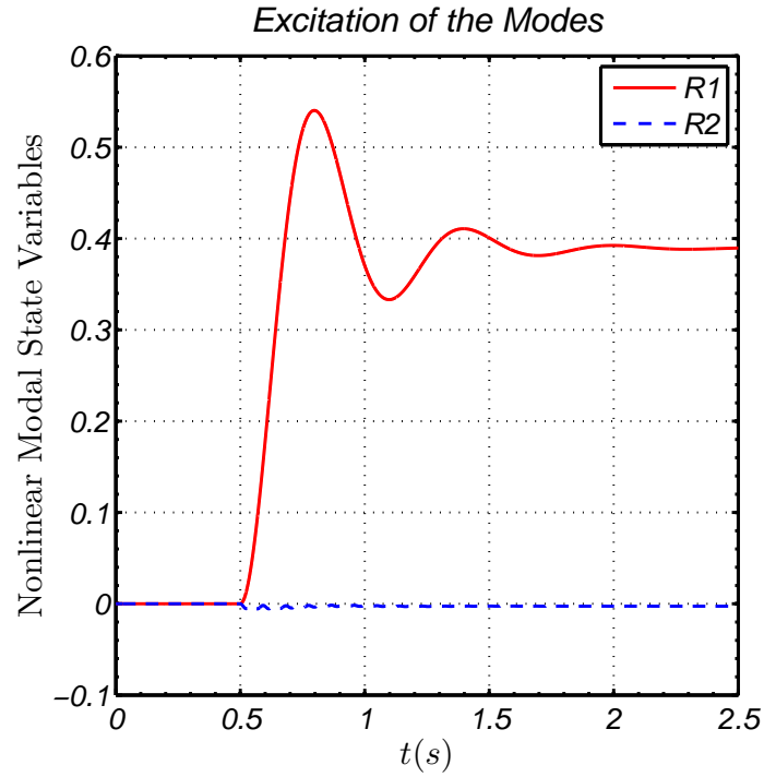
Figure 5.10: Decomposition the Modes under Excitation: R_1, R_2
