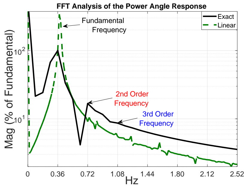
Figure 1.15: Example Case 2: Linear Small Signal Analysis of Stressed Power System Under Large Disturbance
