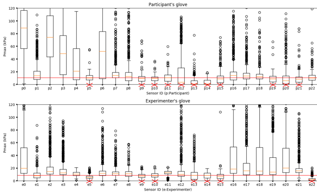
FIGURE B.1: Box-plots of the maximum pressure in the 46 sensors of the 2 human-sized gloves. The data collected is from the experiment presented in Chapter 5
