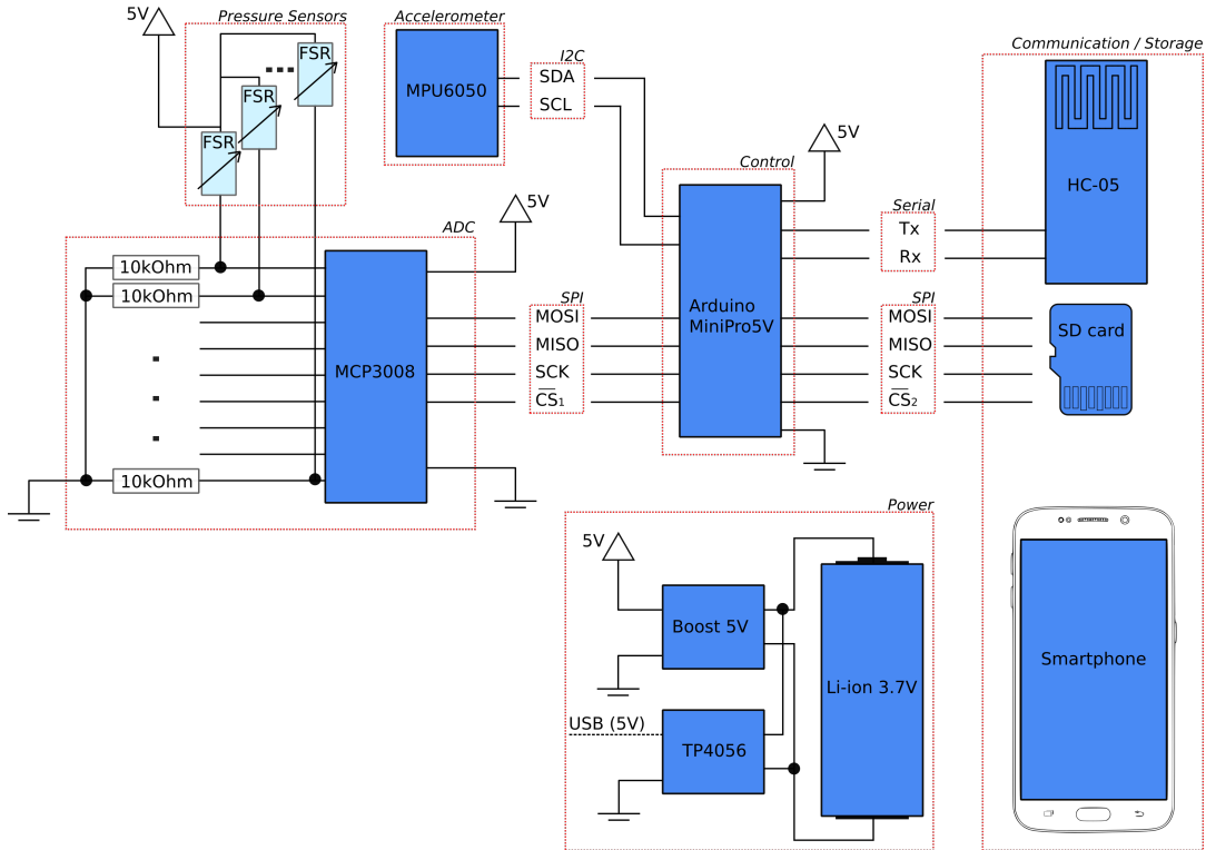
FIGURE 3.7: Electronics diagram
