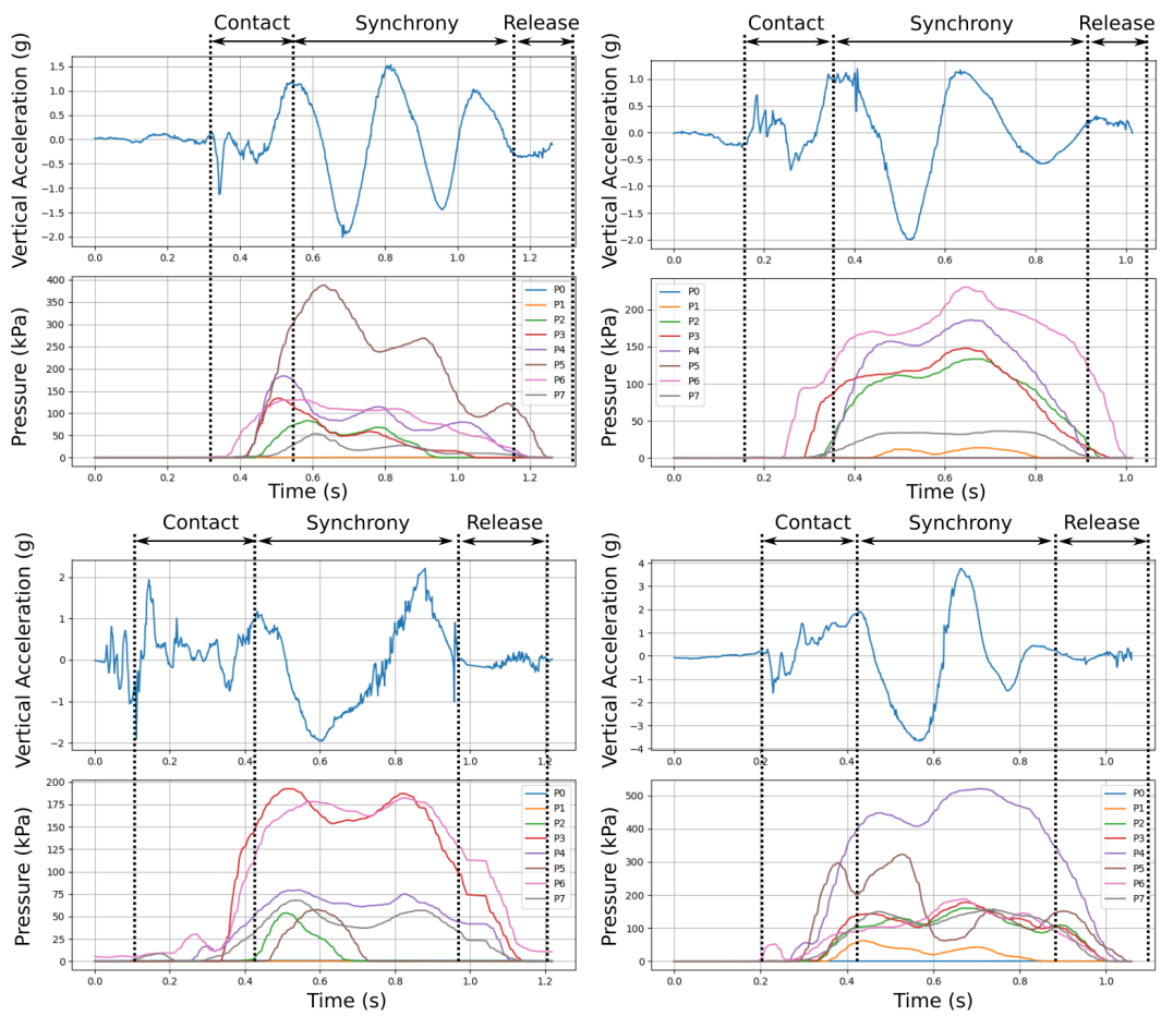
FIGURE 3.8: Examples of handshake data, for 4 handshakes with different participants
