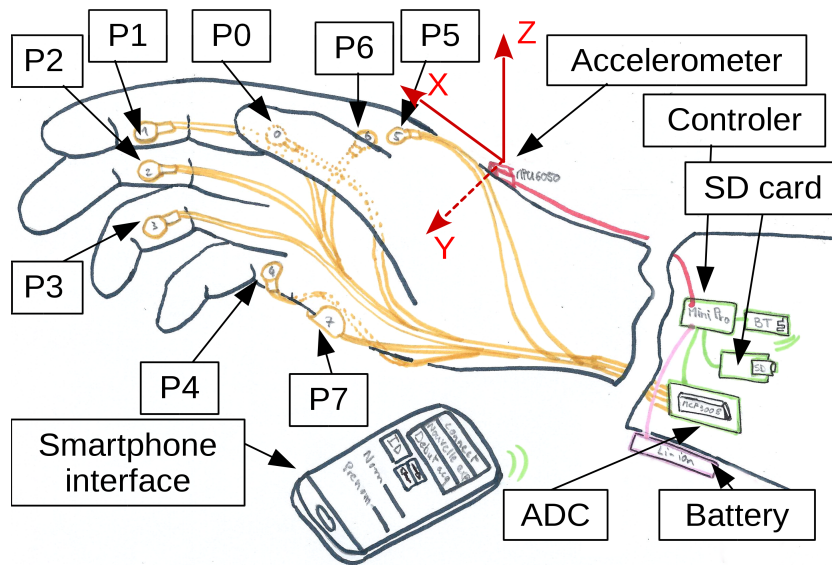
FIGURE 3.5: The glove components and definition of the coordinates
