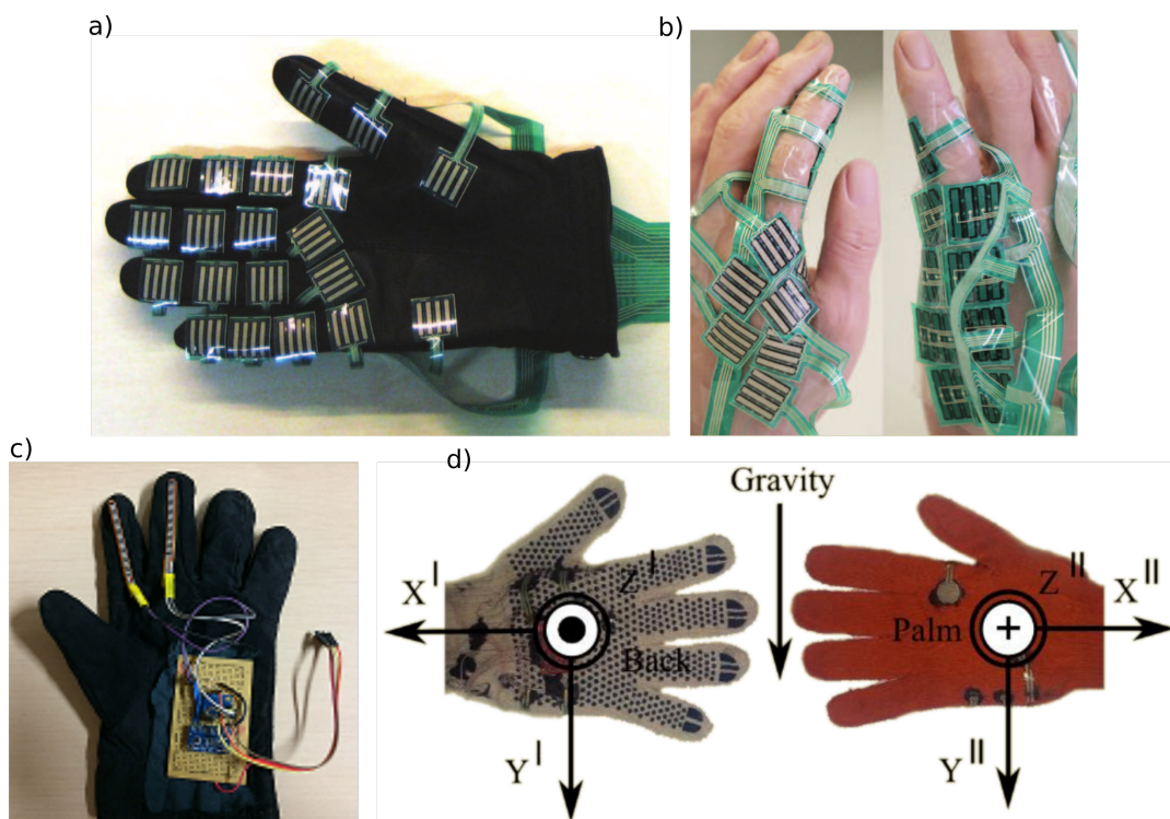
FIGURE 2.11: Examples of gloves that use pressure sensors. a) Extracted from Wang, Hoelldampf, and Buss, 2007, and b) the modified version for handshake measures; c) Extracted from Garg, Mukherjee, and Rajaram, 2017; d) Extracted from Melnyk et al., 2014
