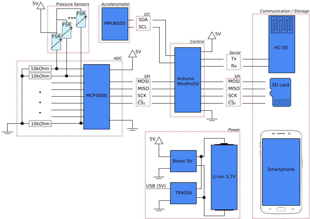
FIGURE 3.7: Electronics diagram
