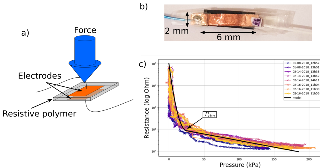
FIGURE 4.9: Design of the piezo-resistive sensors. a) Operating principle, b) picture, and c) calibration laws with corresponding model for one sensor.
