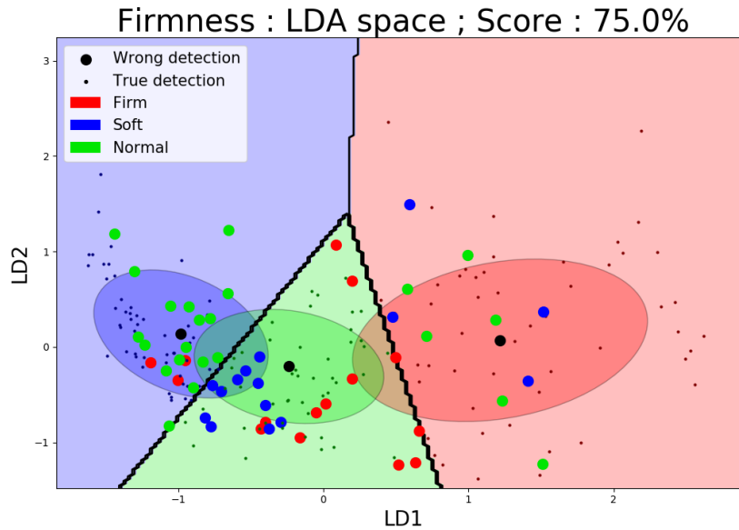
FIGURE 3.10: LDA space for firmness discrimination. The small dots represent the true detections, the large ones represent the wrong detections. The dot's color indicates the real category of the sample. The colored areas are the calculated class attribution from the LDA model.
