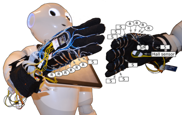
FIGURE 5.1: Sensor positions on the Pepper's glove.
