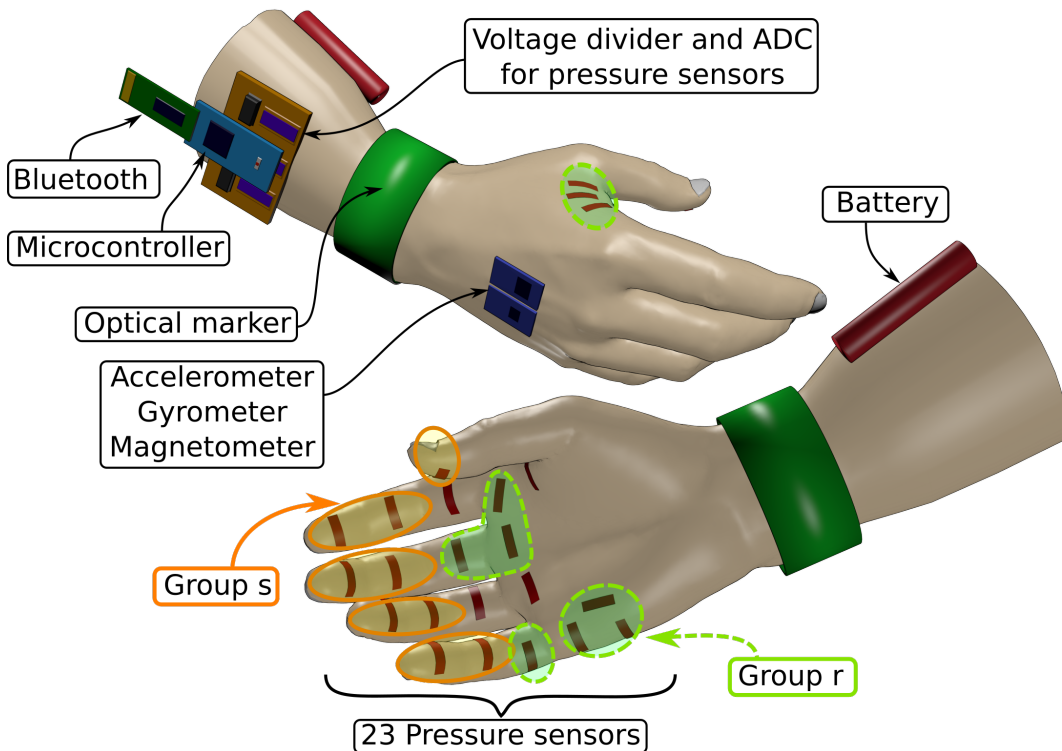
FIGURE 4.10: Glove schematic and sensor positions (here the participant's glove). The sensor groups are described in Chapter 3 Section 3.3: group s on participant's glove in orange and group r in green dot-line.
