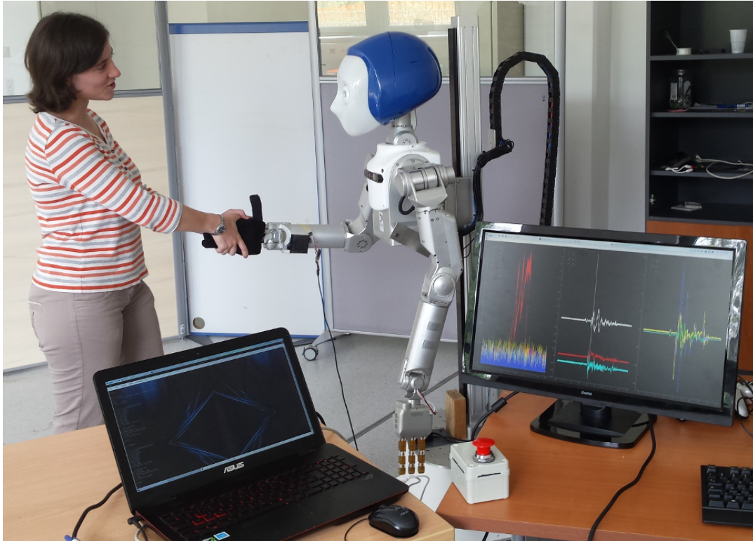
FIGURE 3.14: Human-Robot handshake using Meka humanoid robot
