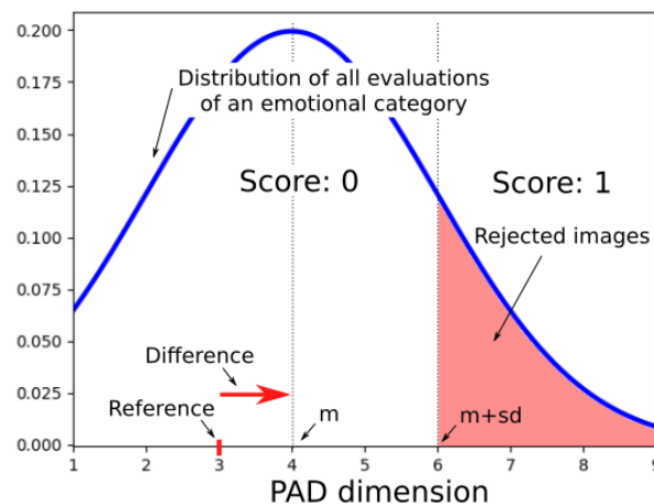
FIGURE 4.7: PAD distance score attribution method for images
