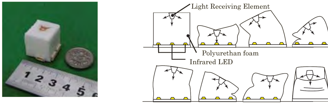
FIGURE 2.3: 3D optical piezo-sensitive cell (extracted from Kadowaki et al., 2009)
