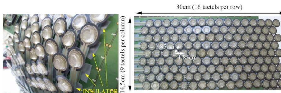
FIGURE 2.7: Piezo-resistive cells assembled in a skin (extracted from Vidal-Verdú et al., 2011)
