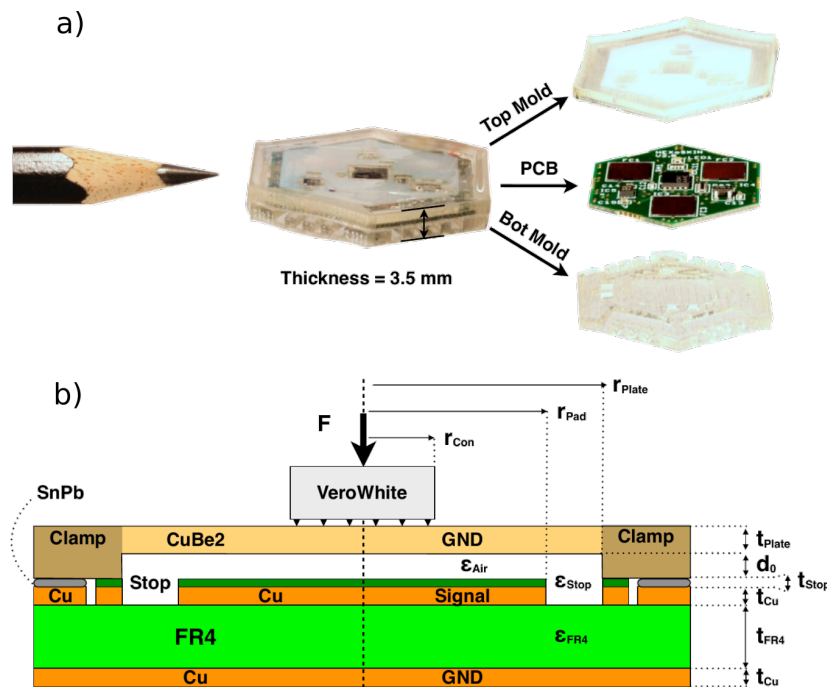
FIGURE 2.10: Modular multi-modal sensor (extracted from Mittendorfer and Cheng, 2012). a) Picture of the full module; b) Schematic of a Piezo-capacitive cell.
