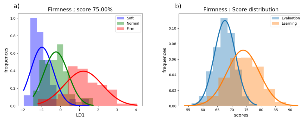
FIGURE 3.11: a) Distribution of the projected data on LD1 depending on the firmness. b) Distribution of the detection scores for the learning sets and evaluation sets.
