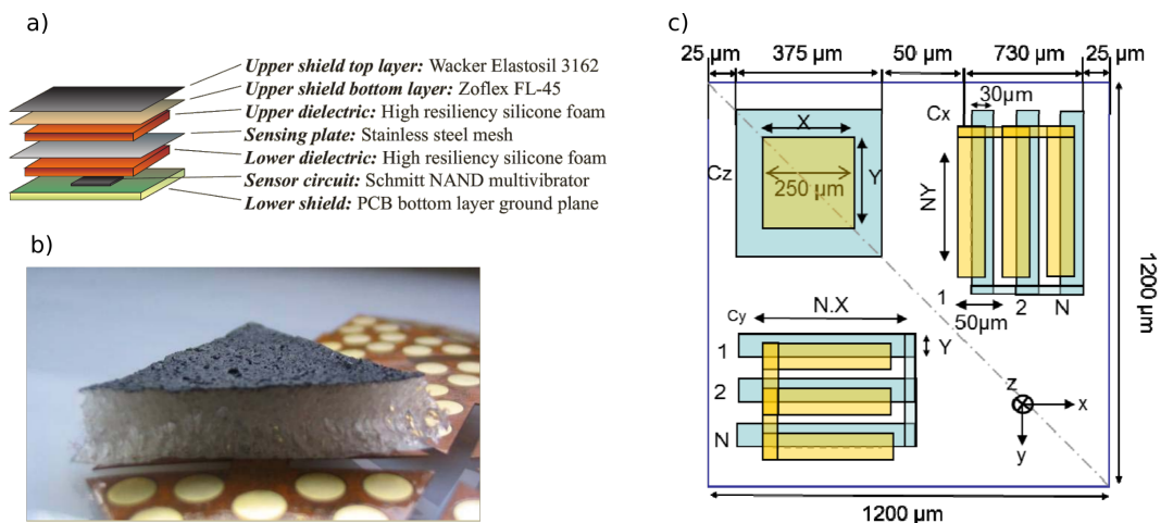
FIGURE 2.6: a) Schematic of a piezo-capacitive cell (extracted from Ulmen and Cutkosky, 2010); b) Picture of a module with 12 piezo-capacitive cells (extracted from Cannata et al., 2008); c) Schematic of a 3D piezo-capacitive cell, composed with 3 sub-cells (extracted from Nazeer, 2012)
