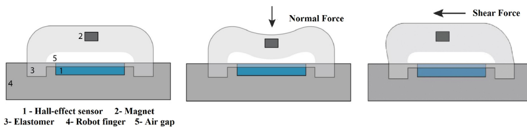
FIGURE 2.4: 3D magnetic piezo-sensitive cell (extracted from Paulino et al., 2017)
