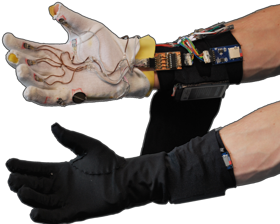
FIGURE 3.6: Glove pictures (top: without the cover layer; bottom: with the cover layer)
