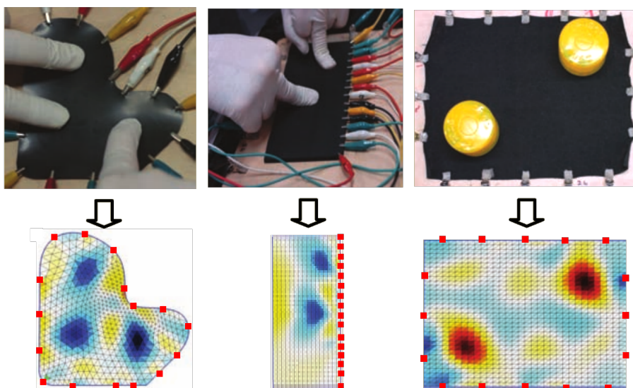
FIGURE 2.9: Examples of Electrical Impedance Tomography (EIT) sensors (extracted from Alirezaei, Nagakubo, and Kuniyoshi, 2007).
