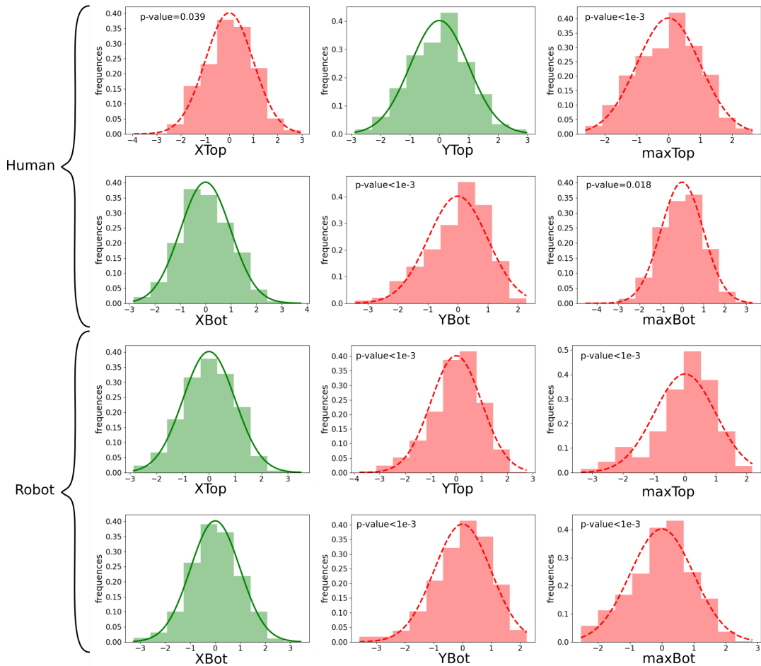
FIGURE 5.7: Distribution on the 6 standardized components, for both agents datasets. In green the histograms when the distribution is Gaussian, in red-dashed when it is not normal. The associated Shapiro p values are specified.
