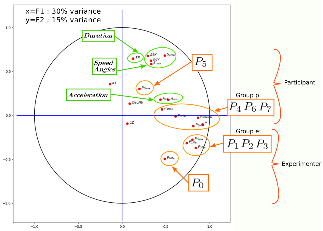
FIGURE 3.9: Correlation circle of the features
