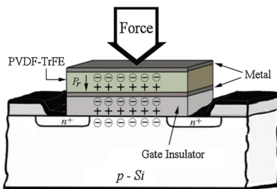
FIGURE 2.5: Schematic of a piezo-sensitive cell based on FET transistor (extracted from Adami et al., 2012)
