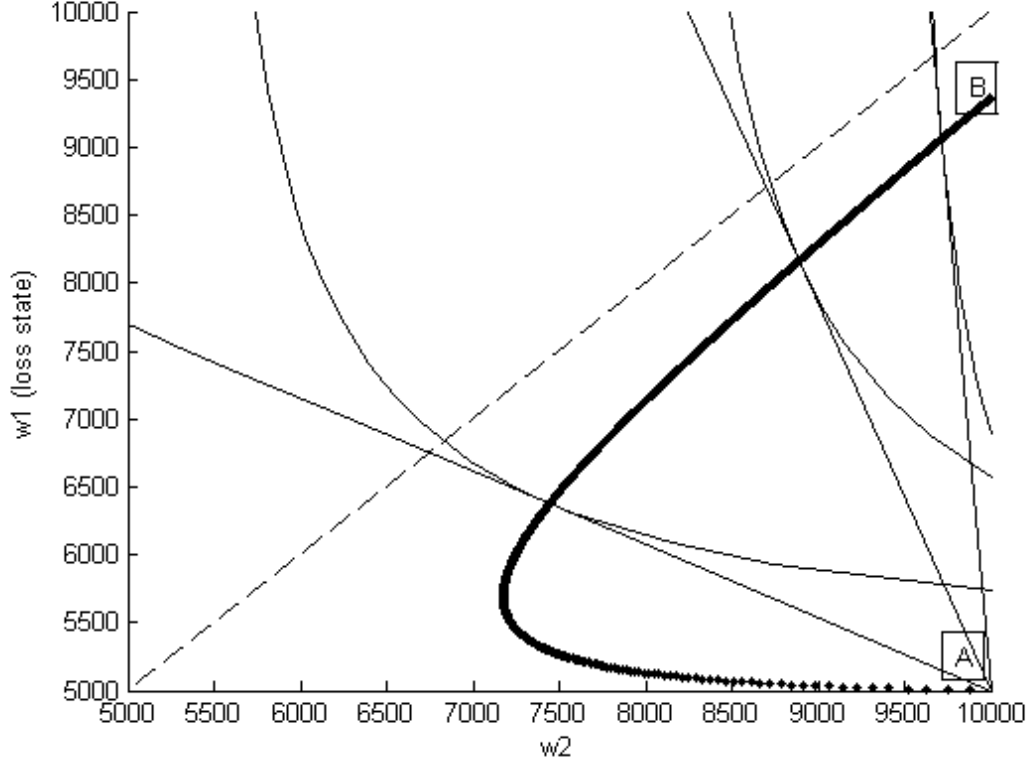
Figure 2.2: w = 10000, L = 5000, u(x) = \frac{x^{-3}}{3}
