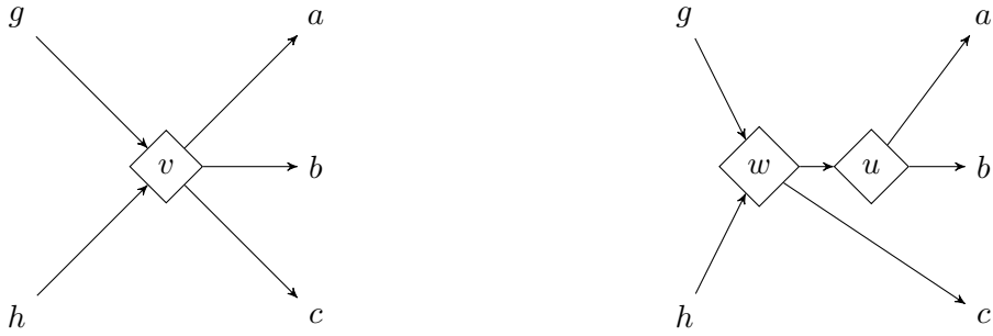
Figure 5.4: Lowering the degree. Random vertices are depicted by diamonds.
