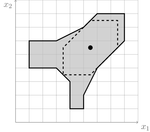
Figure 8.2: Tropical spectrahedron and its maximal inner Hilbert ball (for x_0 = 0 ).
