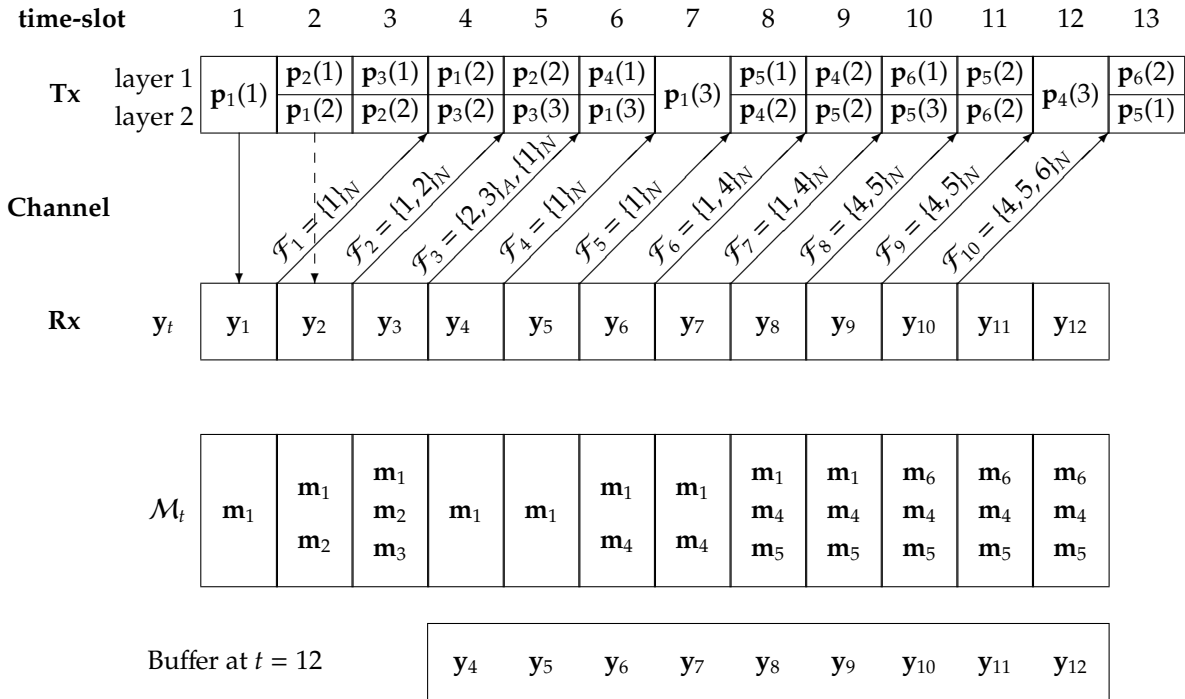
Figure 2.5 – Receiver's buffer during an instance of the proposed protocol.
