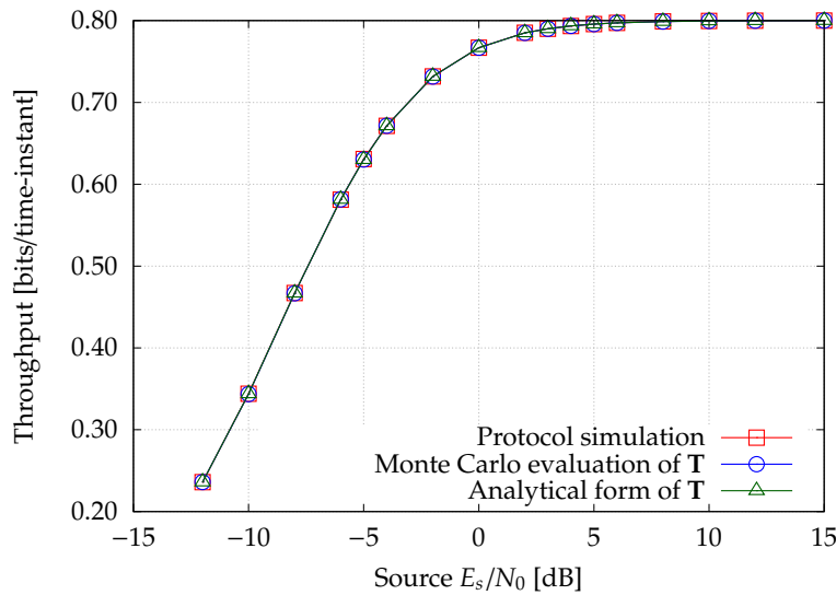
Figure 1.14 – Throughput validation of the investigated protocol.
