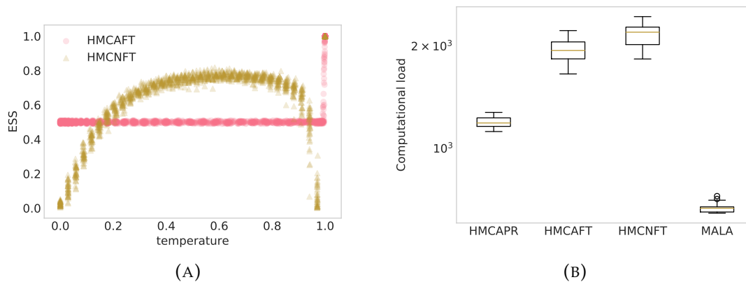
FIGURE 5.2: ESS and temperature steps in dimension d = 500 (Figure 5.2a) and the computational load of the sampler in terms of the number of total gradient evaluations (Figure 5.2b).
