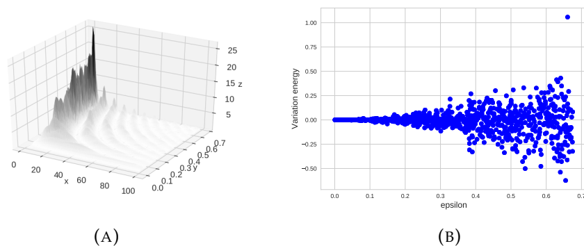
FIGURE 5.1: Tempering of a normal distribution to a shifted and correlated normal distribution in dimension 10 (see the example in Section 5.4.1 for more details). Left: The normalized and weighted squared jumping distance (z-axis) as a function of \epsilon (y-axis) and L (x-axis) for the temperature 0.008. Right: Variation of the difference in energy \Delta E as a function of \epsilon for the same temperature. The values of L are randomized. Based on an SMC sampler with an HMC kernel based on N = 1,024 particles.
