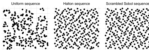
FIGURE 4.1: MC (left), QMC (center) and RQMC (right) sequences of length N = 256 on [0, 1]^2 . QMC and RQMC tend to cover the target space more evenly.
