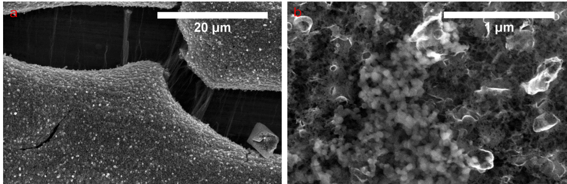
FIGURE 3.6: SEM images of S NPs cathode on VACNT carpets.
