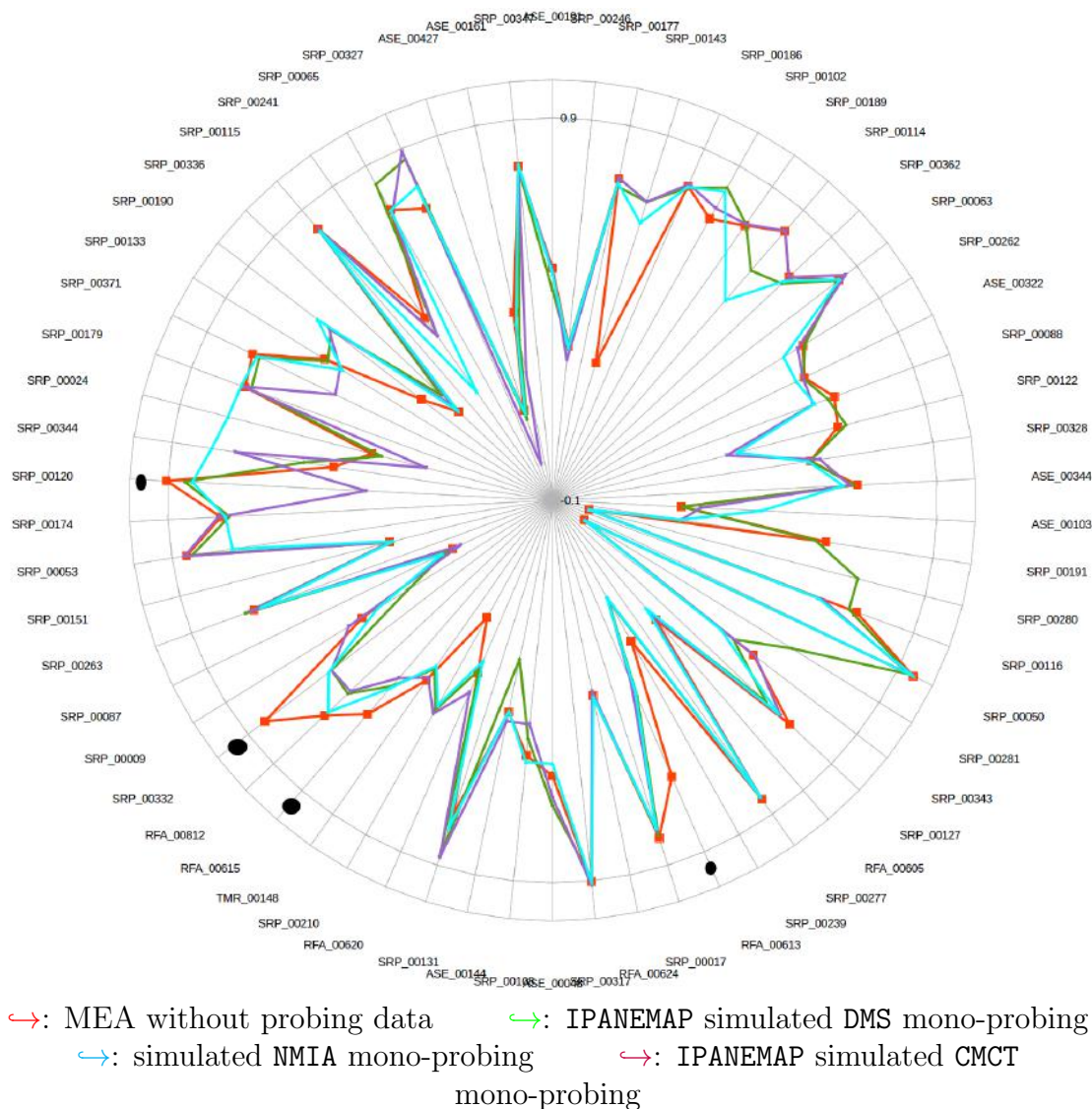
Figure 7.7: Accuracy of predicted structures in mono-probing case using IPANEMAP with simulated data: with the exception of a few RNAs, a comparable if not a better performance is observed when using IPANEMAP, with one of the simulated probing data, compared to the predicted MEA with RNAfold . Circles in black shows the cases where the MEA is performing better than IPANEMAP with one probing data.
