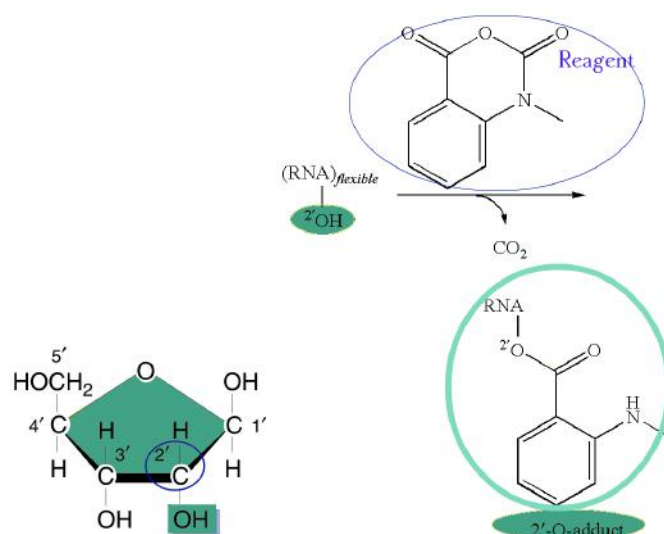
Figure 2.4: SHAPE reagent interaction with the nucleotide ribose: In the left, a nucleotide ribose where the OH component at the 2' position is highlighted. In the right, the reaction of the SHAPE reagent with one molecule of RNA induce the formation of an adduct.
