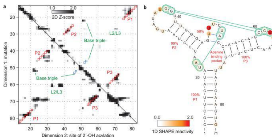
Figure 2.7: M&M 2D plot and the resulting predicted structure for add. riboswitch : the entire M&M data set across 71 single mutations, plotted in grey scale and the Secondary structure derived from incorporating Z-scores (the number of standard deviations from mean at each residue) into the RNAstructure modeling. Squares show secondary structure model guided by M&M data( red, match to crystallographic Watson-Crick stems; blue, match to non-Watson-Crick stem). Additional tertiary contacts inferred from a separate clustering analysis are given in green. The figure was imported from [Kladwang et al., 2011].
