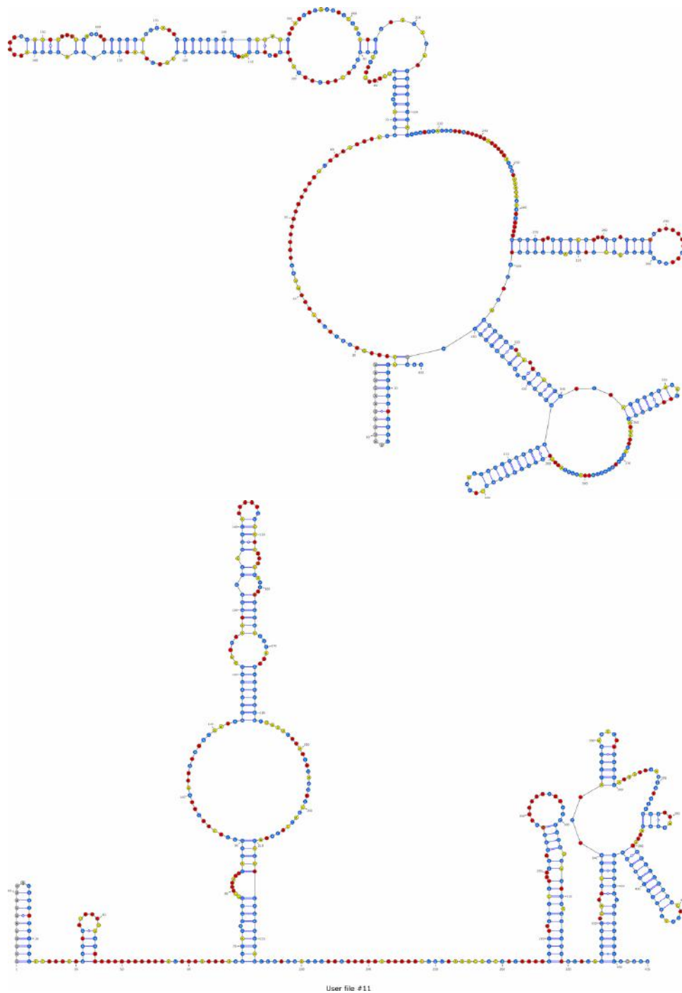
Figure 8.10: Candidate structure(s) for the 5' UTR of the NP gene, predicted using IPANEMAP: IPANEMAP identified 20 dominant clusters. Two clusters were found to be optimal: One cluster has two representative conditions 1M7Mg and 1M7, the resulting centroid is illustrated on the left. The second cluster has MSA as dominant condition with the ensuing centroid presented on the right. Nucleotides are color-coded based on their normalized SHAPE reactivities ( \leq 0.4 \rightarrow blue, \geq 0.7 \rightarrow red, mid range \rightarrow yellow; missing values in gray)
