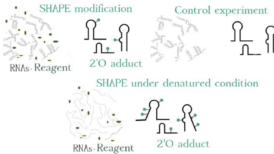
(a) SHAPeMap chemical experiments under a SHAPE, a control and a denatured conditions.
