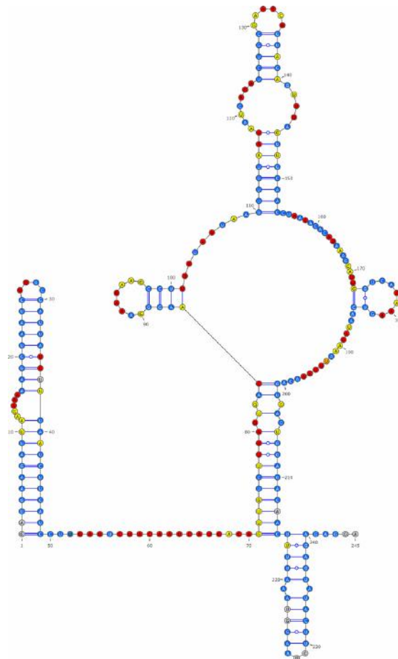
Figure 8.18: Candidate structure(s) for the 5' UTR of the VP30 gene, predicted using IPANEMAP: IPANEMAP identified 2 dominant clusters. One optimal cluster dominated with 2 represented conditions 1M7Mg and 1M7. Nucleotides are color-coded based on their normalized SHAPE reactivities ( \leq 0.4 \rightarrow blue, \geq 0.7 \rightarrow red, mid range \rightarrow yellow; missing values in gray)
