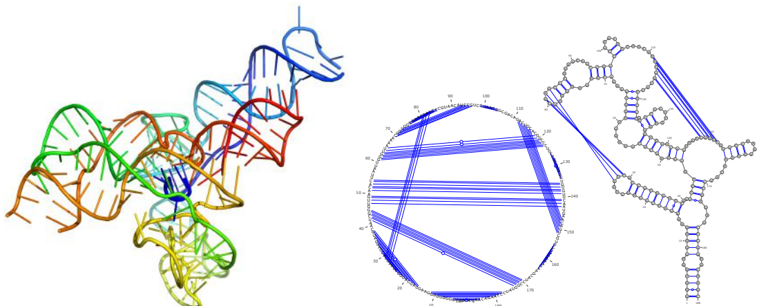
Figure 8.5: Visualization of GIR1 Lariat-capping ribozyme 3D structure with PyMOL [Stockwell, 2003] on the left, and its 2D projection with VARNA [Darty et al., 2009] on the right.
