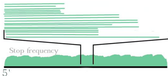
(c) Calculation of the end extremity (the adduct position) frequencies from the aligned cDNAs fragments.
