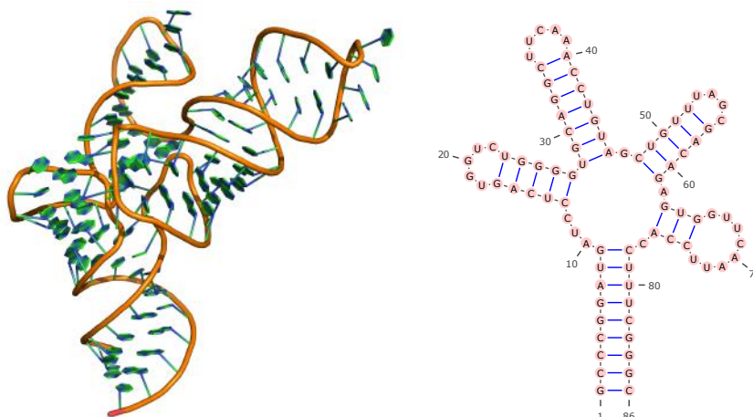
Figure 2.1: 3D model of an atypical selenocysteine-specific tRNA in the Mouse (PDB ID: 3RG5:A, left) and associated secondary structure (right).
