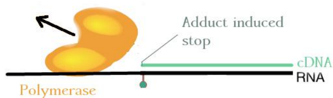
(b) The polymerase proceed with a reverse transcription resulting in a cDNA strand truncated at the level of the adduct.
