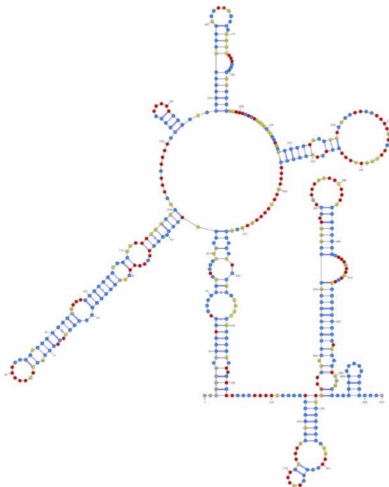
Figure 8.13: Candidate structure(s) for the 3' UTR of the VP40 gene, predicted using IPANEMAP: IPANEMAP identified 20 dominant clusters. One cluster has found to be the optimal with two dominant conditions: 1M7Mg and 1M7. Nucleotides are color-coded based on their normalized SHAPE reactivities ( \leq 0.4 \rightarrow blue, \geq 0.7 \rightarrow red, mid range \rightarrow yellow; missing values in gray)
