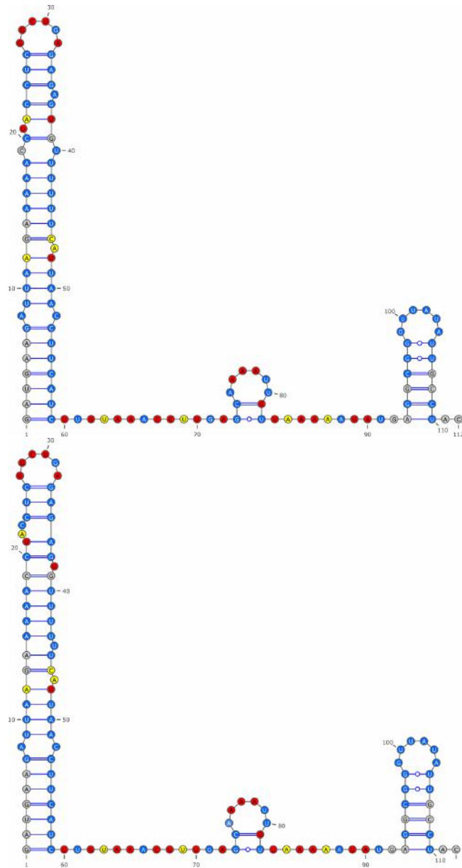
Figure 8.14: Candidate structure(s) for the 5' UTR of the VP40 gene, predicted using IPANEMAP: IPANEMAP identified 3 dominant clusters. Two clusters were found to be optimal: The cluster associated with the top centroid has two representative conditions 1M7Mg and 1M7; The cluster associated with the bottom centroid represents three dominant conditions: MSA,1M7Mg and 1M7. Nucleotides are color-coded based on their normalized SHAPE reactivities ( \leq 0.4 \rightarrow blue, \geq 0.7 \rightarrow red, mid range \rightarrow yellow; missing values in gray)
