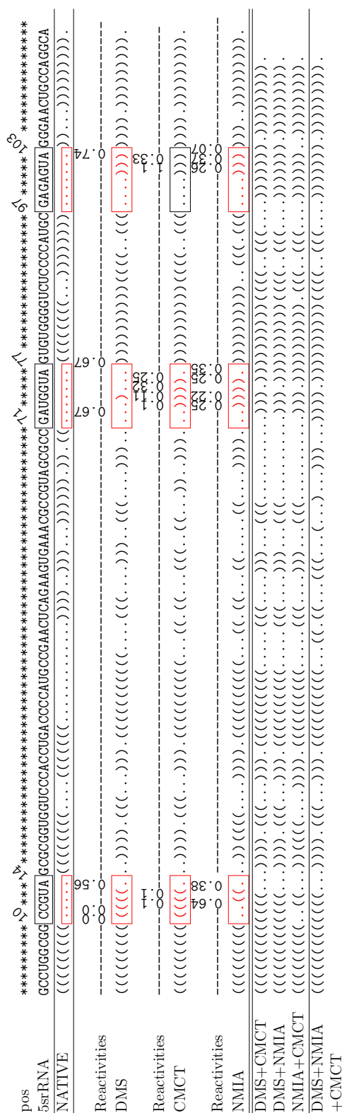
Figure 7.2: 5s rRNA predicted structures using IPANEMAP: we identified 3 single-strand regions in the native structures (in red) where the dominant nucleotides are G and U, and for which NMIA and CMCT conditions are showing a moderate reactivity. The lack of DMS covering and the moderate values reported by the other probing data favored the prediction of stacked nucleotides and subsequently the prediction of an alternative conformation. Although our predictions do not allow to get acceptable MCC as observed with the classic probing guided predictions, the combination of 3 probing data allowed for an accuracy surpassing the minimal value obtained under the mono-probing case.
