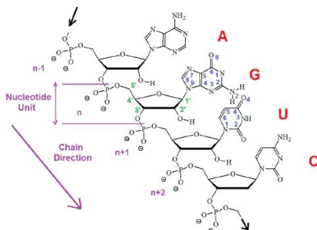
Figure 2.3: The numbering convention of RNA nucleotides: an example of RNA fragment with nucleotides A, G, C and U linked by 3',5'-phosphodiester bonds. The chain direction from 5' to 3' is indicated by an arrow. The atom numbering scheme is indicated in the nucleotide units.
