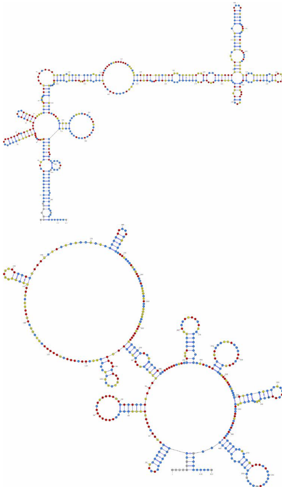
Figure 8.19: Candidate structure(s) for the 3' UTR of the VP24 gene, predicted using IPANEMAP: IPANEMAP identified 20 dominant clusters. Two optimal clusters were identified. The top centroid corresponds to a cluster dominated by MSA and on the right the cluster dominated by 1M7Mg and 1M7 Nucleotides are color-coded based on their normalized SHAPE reactivities ( \leq 0.4 \rightarrow blue, \geq 0.7 \rightarrow red, mid range \rightarrow yellow; missing values in gray)
