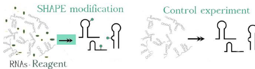
(a) SHAPE protocol with two chemical experiments: the SHAPE experiment in the presence of a reagent and a control experiment to count for the spontaneous stops.
