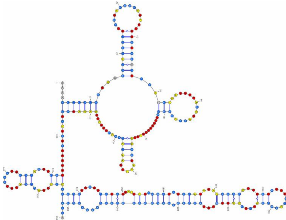
Figure 8.15: Candidate structure(s) for the 3' UTR of the GP gene, predicted using IPANEMAP: IPANEMAP identified 4 dominant clusters. One cluster was found to be optimal with 2 dominant conditions: 1M7Mg and 1M7. Nucleotides are color-coded based on their normalized SHAPE reactivities ( \leq 0.4 \rightarrow blue, \geq 0.7 \rightarrow red, mid range \rightarrow yellow; missing values in gray)
