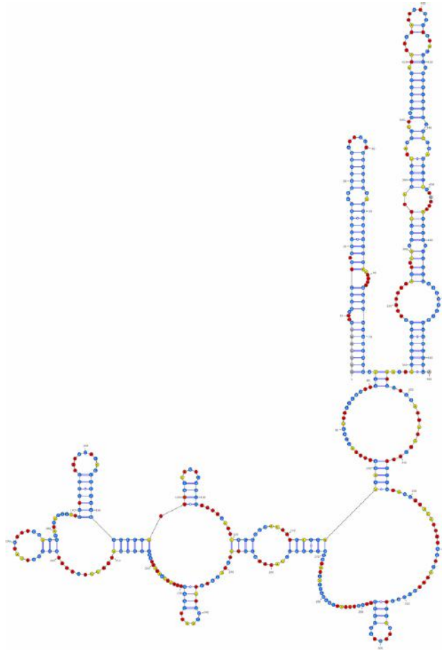
Figure 8.20: Candidate structure(s) for the 5' UTR of the VP24 gene, predicted using IPANEMAP: IPANEMAP identified 3 dominant clusters. One cluster has found to be the optimal with two dominant conditions: 1M7Mg and 1M7. Nucleotides are color-coded based on their normalized SHAPE reactivities ( \leq 0.4 \rightarrow blue, \geq 0.7 \rightarrow red, mid range \rightarrow yellow; missing values in gray)
