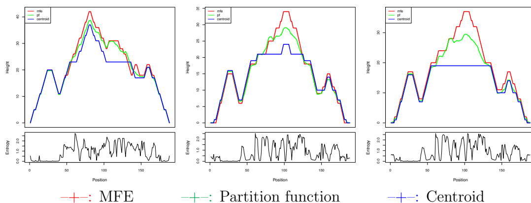
Figure 8.6: Shannon entropy from predictions with RNAfold in the absence of probing data (on the left), with 1M7ILU3 data for a pseudo-energy of \delta G (on the middle) and \frac{\delta G}{2} (on the right). The consideration of probing data allowed for less fluctuations of the local structure. Changing the pseudo-free energy contribution by half does not affect the MFE structure. However, a slight difference has been detected at both extremities of the sequence. Figures were generated with RNAfold.
