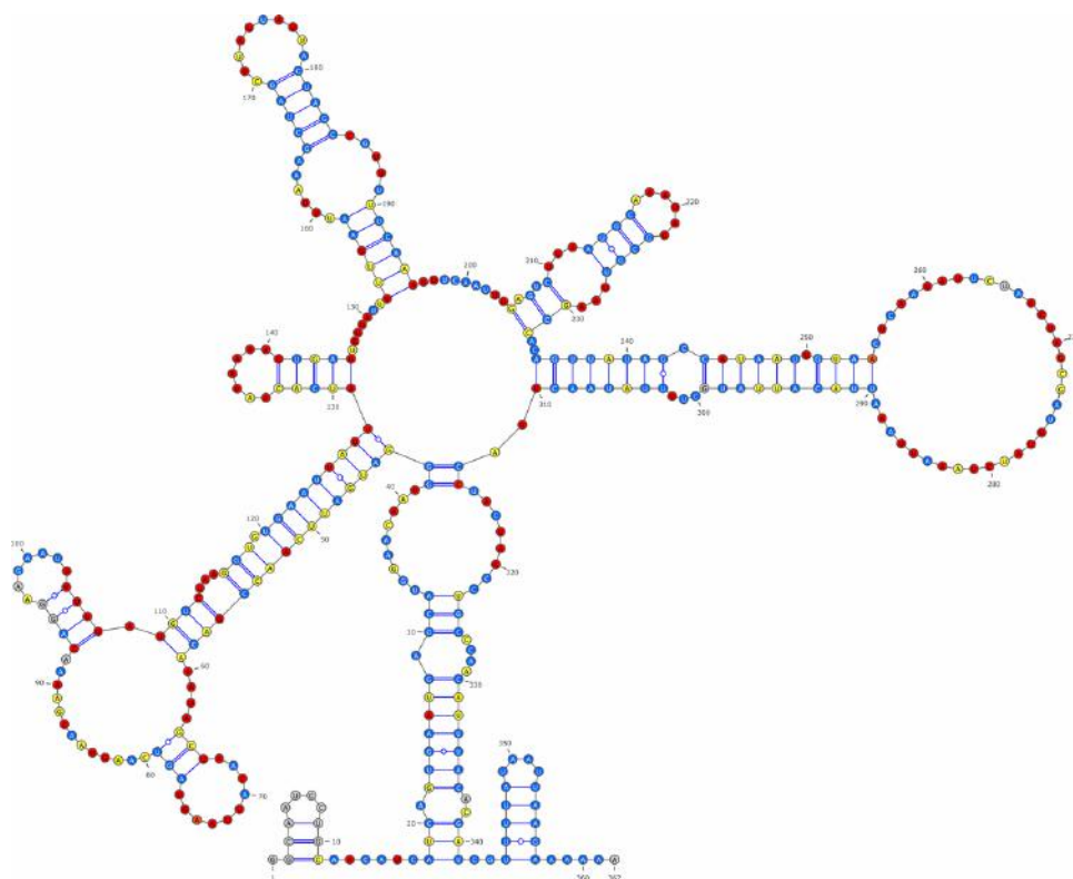
Figure 8.9: Candidate structure(s) for the 3' UTR of the NP gene, predicted using IPANEMAP: IPANEMAP identified 4 dominant clusters. One cluster was found to be the optimal with two dominant conditions: 1M7Mg and MSA. Nucleotides are color-coded based on their normalized SHAPE reactivities ( \leq 0.4 \rightarrow blue, \geq 0.7 \rightarrow red, mid range \rightarrow yellow; missing values in gray)
