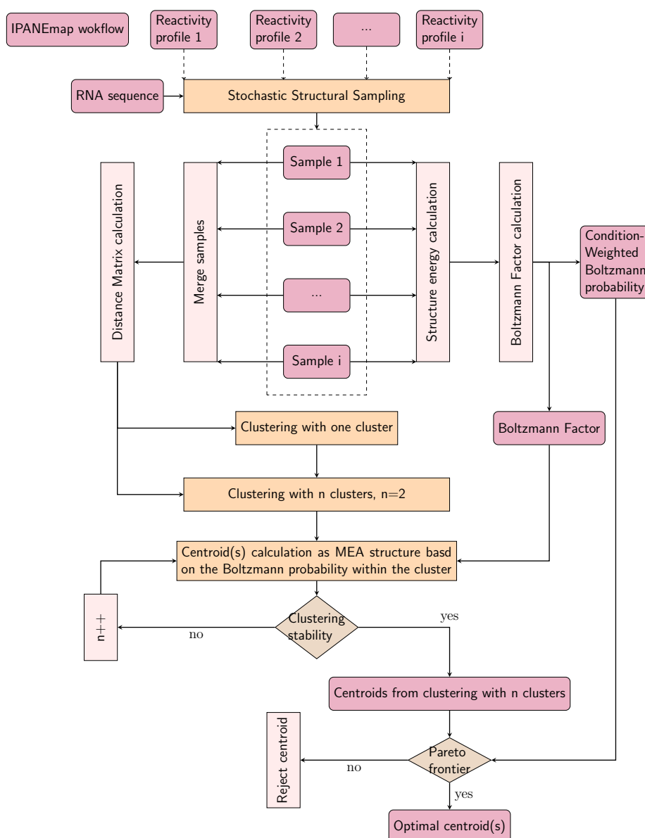
Figure 5.1: Schematic diagram of IPANEMAP. For a given RNA sequence and i relative structural profiling data (Reactivity profile 1, Reactivity profile 2...) as input data, IPANEMAP proceeds with a stochastic sampling for each of the predicted data-driven ensemble apart. Leading to a set of i samples (sample 1, sample 2...) representing the i experimental conditions. Then, the Boltzmann probability is calculated for each structure from each sample apart. We refer to this probability as the Conditional Weighted Boltzmann probability. In Parallel, samples are mixed in one set while retaining the label for the condition of origin of each of the structures. Then, the distance separating different structures from the set are assessed to allow IPANEMAP to proceed for the iterative clustering process that involves a clusters stability checking step and returns the number of clusters with their corresponding structure contents where each cluster is characterized by its centroid structure MEA. Centroids from clusters with their respective cumulated Weighted Boltzmann probability are used for the optimality check (Pareto frontier). Resulting optimal centroid(s) form the predicted structures through our integrative approach.
