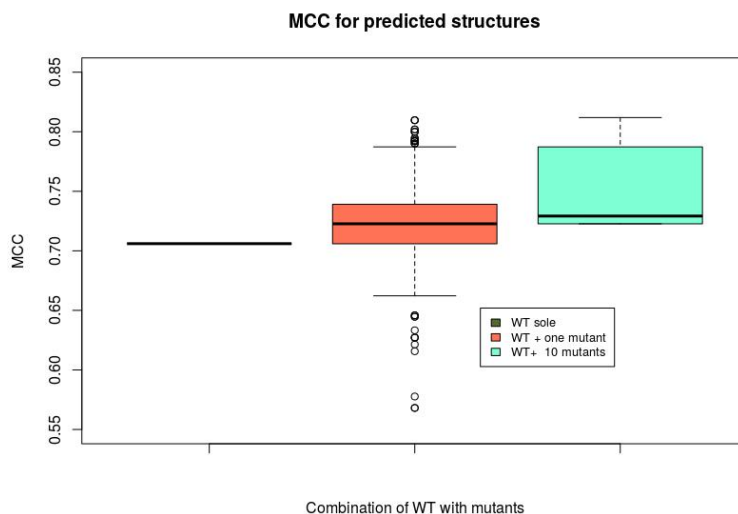
Figure 9.2: MCC distribution from Differential-DMS with different combinations: for mono-probing with the WT, bi-probing from one mutant with the WT and multiprobing from the combination of 10 mutants with the WT. The first quartile from the bi-probing distribution exceeds the value when the WT is used alone. Compared to the bi-probing, the multi-probing with the mutants combination allowed to get an MCC value that surpasses the median value from the bi-probing distribution.
