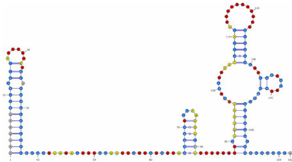
Figure 8.16: Candidate structure(s) for the 5' UTR of the GP gene, predicted using IPANEMAP: IPANEMAP identified 3 dominant clusters. One optimal cluster was found with 2 dominant conditions 1M7Mg and 1M7. Nucleotides are color-coded based on their normalized SHAPE reactivities ( \leq 0.4 \rightarrow blue, \geq 0.7 \rightarrow red, mid range \rightarrow yellow; missing values in gray)
