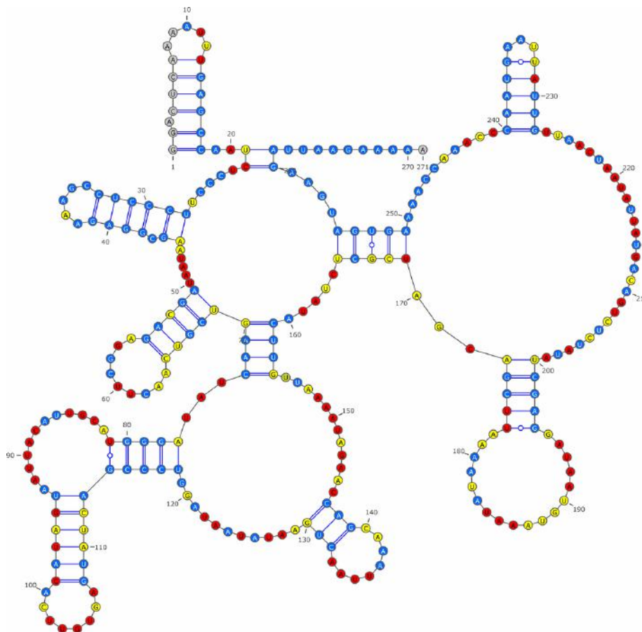
Figure 8.11: Candidate structure(s) for the 3' UTR of the VP35 gene, predicted using IPANEMAP: IPANEMAP identified 3 dominant clusters. One cluster has found to be optimal with 2 dominant conditions: 1M7Mg and 1M7. Nucleotides are color-coded based on their normalized SHAPE reactivities ( \leq 0.4 \rightarrow blue, \geq 0.7 \rightarrow red, mid range \rightarrow yellow; missing values in gray)
