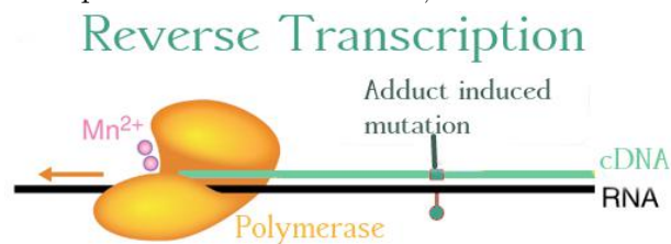
(b) The polymerase proceed in a reverse transcription, the adduct induces a mutation.
