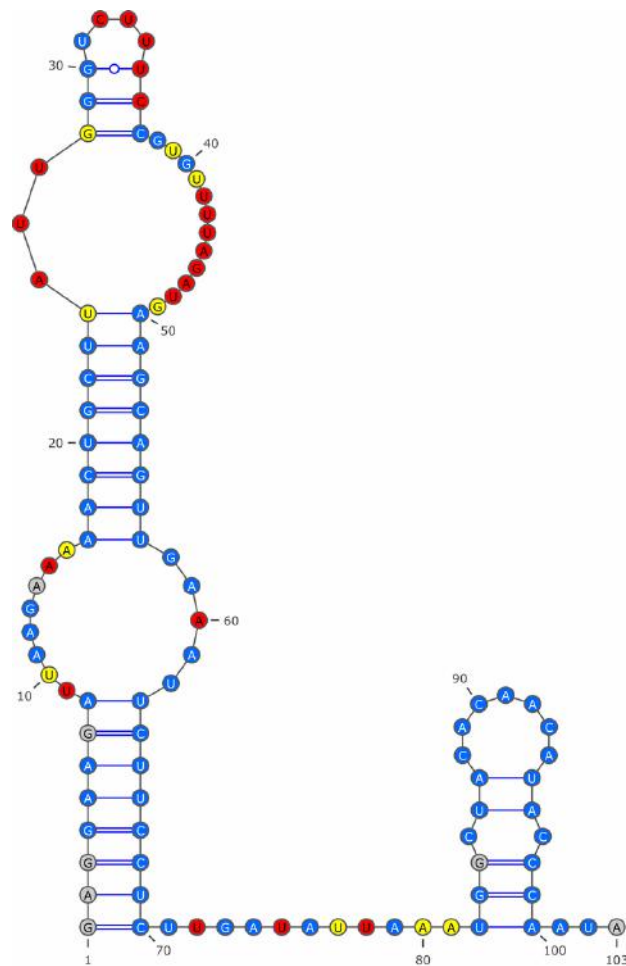
Figure 8.22: Candidate structure(s) for the 5' UTR of the L gene, predicted using IPANEMAP: IPANEMAP identified 2 dominant clusters. One cluster has found to be optimal with all conditions MSA, 1M7Mg and 1M7 as dominant. Nucleotides are color-coded based on their normalized SHAPE reactivities ( \leq 0.4 \rightarrow blue, \geq 0.7 \rightarrow red, mid range \rightarrow yellow; missing values in gray)
