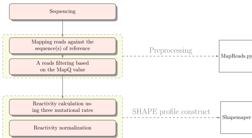
Figure 4.2: SHAPeMap reactivities from HTS output.
