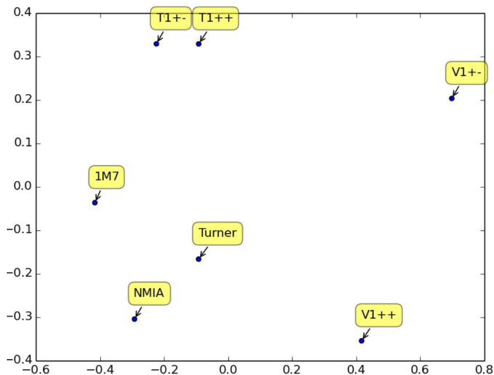
Figure 8.2: Multi-Dimensional Scaling (MDS) to display the euclidean distance between predicted ensembles where the horizontal axes present high-dimensional objects in typically two dimensions. In addition to the six conditions, the case without constraints pointed by Turner is considered. We observed the formation of a cluster, involving conditions from [NMIA, 1M7, V1++, T1++, T1+-], around the Turner model where the condition [V1+-] is distant from the cluster.
