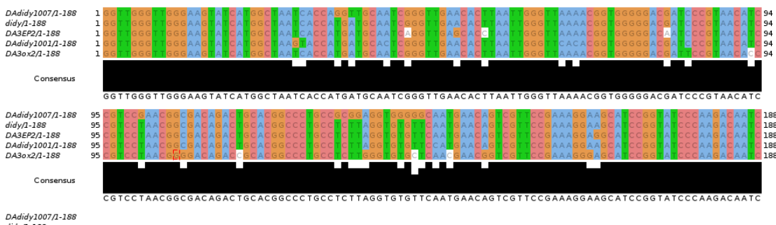
Figure 6.2: Alignment of 5 GIR1 Lariat-capping ribozyme mutants sequences used to build the test dataset. The figure was obtained using Jalview software.
