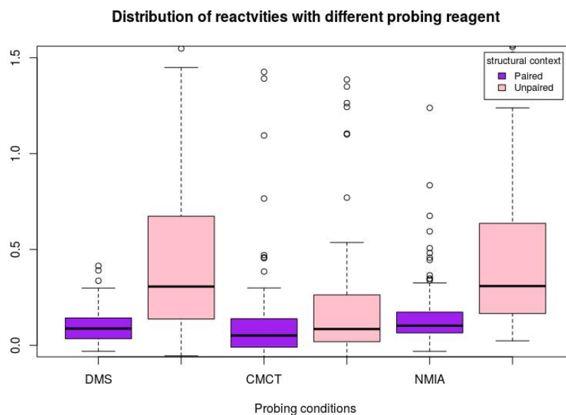
Figure 9.1: Distribution of reactivities for different probing data: DMS, CMCT and NMIA, in function of the structural context (paired/unpaired). A significant overlap between the two structural contexts is observed for the case of CMCT data.
