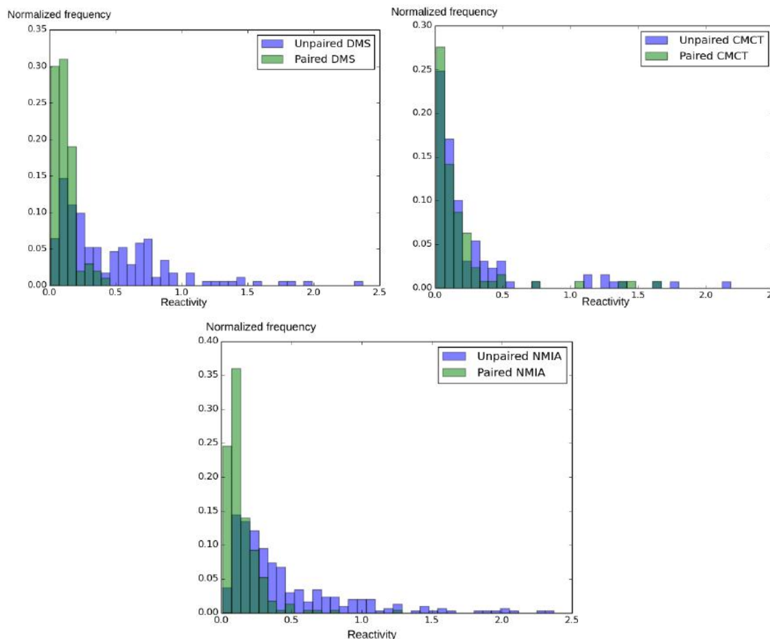
Figure 3.1: Distribution of reactivities for paired vs. unpaired nucleotides. Three probing reagent are considered: DMS, CMCT and NMIA. Data was extracted from [Cordero et al., 2012]. SHAPE NMIA probing data better reflects the correlation with the local structure but less well than the DMS data, whereas CMCT data do not differentiate between paired and unpaired nucleotides.
