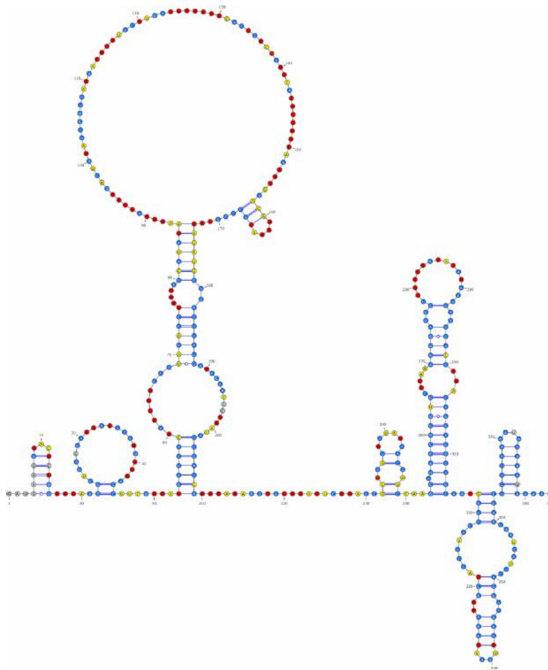
Figure 8.17: Candidate structure(s) for the 3' UTR of the VP30 gene, predicted using IPANEMAP: IPANEMAP identified 4 dominant clusters. One cluster was found to be optimal with one dominant condition: 1M7Mg. Nucleotides are color-coded based on their normalized SHAPE reactivities ( \leq 0.4 \rightarrow blue, \geq 0.7 \rightarrow red, mid range \rightarrow yellow; missing values in gray)
