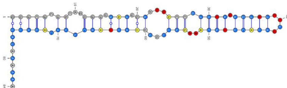
Figure 8.21: Candidate structure(s) for the 3' UTR of the L gene, predicted using IPANEMAP: IPANEMAP identified 2 dominant clusters. One cluster has found to be optimal with all conditions MSA, 1M7Mg and 1M7 as dominant. Nucleotides are color-coded based on their normalized SHAPE reactivities ( \leq 0.4 \rightarrow blue, \geq 0.7 \rightarrow red, mid range \rightarrow yellow; missing values in gray)
