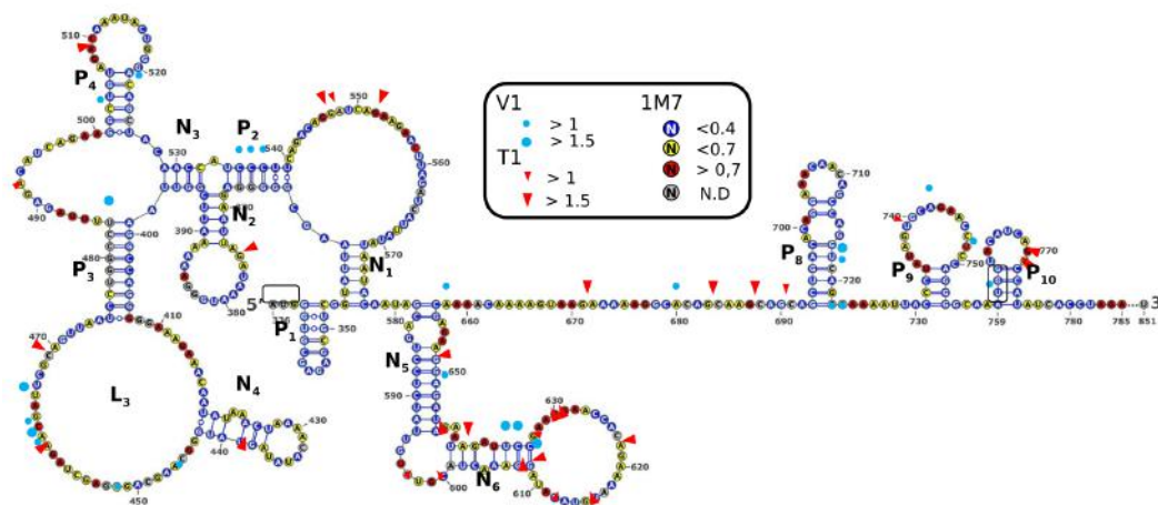
Figure 8.3: HIV1 gag IRES predicted structure using IPANEMAP in the presence of SHAPE and enzymatic probing data as presented in the article [Deforges et al., 2017].
