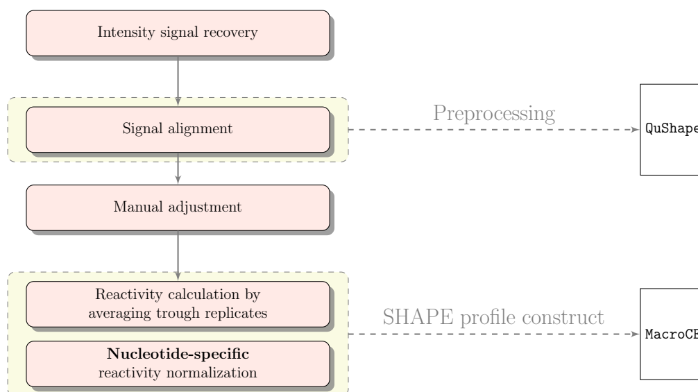
Figure 4.1: Pipeline for computing SHAPE reactivities using capillary electrophoresis technique.
