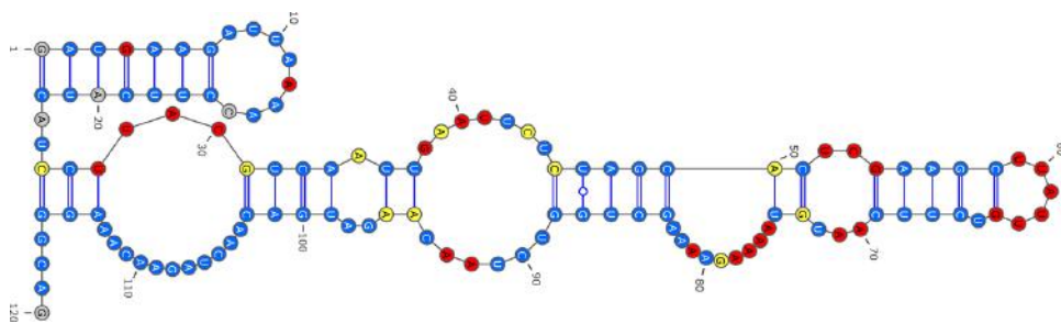
Figure 8.12: Candidate structure(s) for the 5' UTR of the VP35 gene, predicted using IPANEMAP: IPANEMAP identified 3 dominant clusters. One optimal cluster with all conditions: 1M7Mg, 1M7 and MSA as representative. Nucleotides are color-coded based on their normalized SHAPE reactivities ( \leq 0.4 \rightarrow blue, \geq 0.7 \rightarrow red, mid range \rightarrow yellow; missing values in gray)
