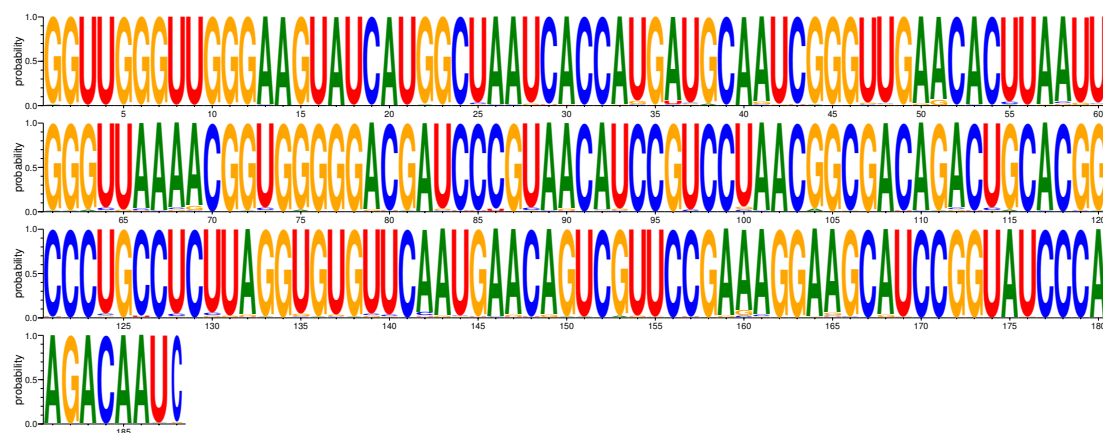
Figure 6.1: Mutation distribution after a non-directed mutagenesis PCR of 30 steps over 92 chosen mutants.
