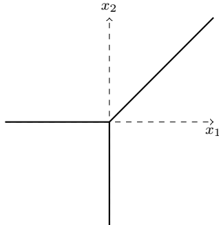
Figure 3.1: Tropical hypersurface associated to the tropical polynomial \max(x_1, x_2, 0) . It corresponds to the union of three rays: \{x \in \mathbb{R}^2 \mid x_1 = x_2 \geq 0\} , \{x \in \mathbb{R}^2 \mid x_1 = 0 \geq x_2\} and \{x \in \mathbb{R}^2 \mid x_2 = 0 \geq x_1\} .
