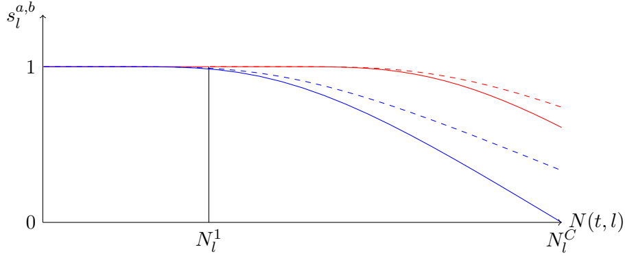
Figure 7.1: Different kind of satisfaction functions of the number of active customers in a cell. The blue ones are those for streaming contents whereas the red ones are those for web, mail and download contents. The dashed ones corresponds to the satisfaction of standard customers, the continuous ones to the satisfaction of premium customers.
