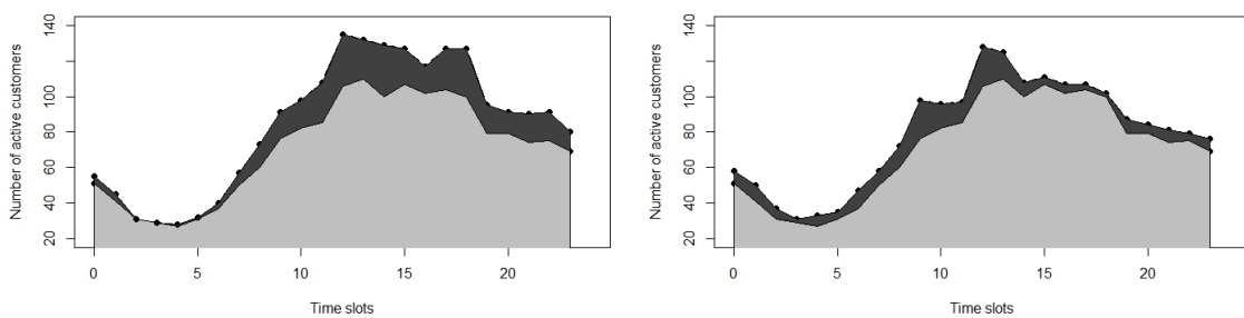
Figure 7.10: Traffic in the most loaded cell. The light grey part represents the web, mail and streaming customers who have no incentives and are fixed. The dark grey part corresponds to the download customers in the cell without (left) and with (right) incentives
