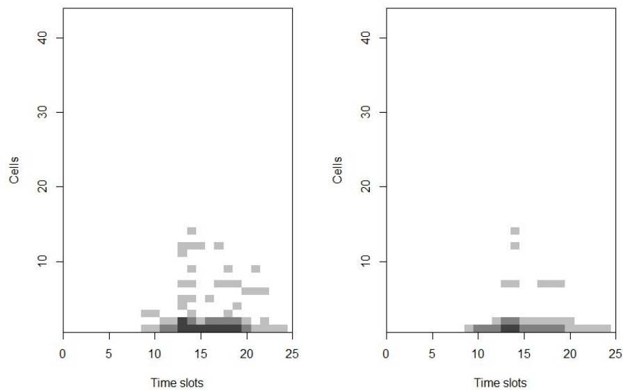
Figure 7.8: Satisfaction of premium customers for web, mail or download without (left) and with (right) incentives
