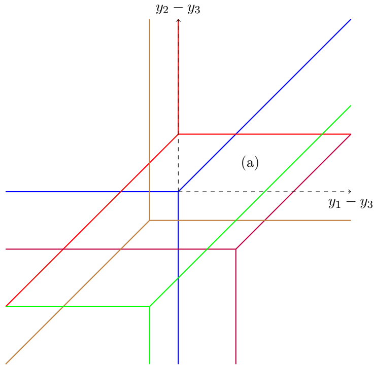
Figure 7.3: Arrangement of tropical hypersurfaces: each tropical hypersurface corresponds to a customer response. For example, the cell (a) corresponds to discounts y with responses (1,0,0) for customer 1, (1,0,1) for customer 2, (0,1,0) for customer 3, (1,1,0) for customer 4 and (0,1,0) for customer 5. Hence, the total number of customers in the network with these discounts is (3,3,1).
