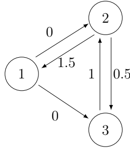
Figure 7.4: Graph G associated to the vector N = (3, 3, 1)
