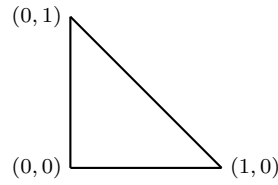
Figure 3.2: Newton polytope associated to the tropical polynomial \max(x_1, x_2, 0) . The vertices of this polytope are in one-to-one correspondence with the maximal cells of the subdivision defined by the tropical line.
