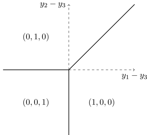
Figure 7.2: A customer response: a tropical line splits the projective space into three cells. Each cell corresponds to a possible customer response
