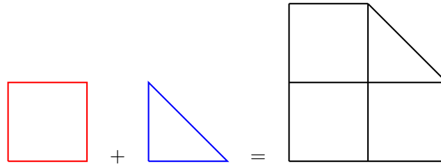
Figure 6.2: The subdivisions of the Newton polytope associated to Q_1 (blue one), Q_2 (red one) and Q (black one). The polytope \text{New}(Q) is equal to \text{New}(Q_1) + \text{New}(Q_2)
