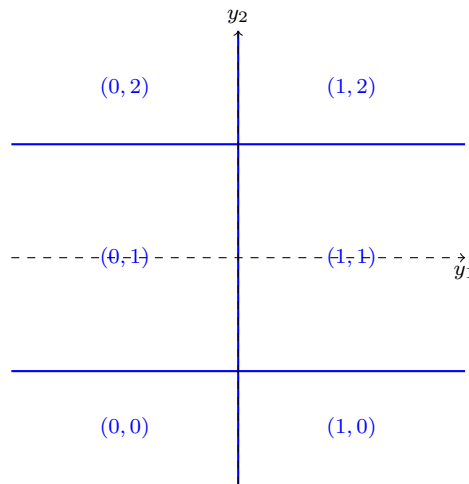
Figure 4.1: Tropical hypersurface \mathcal{T}(Q) associated to the polynomial Q . It subdivides \mathbb{R}^2 in different cells. The degree of the monomial which attains the maximum in Q is mentioned in each full-dimensional cell.
