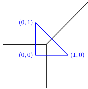
Figure 3.3: One-to-one correspondence between the tropical hypersurface associated to the polynomial \max(x_1, x_2, 0) (in black) and the Newton polytope of this polynomial (in blue). The vertices of this polytope are in one-to-one correspondence with the maximal cells of the subdivision defined by the tropical line.
