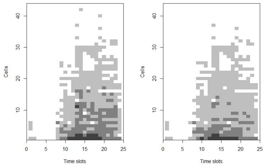
Figure 7.7: Satisfaction of standard customers for streaming without (left) and with (right) incentives
