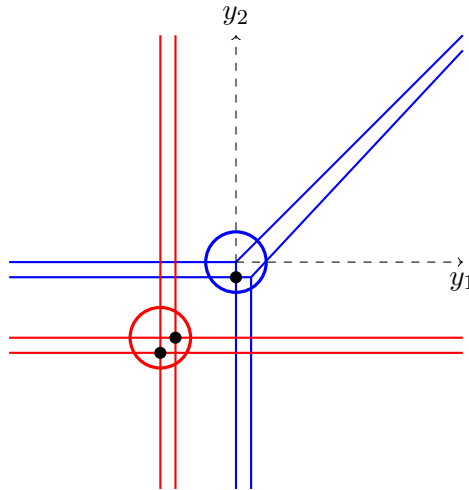
Figure B.1: Arrangement of perturbed tropical hypersurfaces: the blue ones are \mathcal{T}(P_1) together with its perturbation, the red ones are \mathcal{T}(P_2) together with its perturbation. The blue circle is centered in the apex of \mathcal{T}(P_1) , the red one is centered in the apex of \mathcal{T}(P_2) . We see that there exists at least one intersection point of the two "copies" of each tropical hypersurface in every circle.
