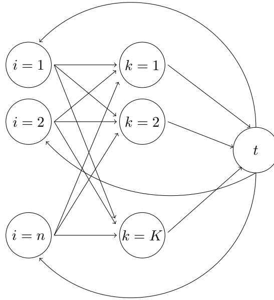
Figure 7.5: Minimum cost flow problem transformed in a minimum cost circulation problem. The flow in the edges between each i and k is in [0, 1] , the flow in the edges between each k and t is equal to R_k , and the flow in the edges between t and each i is N_i^* .
