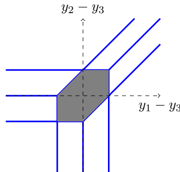
Figure C.2: Representation of the arrangement of the tropical polynomials defined by \bigotimes Q_k in \mathbb{TP}^2 . The cell \mathcal{H}^P is filled in gray.
