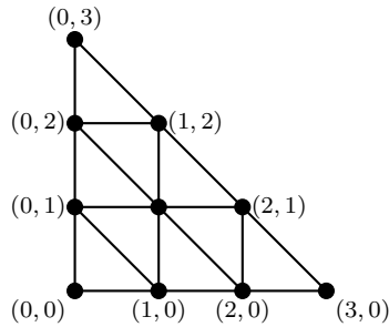
Figure 5.1: An edgewise subdivision of \Delta_3 in dimension 2
