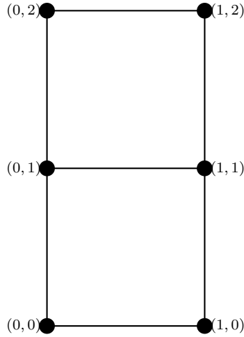
Figure 4.2: Dual subdivision \mathcal{S}' of the Newton polytope \text{New}(Q) = [0, 1] \times [0, 2] .
