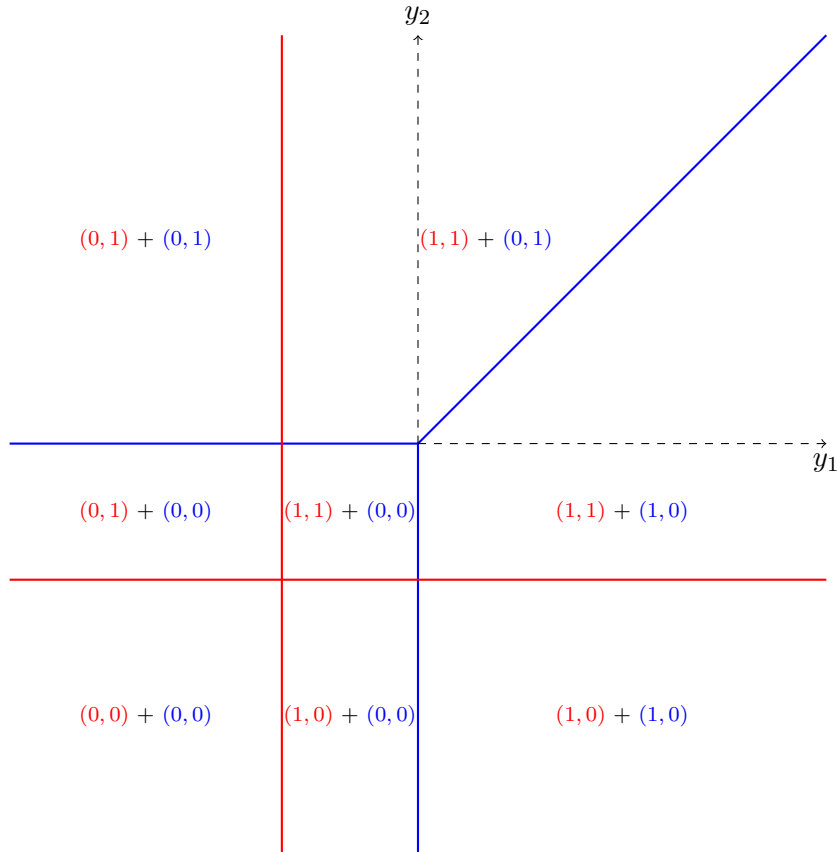
Figure 6.1: Arrangement of tropical hypersurfaces: the blue one is \mathcal{T}(Q_1) and the red one is \mathcal{T}(Q_2) . The arrangement corresponds to the tropical hypersurface associated to Q = Q_1 \odot Q_2 . In each cell, we can determine the global low-level response with its decomposition into each customers.
