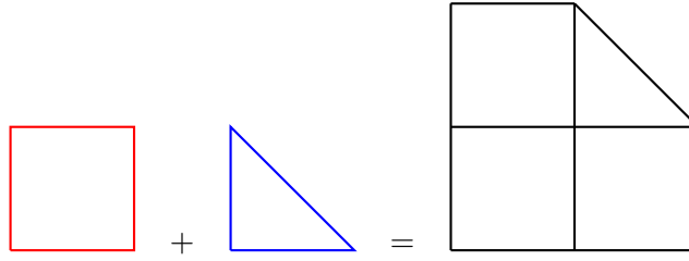
Figure 6.2: The subdivisions of the Newton polytope associated to Q_1 (blue one), Q_2 (red one) and Q (black one). The polytope \text{New}(Q) is equal to \text{New}(Q_1) + \text{New}(Q_2)
