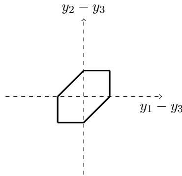
Figure C.1: Representation of \mathcal{H}^P in \mathbb{TP}^2
