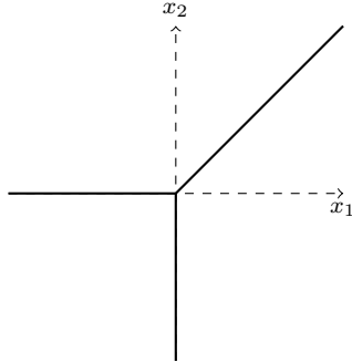
Figure 3.1: Tropical hypersurface associated to the tropical polynomial \max(x_1, x_2, 0) . It corresponds to the union of three rays: \{x \in \mathbb{R}^2 \mid x_1 = x_2 \geq 0\} , \{x \in \mathbb{R}^2 \mid x_1 = 0 \geq x_2\} and \{x \in \mathbb{R}^2 \mid x_2 = 0 \geq x_1\} .
