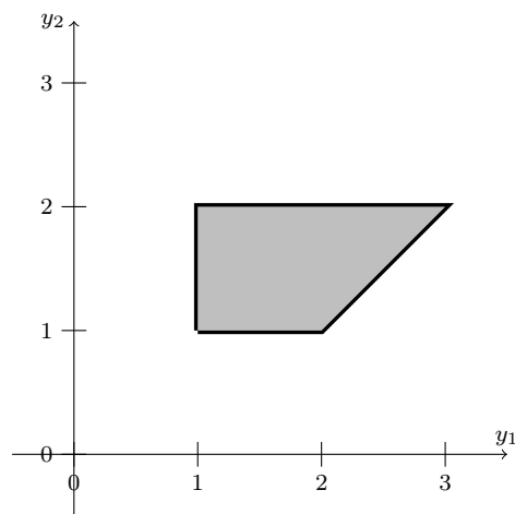
Figure 6.3: Set of optimal prices \mathcal{Y}_\lambda of Problem (\mathcal{P}_\lambda) for \lambda = 0.1
