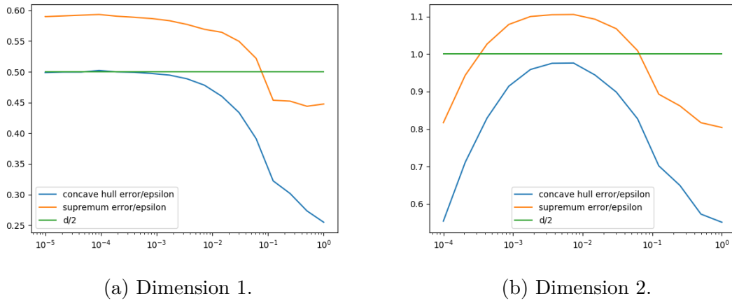
Fig. 5.1 Duality gap for the supremum, and the concave hull dual approximation vs \varepsilon .
