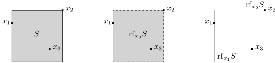
Fig. 2.2 Examples of relative faces.
