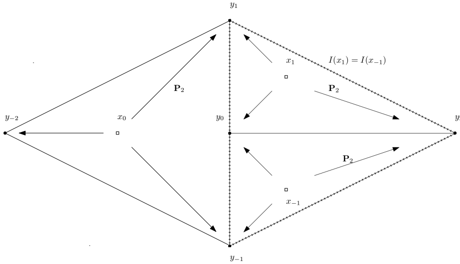
Fig. 3.3 Disintegration on an irreducible component is not irreducible.
