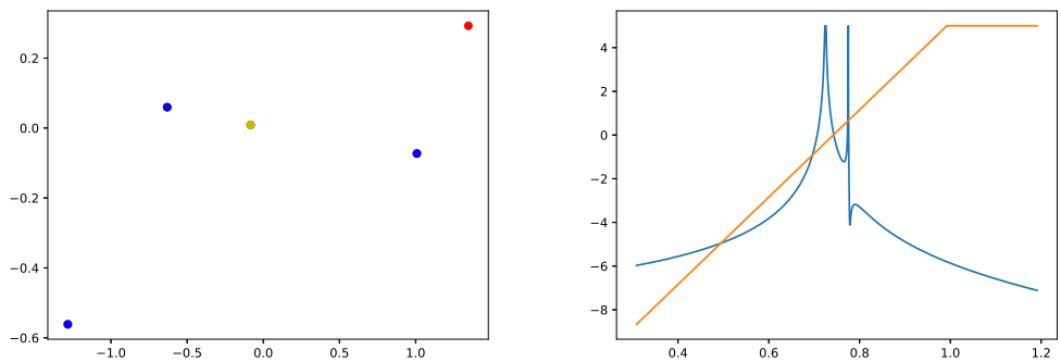
Fig. 4.3 S_0 for d = 2 and p = 2.1 .
