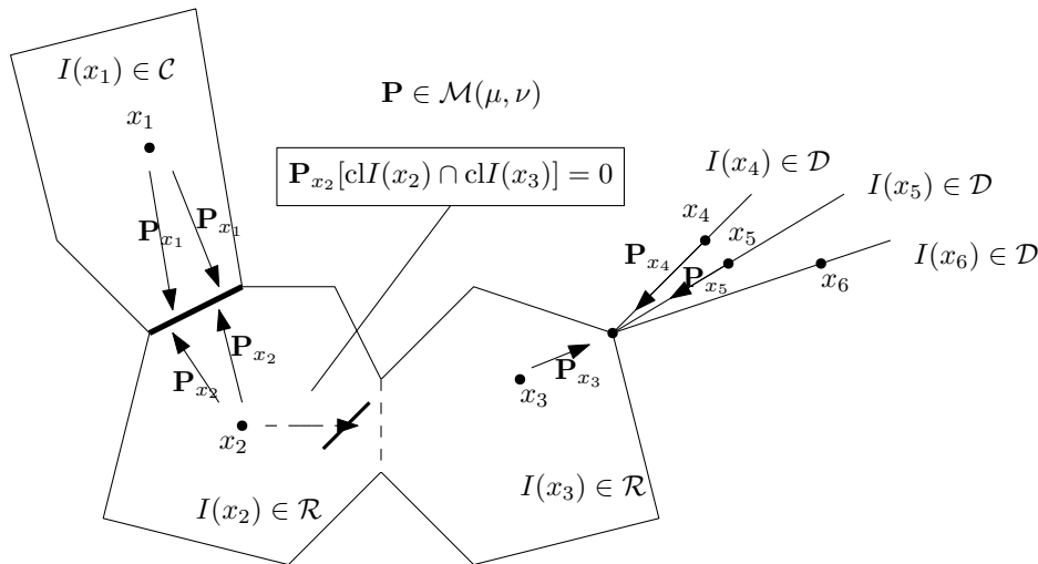
Fig. 3.1 No communication between frontiers of elements in \mathcal{R} .
