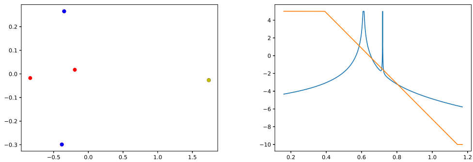
Fig. 4.2 S_0 for d = 2 and p = 1.9 .
