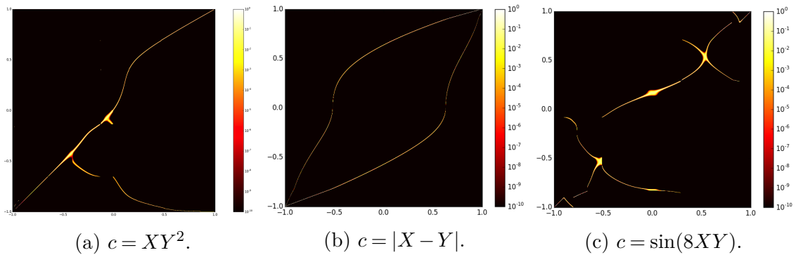
Fig. 5.3 Optimal coupling for different costs in dimension one.
