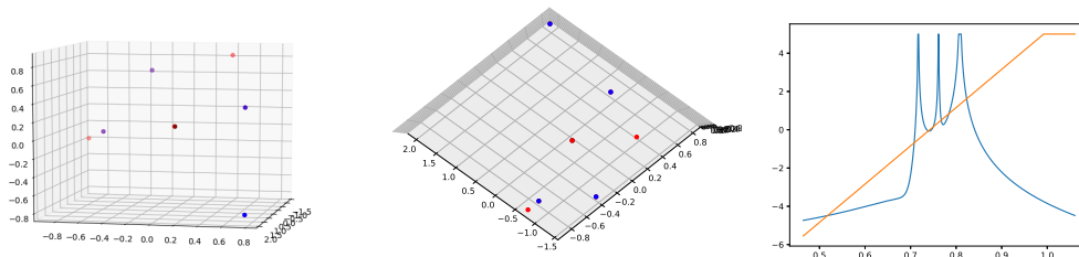
Fig. 4.5 S_0 for d = 3 and p = 2.1 .
