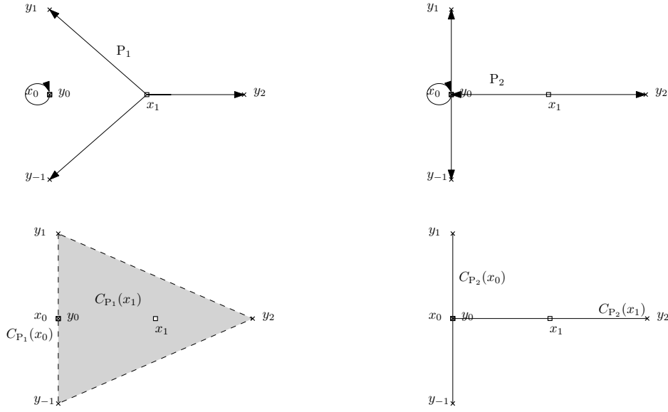
Fig. 2.1 The extreme probabilities and associated irreducible paving.
