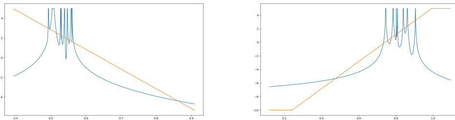
Fig. 4.6 S_0 for d = 8 , p = 1.9 on the left and p = 2.1 on the right.
