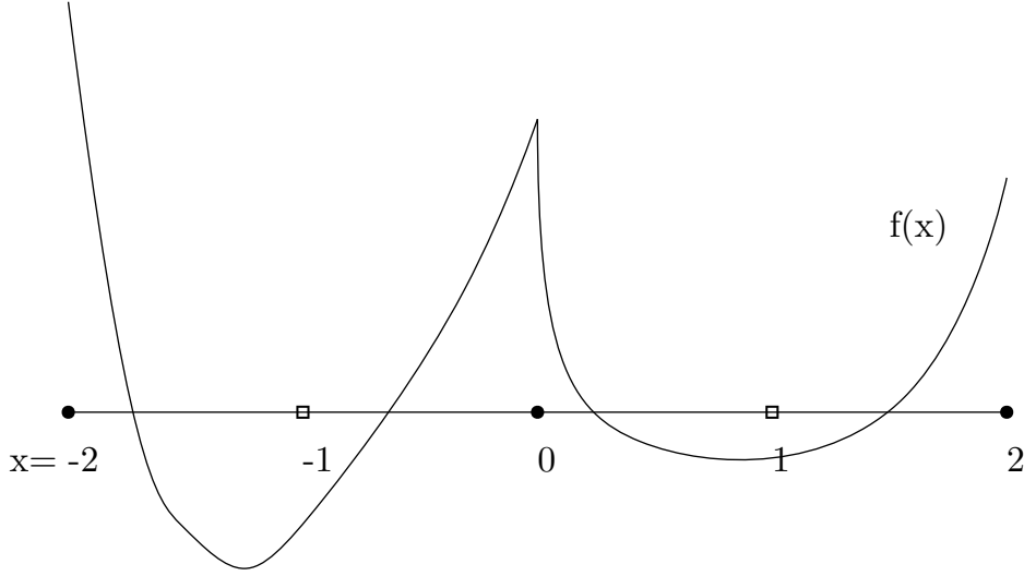
Fig. 3.2 Example of a \mathcal{M}(\mu, \nu) -convex function.
