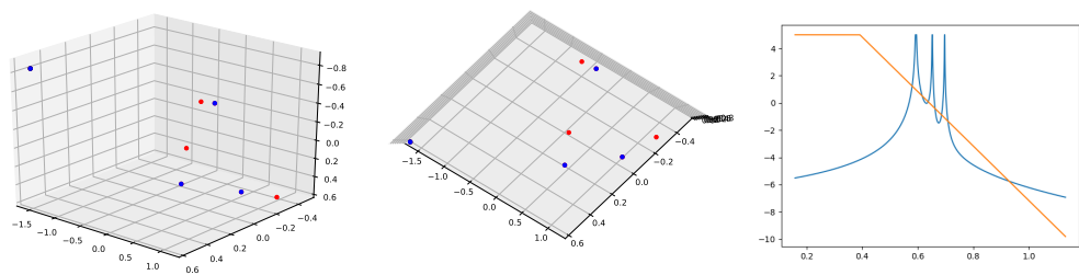
Fig. 4.4 S_0 for d = 3 and p = 1.9 .
