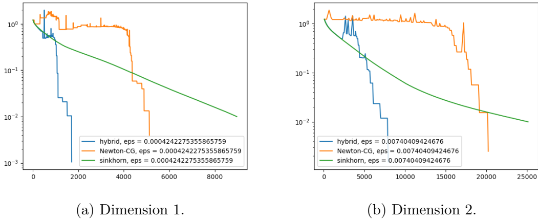
Fig. 5.2 Log plot of the size of the gradient VS time for the Bregman projection algorithm, the Newton algorithm, and the Hybrid algorithm.
