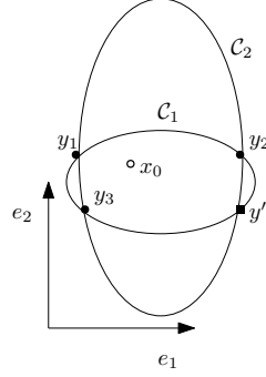
Fig. 4.1 Solution of c_x(x_0, Y) = A(Y) for c(x, y) = x_1(y_1^2 + 2y_2^2) + x_2(2y_1^2 + y_2^2) .
