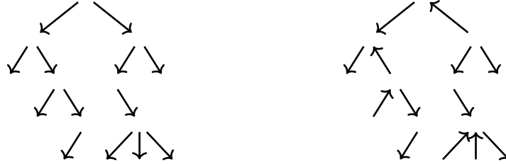
Figure 2 – Examples of unlabeled downward tree (left) and polytree (right)
