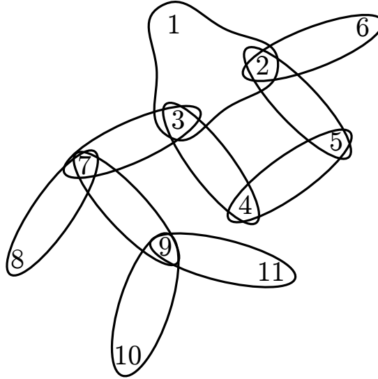
Figure 1.1 – Hypergraph associated to the relational instance from Example 1.1.1.
