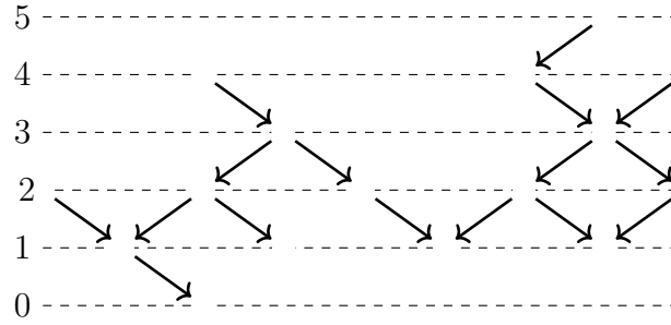
Figure 2.6 – A DAG with a level mapping (dashed lines), see Definition 2.3.5.
