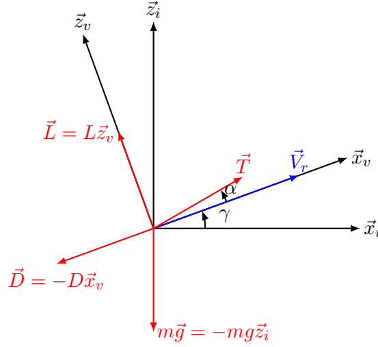
Figure 3.1 – \mathcal{R}_v rotation relative to \mathcal{R}_i in the case of a trajectory in a vertical plane with flat Earth assumption (all the vectors depicted are contained in the same plane).
