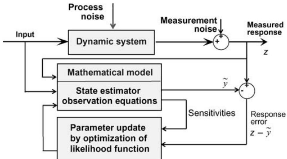
Figure 3.9 – Block schematic of Filter-Error method (figure from [Jategaonkar, 2006, p.133]).
