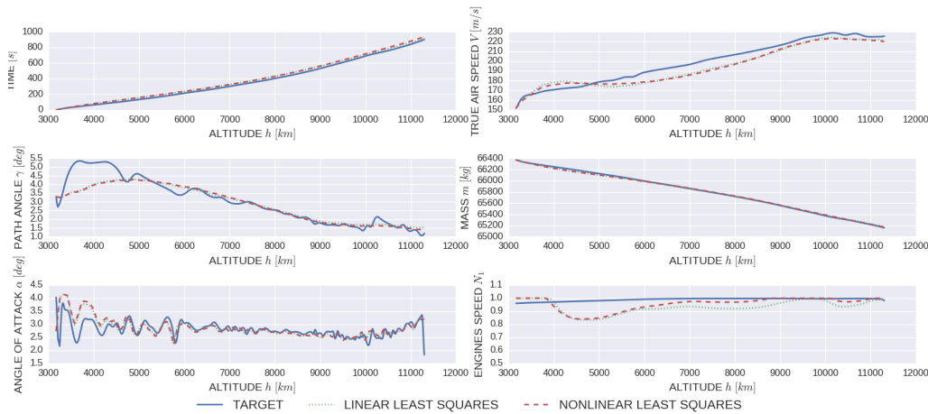
Figure 3.15 – Solution of problem (3.7.5) using dynamics estimated by single-task OLS (dotted green) and multi-task NLS (dashed red), in comparison to a recorded flight (full blue line).
