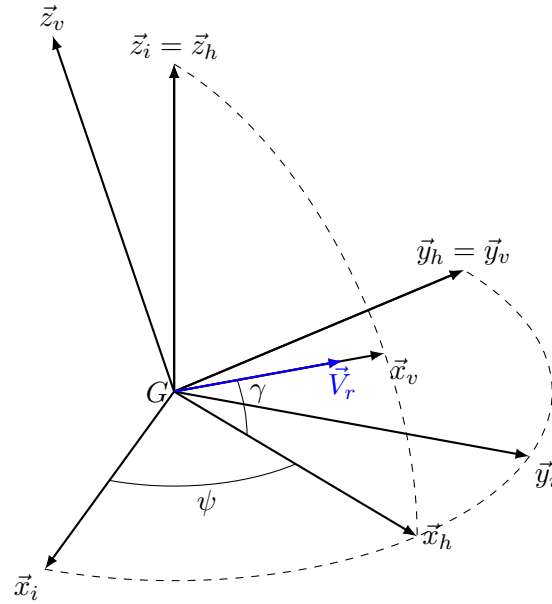
Figure 3.3 – \mathcal{R}_v rotation relative to \mathcal{R}_i in the case of a 3D trajectory with flat Earth assumption.
