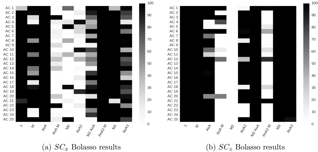
Figure 4.5 – Single-task aerodynamic features selection results using no-wind-dynamics.
