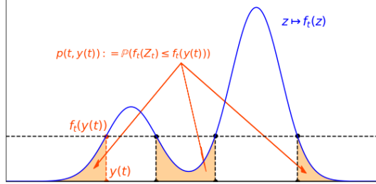
Figure 5.2 – Illustration of the confidence level in the case of a univariate bimodal distribution
