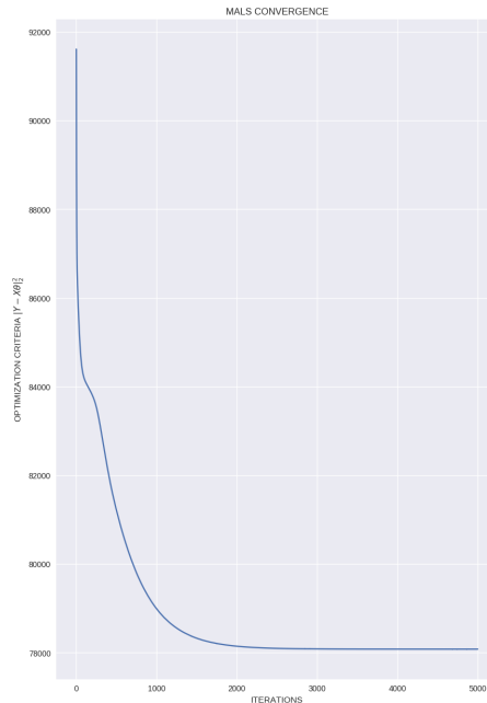
Figure 4.10 – Evolution of the multi-task least-squares criterion over ALS iterations.
