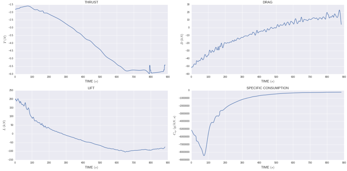
Figure 4.9 – Predicted forces using nonlinear least-squares. These results corresponds to the same experiment as figure 3.14 from section 3.8.
