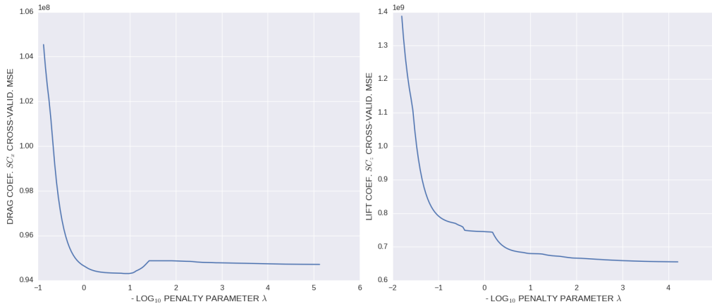
Figure 4.4 – Single-task Bolasso penalty parameter selection via cross-validation (no-wind-dynamics)
