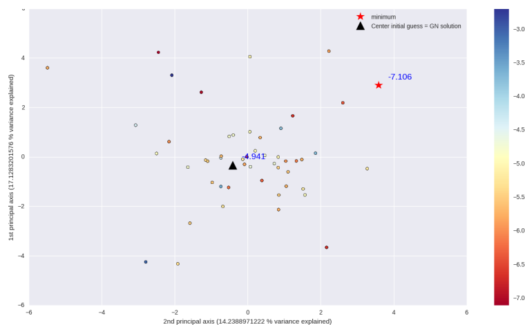
Figure 3.11 – Projection on two most informative principal components of the local solutions of problem (3.6.30). The black triangle represents the solution obtained by initializing at \hat{\theta}_{NLLS} , the solution of nonlinear least-squares, while the red star is the best local minimum w.r.t. the negative log-likelihood. The color encodes the criterion value.
