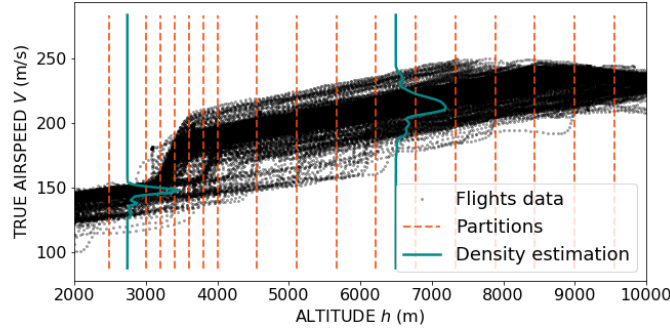
Figure 5.3 – Illustration of the marginal density estimation.
