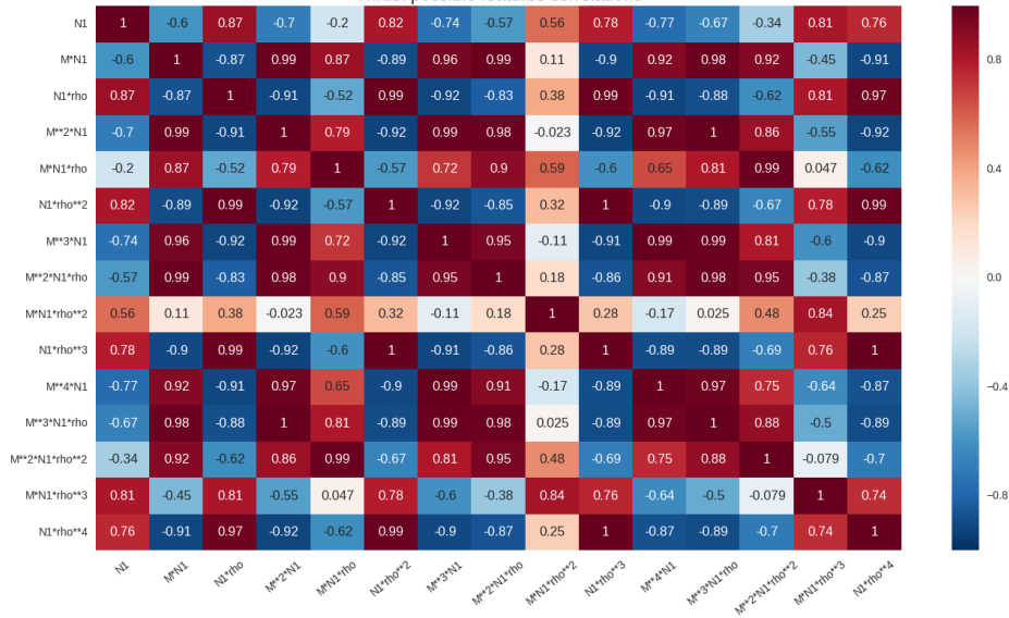
Figure 4.8 – Monomials correlation matrix of the Thrust model.
