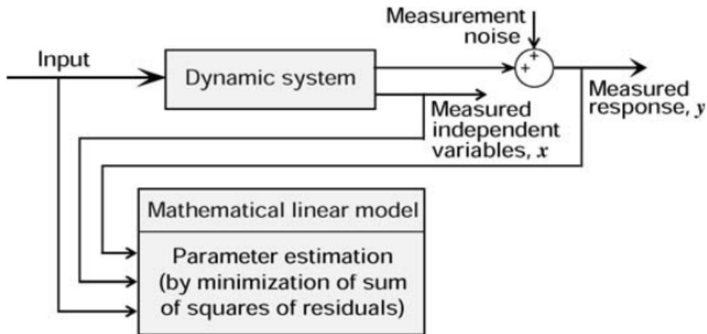
Figure 3.10 – Block schematic of Equation-Error method (from [Jategaonkar, 2006, p.179]).
