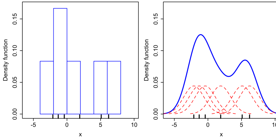
Figure 5.4 – Illustration of a histogram density estimation ( left ) and a kernel density estimation ( right ) built using the same samples. The red dashed curves correspond to the kernels centered at the data points. 3
