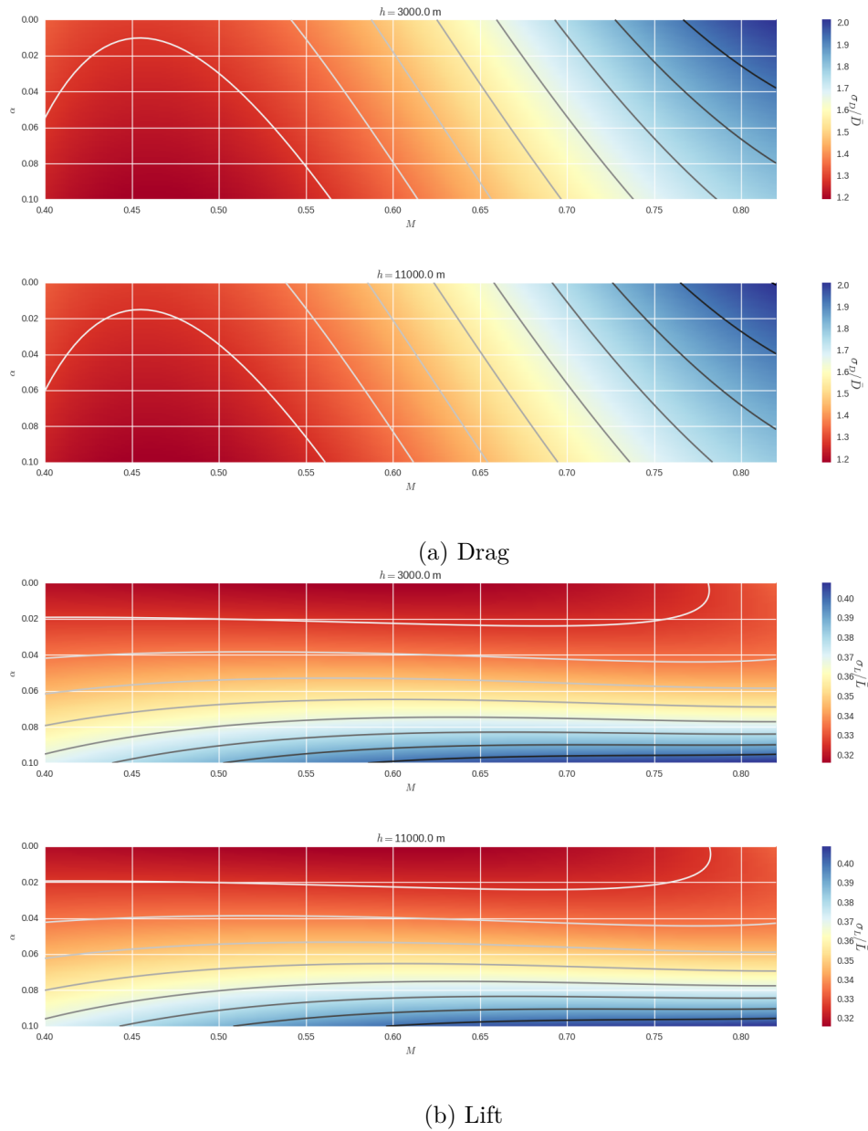
Figure 3.12 – Standardized dispersion (ratio of the standard deviation to the mean \sigma/\mu ) induced on the predicted drag \hat{D} and lift \hat{L} by the 50 local solutions found. As D and L depend on h, \alpha, M , each panel corresponds to a fixed altitude h and depicts the dispersion over a realistic range of (\alpha, M) .
