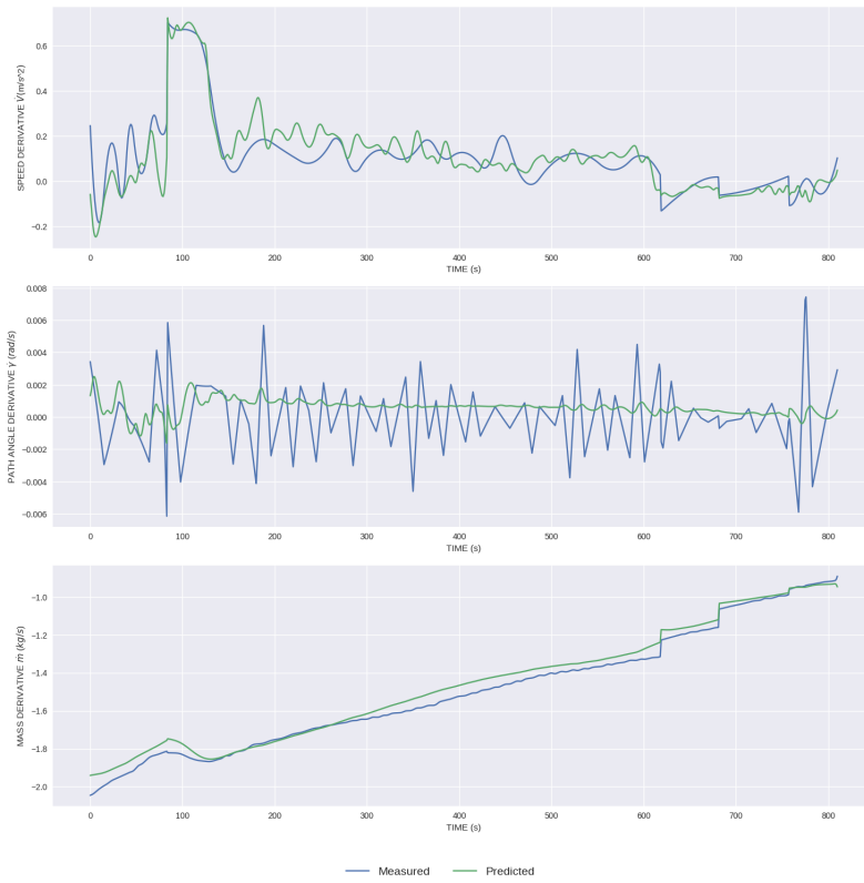
Figure 4.12 – Estimated states derivatives using the ALS solutions.
