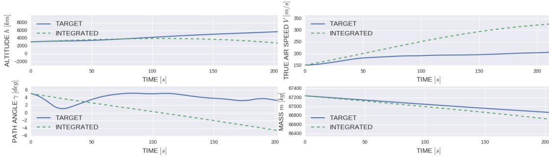
Figure 3.13 – (Dashed green) Direct integration of predicted dynamics of the beginning of a flight (using single-task OLS). (Blue) Observed states derivatives.
