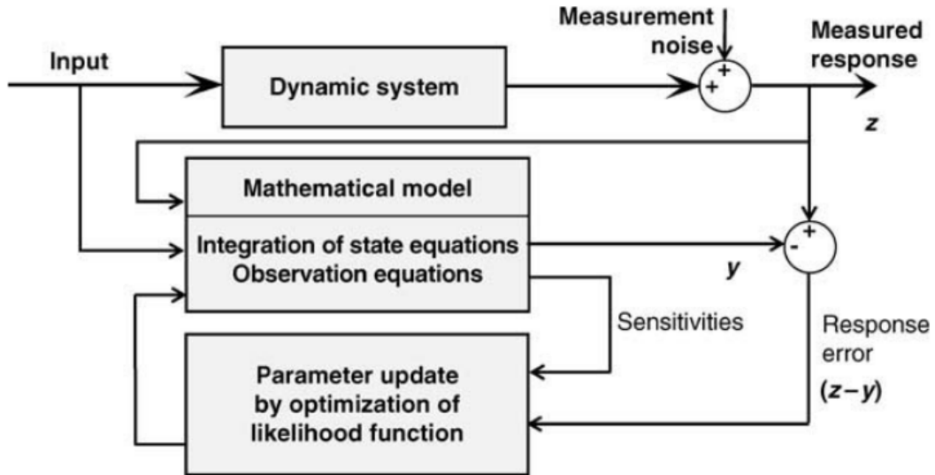
Figure 3.8 – Block schematic of Output-Error method (figure from [Jategaonkar, 2006, p.85]).
