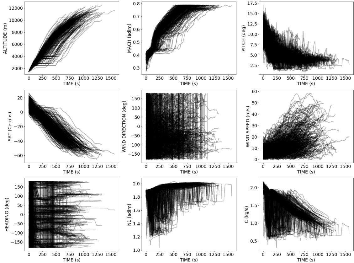
Figure 2.1 – Raw signals of 424 different flights extracted from the QAR of the same B737-800.
