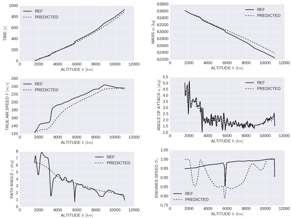
Figure 4.16 – Resimulated trajectory obtained by solving problem (4.6.1) with BOCOP.
