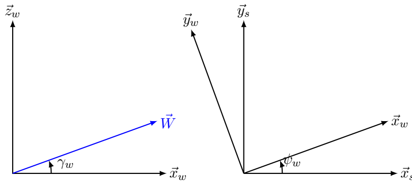
Figure 3.7 – \mathcal{R}_w rotation relative to \mathcal{R}_s ( = \mathcal{R}_i in subsection 3.2.5).
