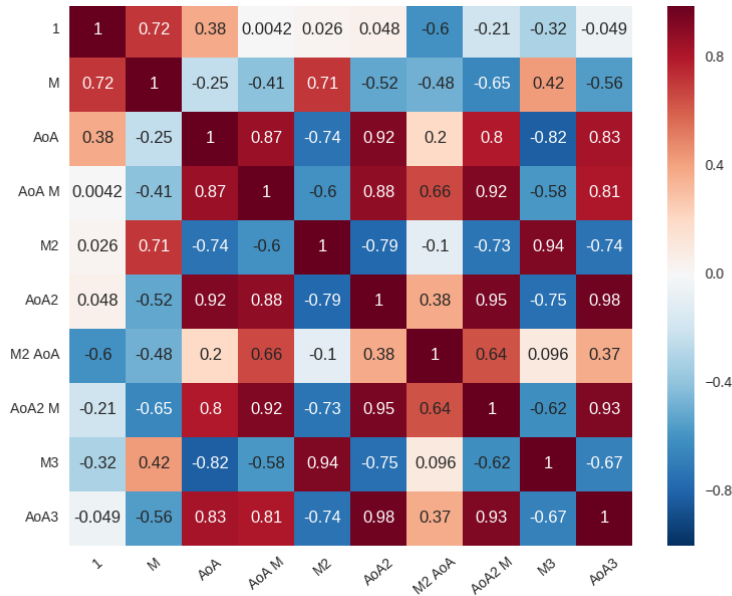
Figure 4.3 – Monomials correlation matrix of the Lift and Drag models.
