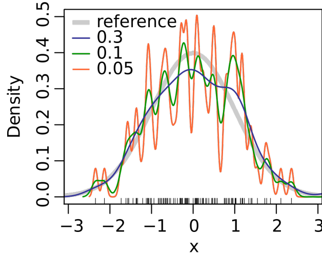
Figure 5.5 – Example of kernel density estimation using different bandwidth. The sample was drawn from a standard Gaussian distribution. 4
