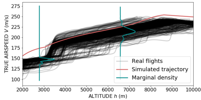
Figure 5.1 – Illustration of the marginal likelihoods.
