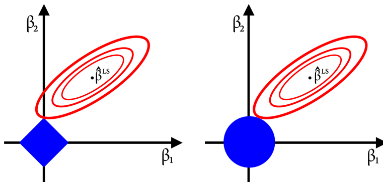
Figure 4.1 – The left frame shows the shape of the L^1 constraint of the Lasso in blue, the contours of the least-squares criterion being represented by the ellipsoids. The right frame represents the same, but with the squared L^2 constraint from the Ridge regression. The OLS solutions are denoted by \hat{\beta}^{LS} here. 1
