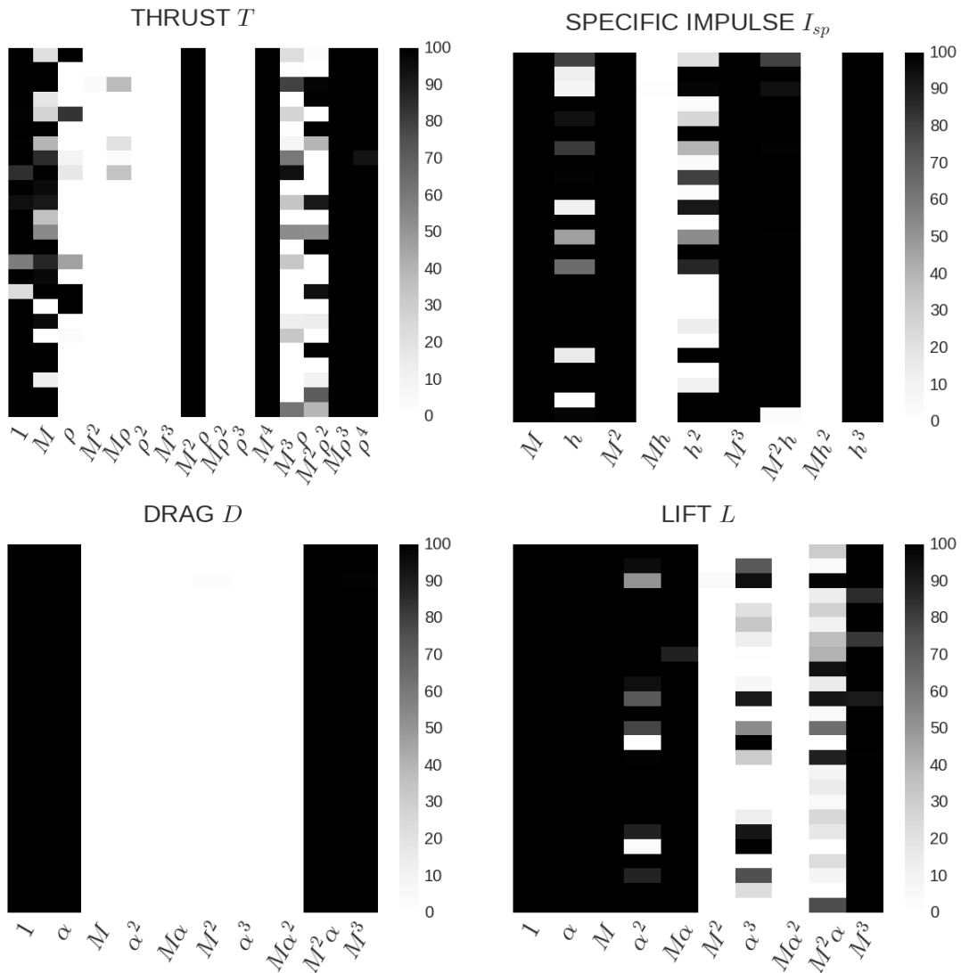
Figure 4.14 – Block sparse Bolasso selections for the thrust, drag, lift and specific impulse models. The columns correspond to possible features for T/N_1, D/q, L/q and I_{sp}/SAT .
