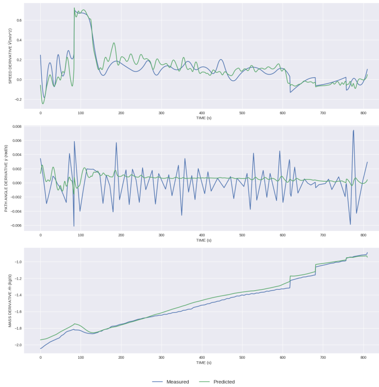
Figure 4.12 – Estimated states derivatives using the ALS solutions.
