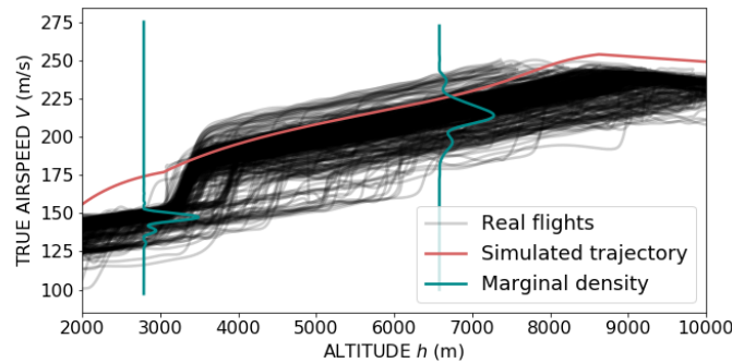
Figure 5.1 – Illustration of the marginal likelihoods.
