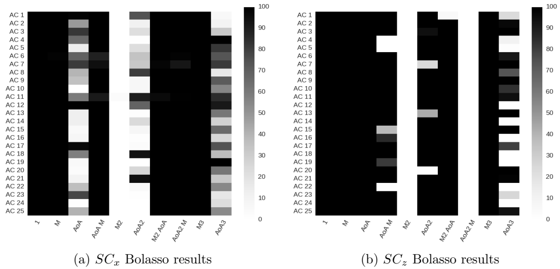
Figure 4.6 – Single-task aerodynamic features selection results with wind-dynamics.
