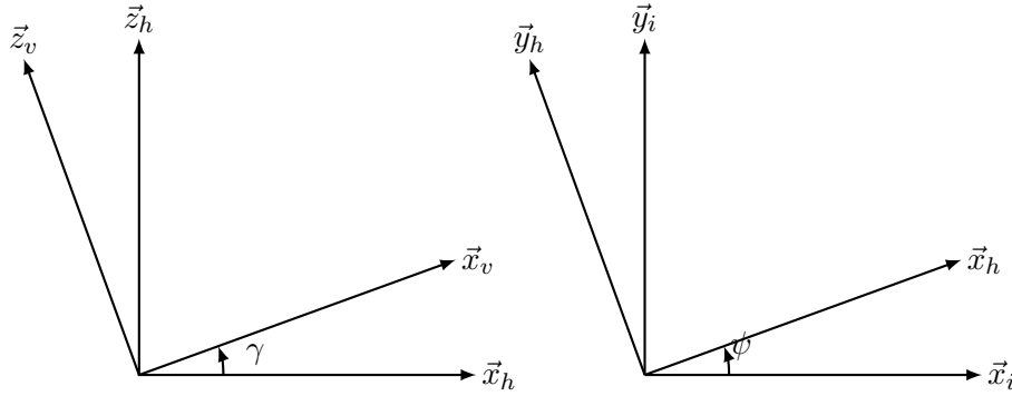
Figure 3.4 – \mathcal{R}_v rotation relative to \mathcal{R}_i in the case of a 3D trajectory with flat Earth assumption (2D representation).
