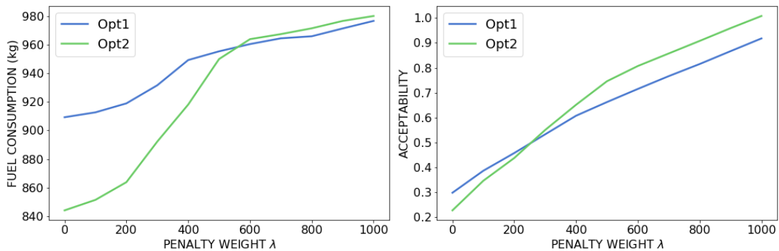
Figure 6.1 – Average over 20 flights of the total fuel consumption and MML score (called acceptability here) of optimized trajectories with varying MML-penalty weight \lambda .
