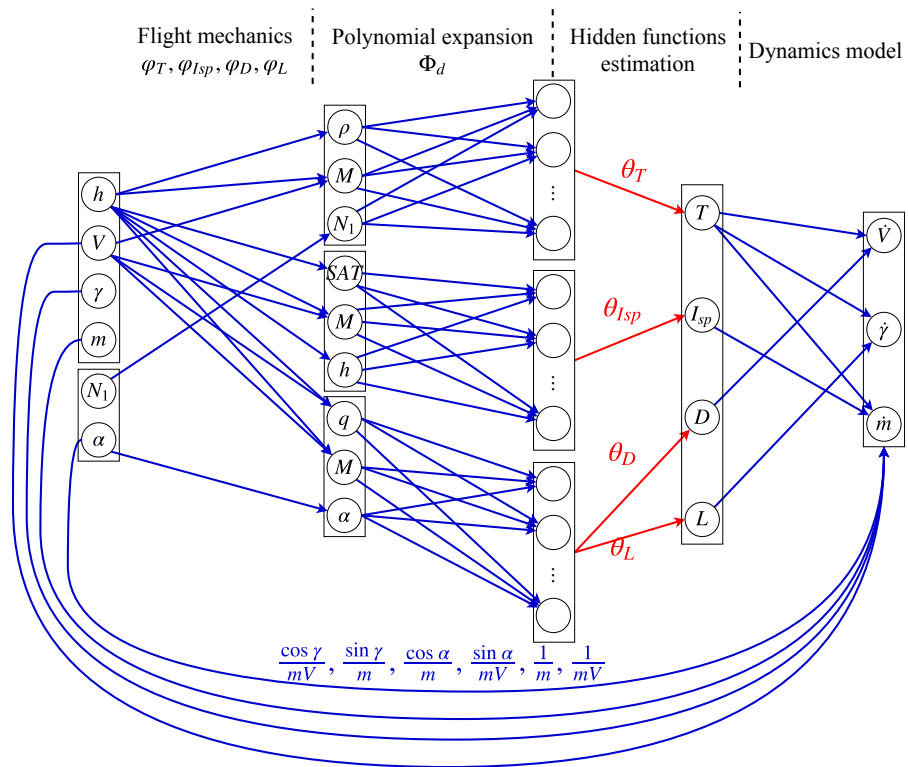
Figure 4.7 – General computational graph representing the layers of hidden features of the model. Blue arrows represent nonlinear transformations, while red arrows represent linear combinations.
