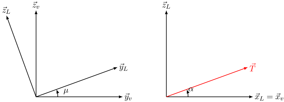
Figure 3.2 – \mathcal{R}_L rotation relative to \mathcal{R}_v .
