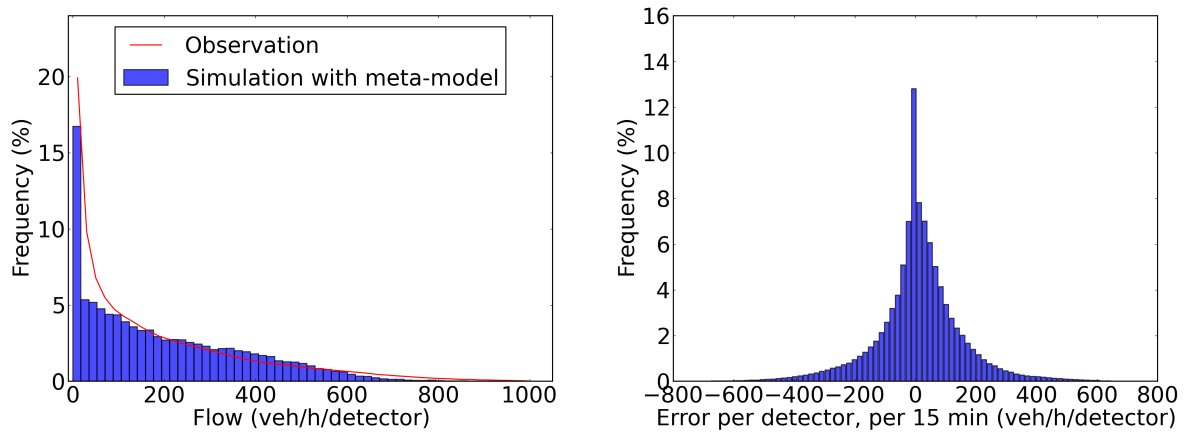
Figure 4.19: Left: the total distribution of the flows computed for each \Delta h on each detector, by the simulation with metamodel . Right: the distribution of error between the flows computed by metamodel and flows measured by detectors.
