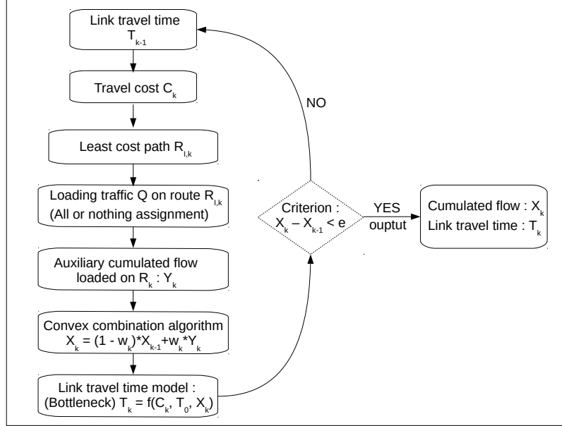
Figure 2.2: The algorithm framework of LTK software
