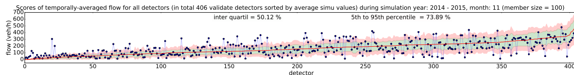
Figure 7.11: Statistical scores for the ensemble prediction of temporally-averaged traffic flows for all detectors. The loop detector observations are represented by blue points, averaged from observations of all 15 minute intervals for each detector during November 2014. The green color band delimits the values between the 25 th and 75 th percentiles of the temporally-averaged flows computed by the ensemble. The red color band delimits the values between the 5 th and 95 th percentiles of the temporally-averaged flows computed by the ensemble. The detectors are sorted from left to the right with respect to the mean of temporally-averaged flows estimated by the ensemble (plotted by the red line).
