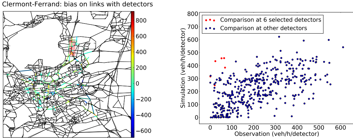
Figure 4.6: Left: map of bias (in \text{veh h}^{-1} \text{link}^{-1} ) between the temporally-averaged flows computed by LCF on each link and the measured flows, on the 20 th November 2014. (In the red rectangle, the links with overestimated flows have detectors only on left-turn lanes.) Right: scatter plot of the temporally-averaged flows on each detector. (The red points match the simulation-observation comparison at detectors located on left-turning lanes in the red-rectangle zone of the left figure.)
