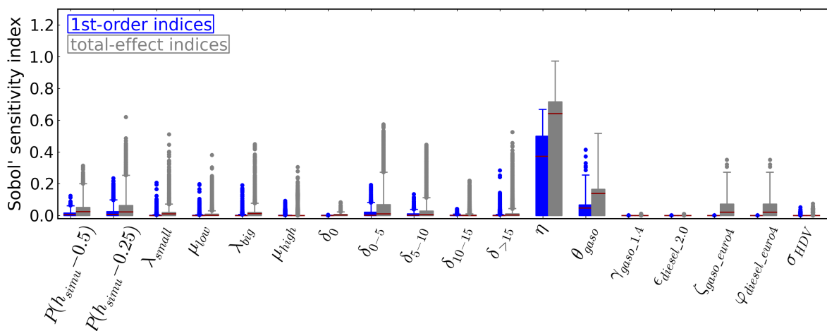
Figure 6.13: First-order and total-effect Sobol' sensitivity index of some inputs of modeling chain of Meta-LCF-COPERT IV, for the computed traffic emissions of CO
