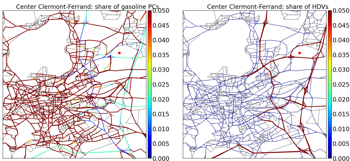
Figure 6.12: Spatial distribution of the 1st order sensitivity indices of the computed NOx emissions with respect to the share of gasoline passenger cars \theta_{\text{gaso}} (left) and heavy duty vehicles \sigma_{\text{HDV}} (right). The red point in the map represents a big industrial logistic center.
