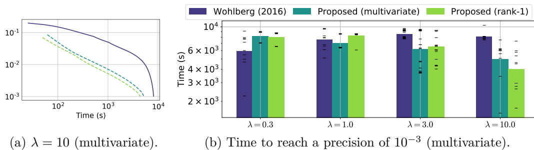
Figure 5.12 – Comparison of state-of-the-art multivariate methods, using P = 5 channels. (a) Convergence plot with the objective function relative to the obtained minimum, as a function of computational time. (b) Time taken to reach a relative precision of 10^{-3} , for different regularization parameters \lambda .
