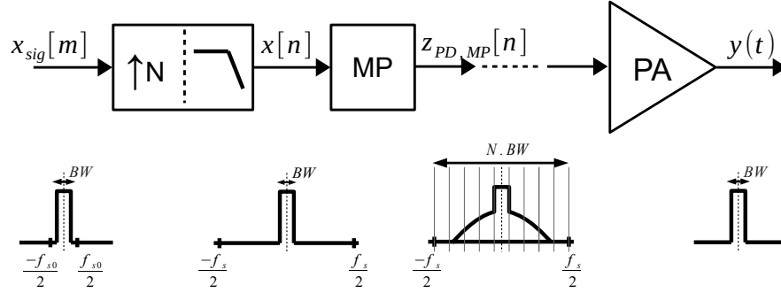
FIGURE 3.1: Illustration of MP predistorter
