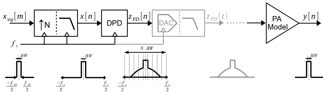
FIGURE 4.1: Simulation testbench for the DPD
