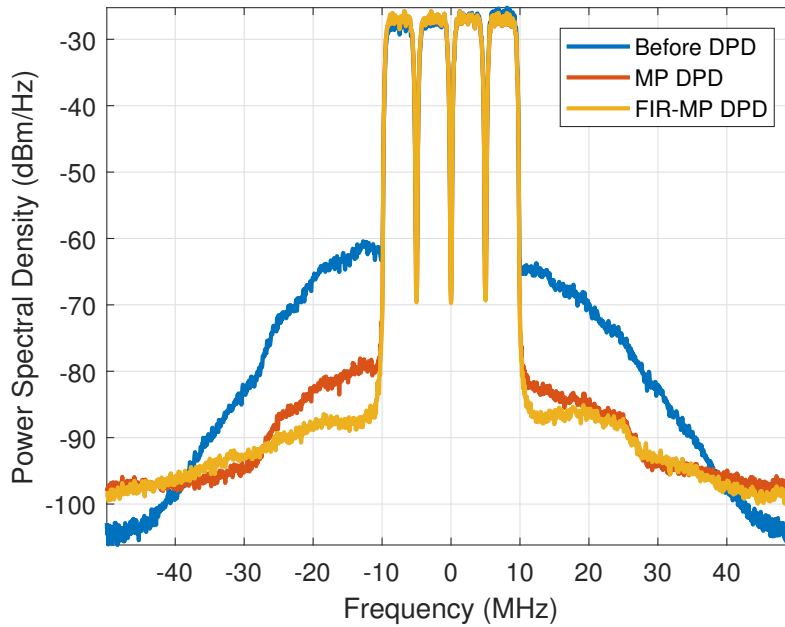
FIGURE 3.23: Power spectra of the output before and after linearization for a 4 carrier WCDMA signal with a total bandwidth of 20 MHz and PAPR of 8.4 dB. ACLR1 improvement of 7.2 dB is obtained using FIR-MP.
