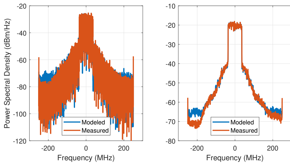
FIGURE 3.15: Spectra of the measured and modeled PA output. Spectra on the left is obtained with a single spectrum for both measured and modeled data and the spectra on the right is obtained by averaging
