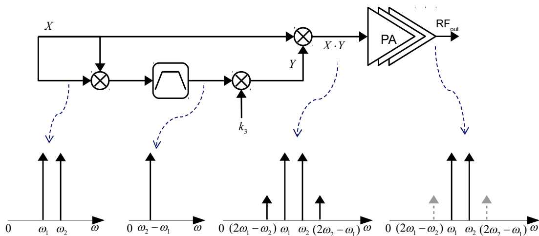
FIGURE A.1: Illustration of predistortion signal generation for the case of two-tone signal.
