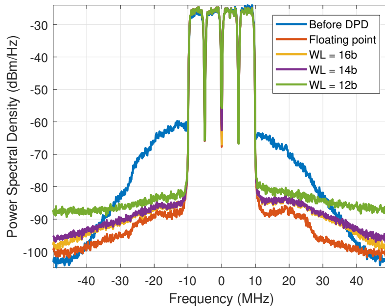
FIGURE 3.26: Spectra of the output signal without DPD and with floating-point and fixed-point representations of 16 bits, 14 bits and 12 bits for 20 MHz signal
