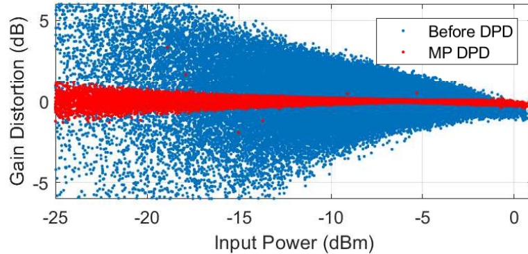
FIGURE 3.2: AM/AM plot without and with MP predistorter for a 4 carrier modulated signal with a total bandwidth of 80 MHz and PAPR of 8.4 dB
