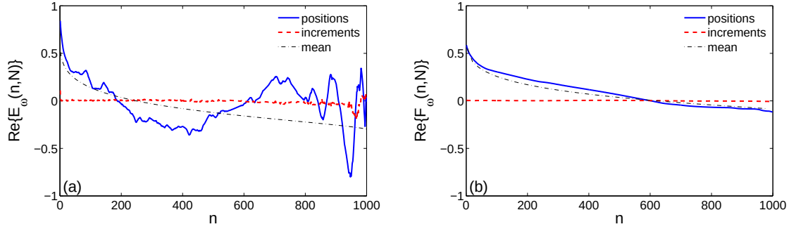
Figure 2.13: The real parts of the mixing (a) and ergodicity (b) estimators at \omega = 1 applied to the increments of a single CTRW trajectory (dashed line) and to the positions of the same trajectory (solid line), with N = 1000 , \alpha = 0.7 , and \sigma = 1 . In both cases, X(n) are normalized by the empirical standard deviation of the increments. Thin dash-dotted line presents the mean estimators from Eqs. (2.51, 2.52).
