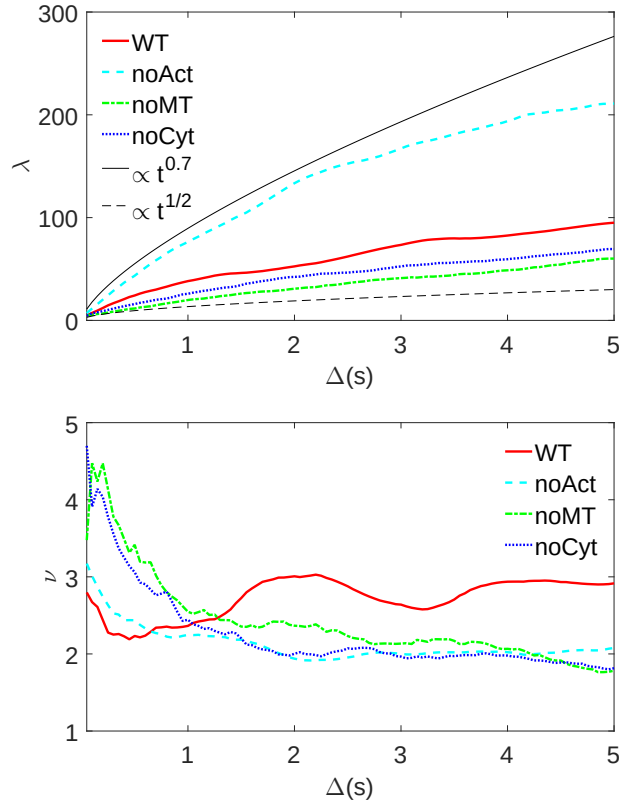
Figure 5.16: Parameters \lambda ( top ) and \nu ( bottom ) fitted at each lag-time \Delta for four cytoskeleton states: Wild type ( red line ), depolymerized actin ( cyan dashed line ), disrupted microtubules ( dash-dotted green line ), and deprived of both actin and microtubules ( dotted blue line ). black line (resp. dotted black line ) is visual guideline \propto \Delta^{0.7}(s) (resp. \propto \Delta^{0.5}(s) ).
