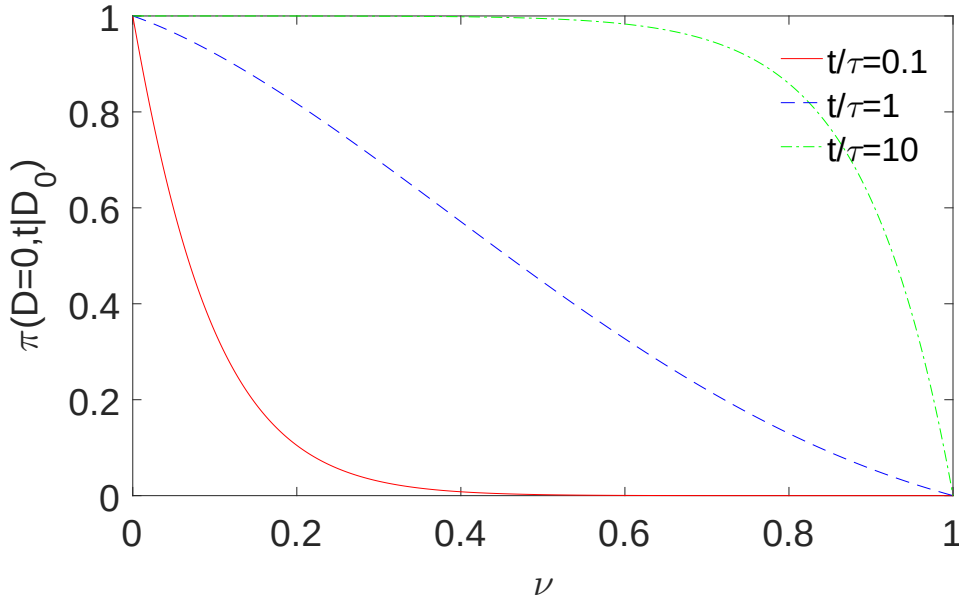
Figure 4.5: Probability of D = 0 as a function of \nu for three different dimensionless times t/\tau = \{0.1, 1, 10\} . \nu is varied from 0 to 1 by keeping \sigma = 1 , \tau = 10 and adjusting \bar{D} = \nu\sigma^2\tau with initial diffusivity D_0 = \bar{D} .
