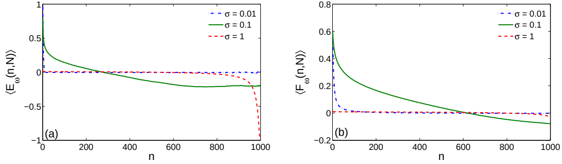
Figure 2.6: The mean mixing (a) and ergodicity (b) estimators at \omega = 1 as a function of n for geometric Brownian motion with \mu = 0 and \sigma = 0.01 , \sigma = 0.1 , and \sigma = 1 . Each generated trajectory was normalized by the empirical standard deviation of its increments in order to get comparable results for different \sigma . The mean was computed numerically by averaging over 1000 trajectories.
