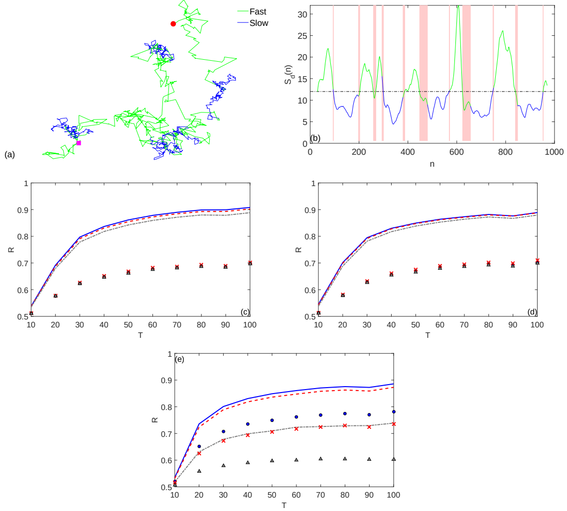
Figure 3.7: Model 5 (a) A single trajectory of an intermittent process, alternating a “slow” phase of planar Brownian motion (with D = 1/2 , dark blue) and a “fast” phase of two-dimensional exponential flights (with \ell = 3 , light green), of the mean phase duration T = 100 . Circle and square indicate the starting and ending points. (b) The weighted LCH diameter S_d(n) with the window size \Delta = 10 applied to this trajectory. Pink shadow highlights the false classification zones. Dashed horizontal line shows the empirical mean S_d over that trajectory. (c,d,e) Recognition score R of the diameter-based discriminator S_d(n) (c), the volume-based discriminator S_v(n) (d), and the TA MSD-based discriminator (e) as a function of the mean phase duration T . Lines show the results for the case \ell = 3 with three noise levels \sigma_n : 0 (blue solid), 0.5\sigma (red dashed), and \sigma (gray dash-dotted) ( \sigma being the empirical standard deviation of increment calculated for each trajectory). Symbols correspond to the case \ell = \sqrt{2} with the same levels of noise \sigma_n : 0 (circles), 0.5\sigma (crosses), and \sigma (triangles).
