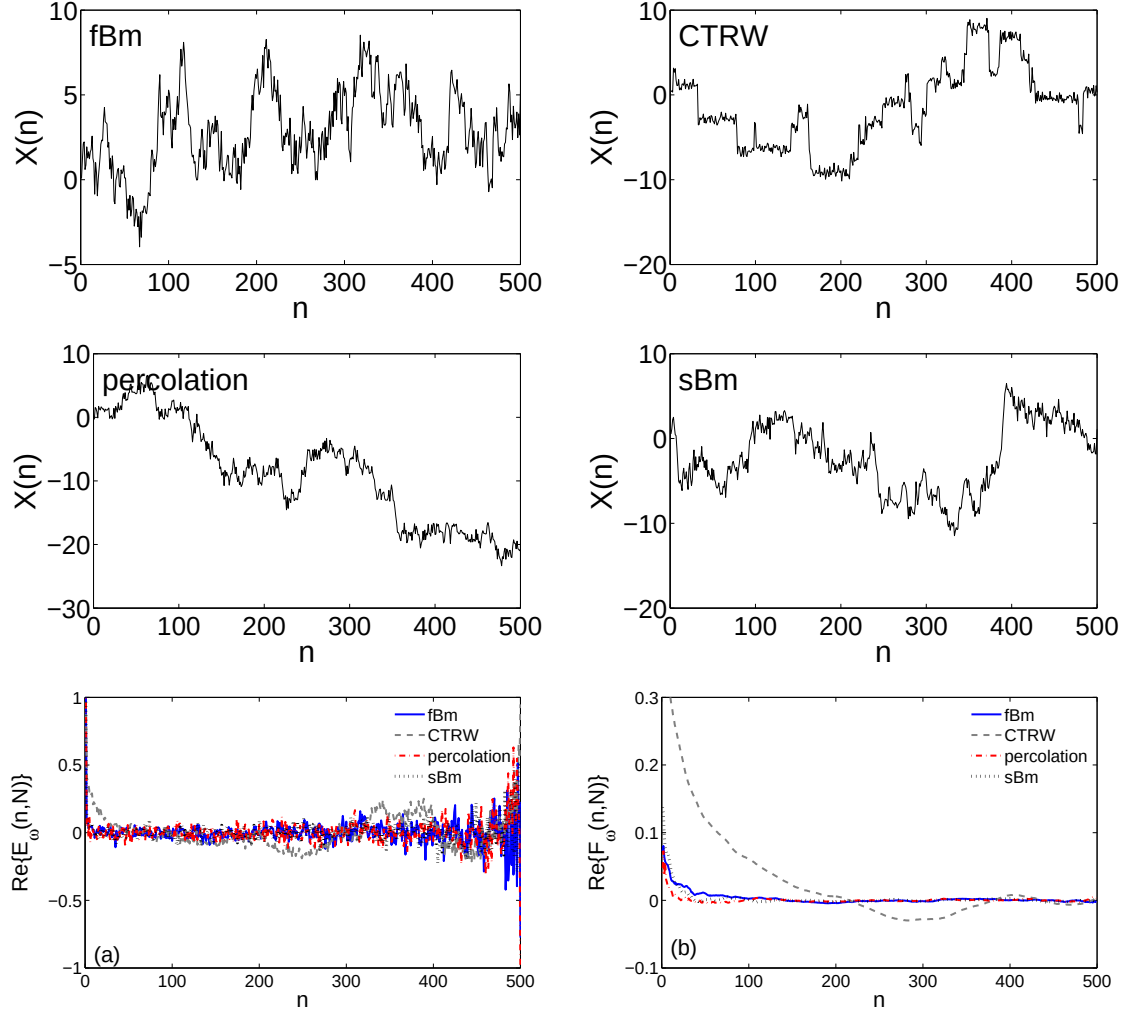
Figure 2.8: (Top) . Examples of trajectories of four anomalous diffusion models: fBm, CTRW, diffusion on percolating clusters, and sBm, with the same scaling exponent \alpha = 0.7 and one-step size \sigma = 1 . Each trajectory was corrupted by the white Gaussian noise of level \sigma_\varepsilon = 0.2 and then normalized by the empirical standard deviation of its increments. (Bottom) . The real part of the mixing and ergodicity estimators at \omega = 2 applied to these four trajectories.
