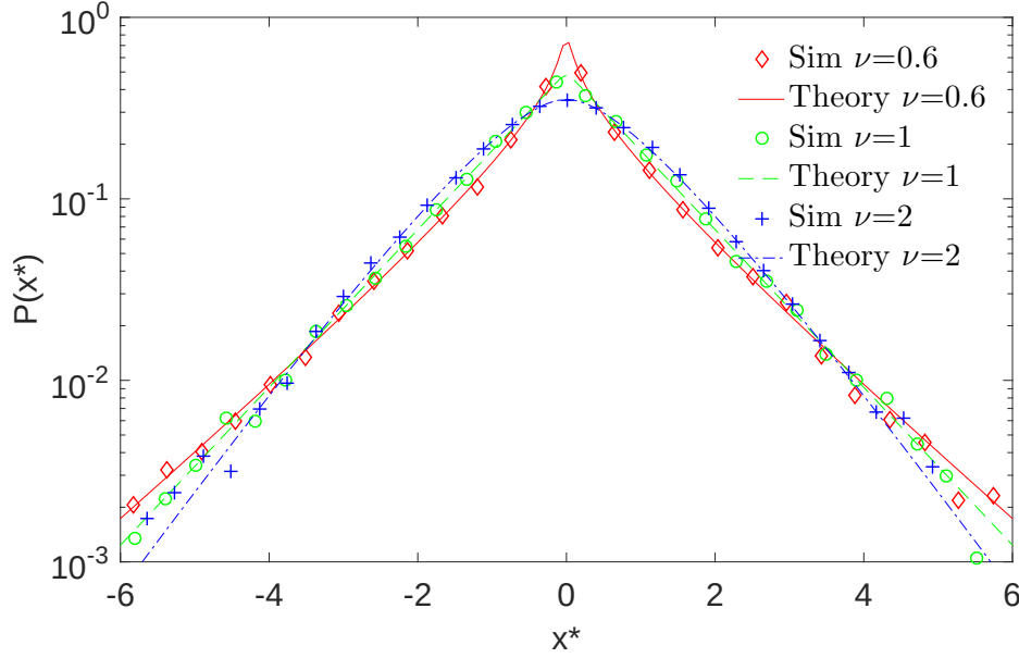
Figure 4.2: Distribution of normalized displacements, with x^* = x/\sqrt{\bar{D}t} , at fixed time t = 1 for different parameters \nu = \{0.6, 1, 2\} . For each case, we kept \bar{D} = 1 and \tau = 100 and varied \sigma . Theoretical results (lines) are compared to Monte Carlo simulations (symbols) with M = 10^6 particles.
