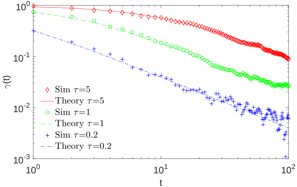
Figure 4.6: The non-Gaussian parameter calculated from Eq. (4.85) (lines) and from Monte Carlo simulations (symbols) with M = 10^5 particles, for different values of \tau = \{0.2, 1, 5\} , while keeping \nu = 1 , \bar{D} = 1 and \sigma = 1/\sqrt{\tau} .
