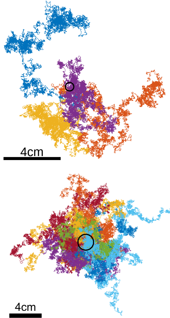
Figure 5.1: (Top) Example of random trajectories of 4 disks that were originally located close to each other (inside the black circle) and then diffused during 600 seconds (i.e., 15 000 points in each trajectory). (Bottom) Example of random trajectories of 34 disks that were originally located close to each other and then diffused during 464.6 seconds (i.e., 11 615 points in each trajectory).
