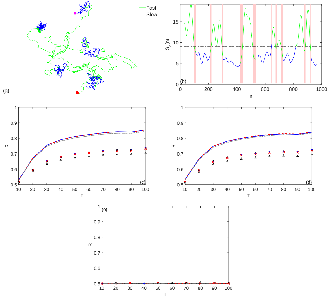
Figure 3.5: Model 3 (a) A single trajectory of planar fBm, alternating a “slow” phase ( H_1 = 0.35 , dark blue) and a “fast” phase ( H_2 = 0.7 , light green), of the mean phase duration T = 100 and D_H = 1/2 . Circle and square indicate the starting and ending points. (b) The weighted LCH diameter S_d(n) with the window size \Delta = 10 applied to this trajectory. Pink shadow highlights the false classification zones. Dashed horizontal line shows the empirical mean S_d over that trajectory. (c,d,e) Recognition score R of the diameter-based discriminator S_d(n) (c), the volume-based discriminator S_v(n) (d), and the TA MSD-based discriminator (e) as a function of the mean phase duration T . Lines show the results for the case H_1 = 0.35 , H_2 = 0.7 with three noise levels \sigma_n : 0 (blue solid), 0.5\sigma (red dashed), and \sigma (gray dash-dotted) ( \sigma being the empirical standard deviation of increment calculated for each trajectory). Symbols correspond to the case H_1 = 0.35 , H_2 = 0.5 with the same levels of noise \sigma_n : 0 (circles), 0.5\sigma (crosses), and \sigma (triangles).
