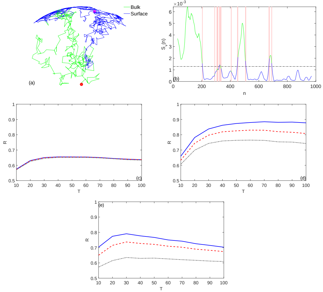
Figure 3.8: Model 6 (a) A single trajectory of surface-mediated diffusion in a three-dimensional sphere of radius R = 1 , alternating bulk diffusion (light green) and surface diffusion (dark blue), with D_{2d} = D_{3d} = 10^{-3} and \lambda = 10^{-2} . Circle and square indicate the starting and ending points. (b) The weighted LCH diameter S_d(n) with the window size \Delta = 10 applied to this trajectory. Pink shadow highlights the false classification zones. Dashed horizontal line shows the empirical mean S_d over that trajectory. (c,d,e) Recognition score R of the diameter-based discriminator S_d(n) (c), the volume-based discriminator S_v(n) (d), and the TA MSD-based discriminator (e) as a function of the mean duration of the surface phase T = 1/\lambda . Three curves correspond to three noise levels \sigma_n : 0, 0.5\sigma , and \sigma ( \sigma being the empirical standard deviation of increment calculated for each trajectory).
