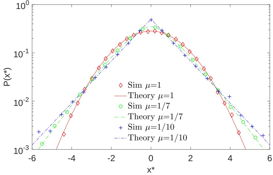
Figure 4.3: Distribution of normalized displacements, with x^* = x/\sqrt{\bar{D}t} , at fixed time t = 1 , with \mu(t) from Eq. (4.20) being varied in the range \{1/10, 1/7, 1\} corresponding to \nu = \{1, 2, 100\} , by changing \sigma and keeping \bar{D} = 1 and \tau = 100 . Theoretical results (lines) are compared to Monte Carlo simulations (symbols) with M = 10^6 particles.
