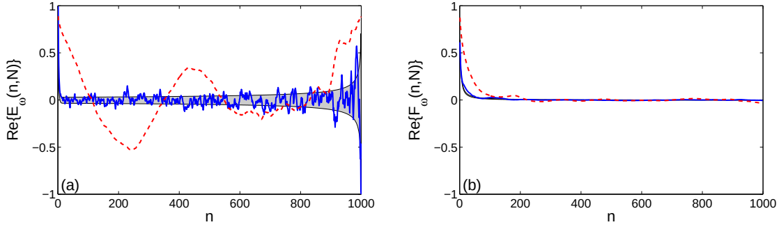
Figure 2.17: The real part of the mixing (a) and ergodicity (b) estimators at \omega = 1 as a function of n for an original Brownian motion trajectory with N = 1000 and \sigma = 1 (solid line) and for the same trajectory corrupted by resetting ten randomly chosen points to 0 (dashed line). In both cases, the trajectory was normalized by the empirical standard deviation of its increments. Light gray shadowed region delimits the mean plus and minus the standard deviation of each estimator computed for Brownian motion according to Eqs. (2.11, 2.12, 2.17, 2.18).
