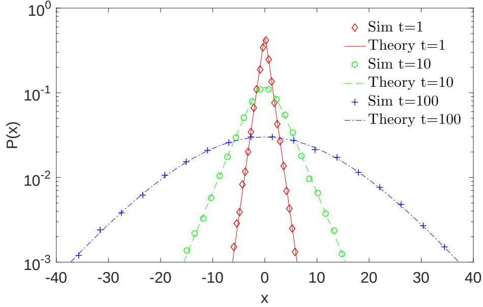
Figure 4.1: Distribution of displacements at times t = \{1, 10, 100\} . Here \tau = 10 , \bar{D} = 1 , \sigma = 1/\sqrt{\tau} and thus \nu = 1 . Theoretical results (lines) are compared to Monte Carlo simulations (symbols) with M = 10^6 particles.
