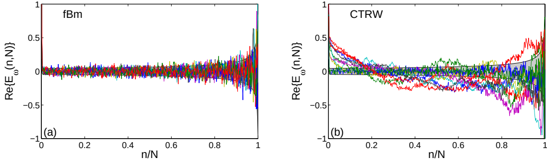
Figure 2.9: The real part of the mixing estimator at \omega = 2 for ten simulated trajectories from two anomalous diffusion models: ergodic fBm with 2H = 0.7 (a) and nonergodic CTRW with the same exponent \alpha = 0.7 (b) (in both cases, we set \sigma = 1 and N = 500 ). All trajectories were corrupted by white Gaussian noise with standard deviation \sigma_\varepsilon = 0.1 . Each trajectory is normalized by the empirical standard deviation of its increments. Light gray shadowed region delimits the typical range of fluctuations for Brownian motion, i.e., the mean plus and minus the standard deviation.
