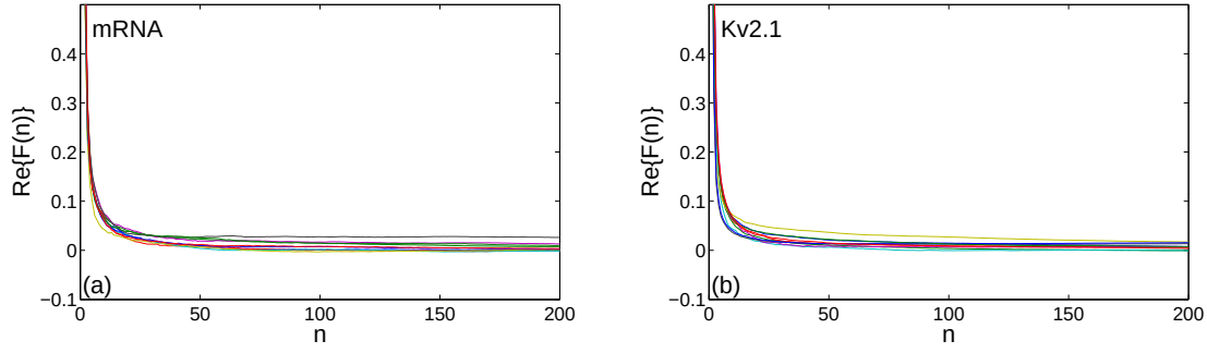
Figure 2.14: The real part of the original ergodicity estimator, \text{Re}\{n^{-1} \sum_{k=0}^{n-1} \hat{E}(k)\} from [175], applied to ten experimental trajectories of two samples: (a) the motion of mRNA molecules inside live E. coli cells [106] and (b) Kv2.1 potassium channel anomalous dynamics in the plasma membrane [280]. The estimator is applied to the increments of each trajectory which are normalized by their empirical standard deviation. The trajectory length ranges between 400-500 points for the first set and around 1500 points for the second set.
