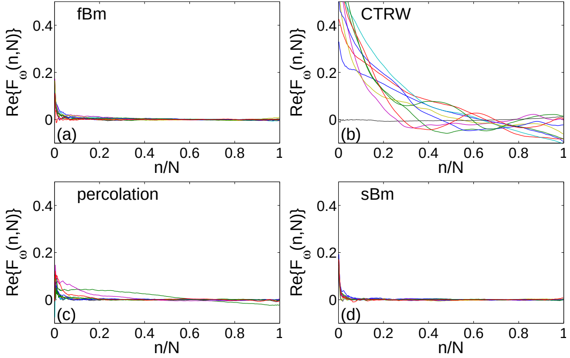
Figure 2.10: The real part of the ergodicity estimator at \omega = 2 for ten simulated trajectories from four anomalous diffusion models with the same exponent \alpha = 2H = 0.7 : fBm (a), CTRW (b), diffusion on percolating cluster (c), and sBm (d) (in all cases, we set \sigma = 1 and N = 500 ). All trajectories were corrupted by white Gaussian noise with standard deviation \sigma_\varepsilon = 0.1 . Each trajectory was normalized by the empirical standard deviation of its increments.
