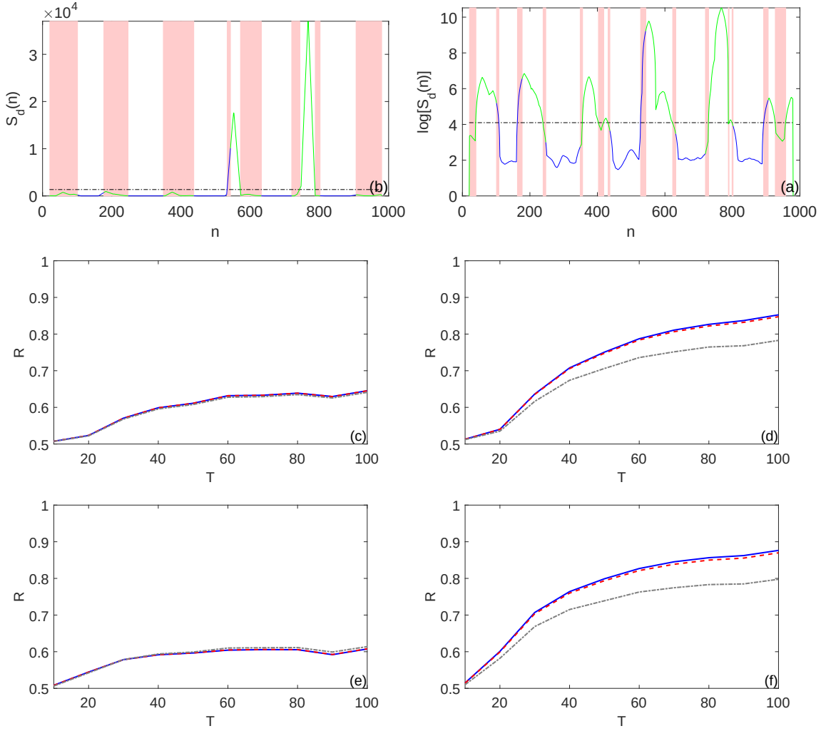
Figure 3.9: (a,b) Results for a two-dimensional intermittent process, alternating a “slow” phase of Brownian motion with standard deviation of increments in each dimension \sigma = 1 (blue) and a “fast” phase of Lévy walk with stable increments of parameters \alpha = 0.7 , \beta = 1 , \sigma = 1 , and \mu = 0 (light green). (a) The weighted LCH diameter S_d(n) with the window size \Delta = 10 applied to a single trajectory of length N = 1000 . Dotted line shows the empirical average of S_d . (b) The logarithm of S_d(n) from (a). Dotted line shows the empirical average of \log S_d . (a,b) Pink shadow highlights the false classification zones. (c,e) Recognition score R of the diameter-based discriminator S_d(n) , and (c) and the volume-based discriminator S_v(n) (e) . (d,f) Recognition score R of the diameter-based discriminator \log S_d(n) (d) and the volume-based discriminator \log S_v(n) (f) . (c,d,e,f) Plot as a function of the mean phase duration T . Lines show the results with three noise levels \sigma_n : 0 (blue solid), \sigma (red dashed), and 10\sigma (gray dash-dotted) ( \sigma being the standard deviation of increments of the Brownian phase).
