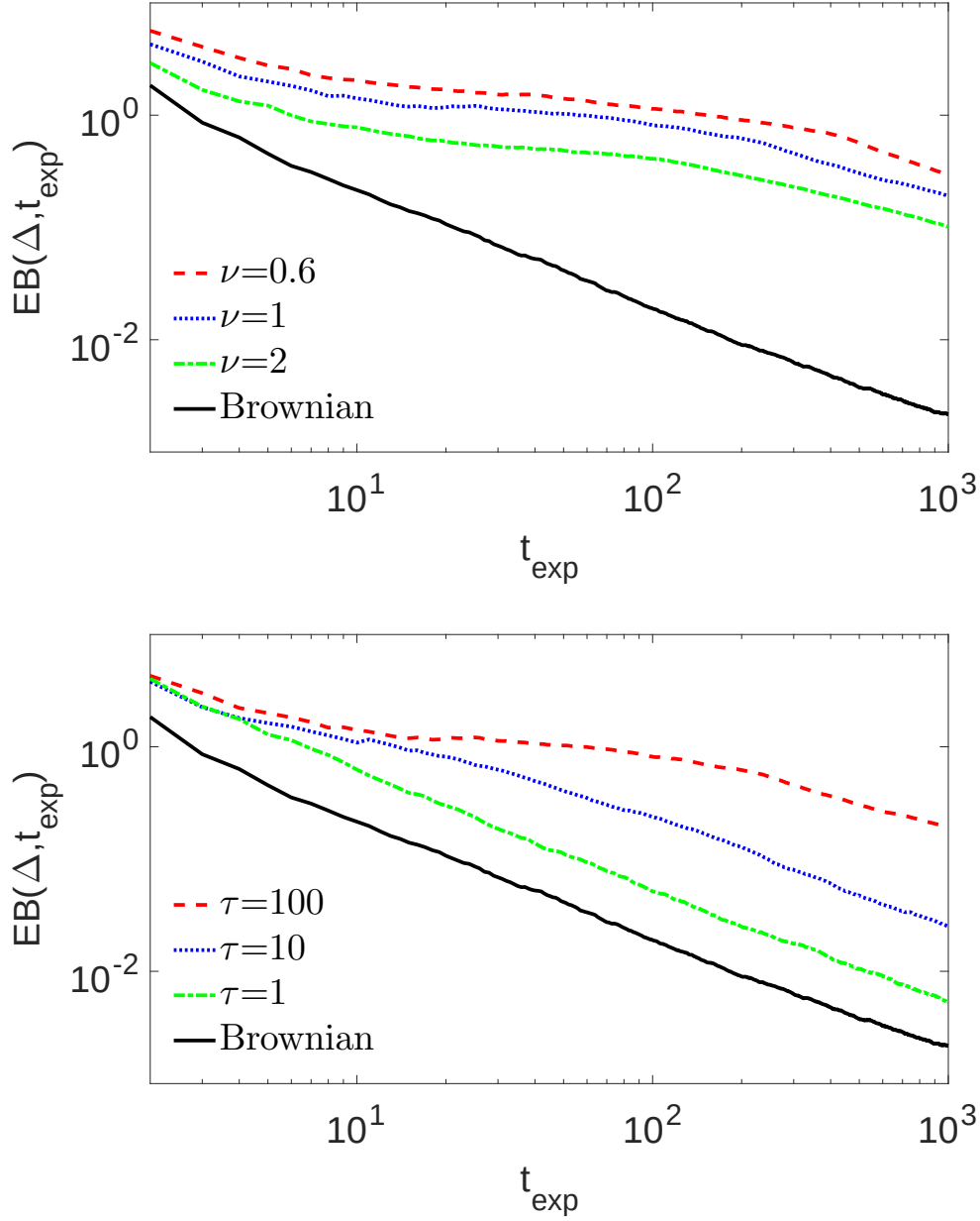
Figure 4.7: Ergodicity breaking parameter calculated by averaging over M = 10^3 simulated trajectory of length t_{\text{exp}} = 10^3 . The result for Brownian motion (solid line) is also plotted for comparison. Top. Results for variable shape parameter \nu = \{0.6, 1, 2\} by varying \tau , with \bar{D} = 1 and \sigma = 1 being constant. Bottom. Results for variable correlation time \tau = \{1, 10, 100\} while keeping \nu = 1 , \bar{D} = 1 and \sigma = 1/\sqrt{\tau} .
