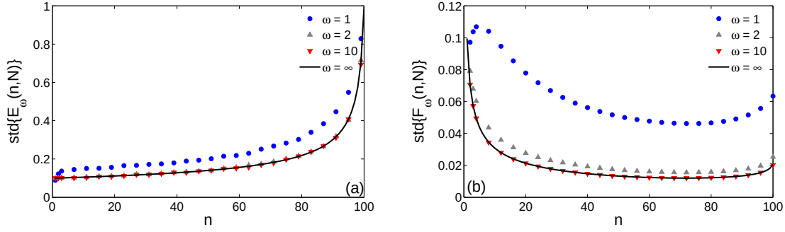
Figure 2.2: The standard deviation of the mixing (a) and ergodicity (b) estimators at several values of \omega for Brownian motion with N = 100 and \sigma = 1 . The large \omega asymptotic limits given by square roots of Eqs. (2.17, 2.18) are shown by solid lines.
