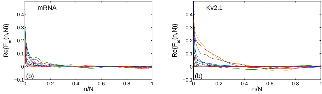
Figure 2.12: The real part of the ergodicity estimator at \omega = 2 for ten experimental trajectories of two samples: the motion of mRNA molecules inside live E. coli cells [106] and Kv2.1 potassium channel anomalous dynamics in the plasma membrane [280]. Each trajectory is normalized by the empirical standard deviation of its increments. The trajectory length ranges between 400-500 points for the first set and around 1500 points for the second set. Light gray shadowed region delimits the typical range of fluctuations for Brownian motion, i.e., the mean plus and minus the standard deviation.
