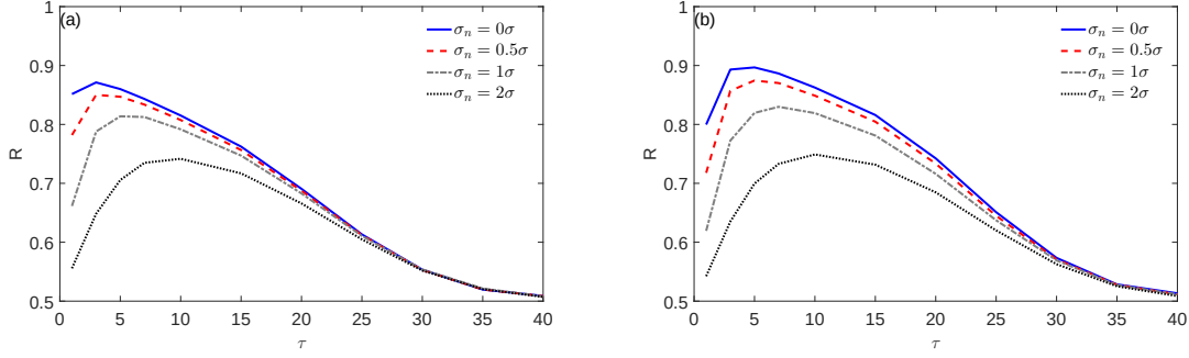
Figure 3.10: Effect of the window size \Delta on the recognition score R for intermittent Brownian motion (Model 1) with D_1 = 1/2 , D_2 = 2 , and the mean phase durations T_1 = T_2 = 40 . (a) The diameter-based discriminator S_d(n) ; (b) the volume-based discriminator S_v(n) . Four curves correspond to four noise levels \sigma_n : 0 , 0.5\sigma , \sigma , and 2\sigma ( \sigma being the empirical standard deviation of increment calculated for each trajectory).
