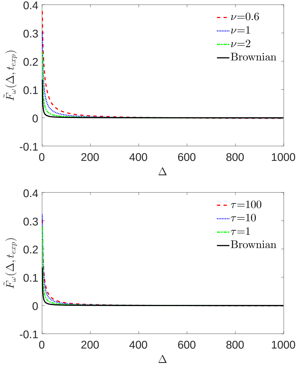
Figure 4.8: Mean ergodicity estimator \tilde{F}_\omega(\Delta, t_{exp}) , calculated with M = 10^3 simulated trajectories of length t_{exp} = 10^3 . The mean estimator for Brownian motion (solid line) is also plotted for comparison. Top. Different values of the shape parameter \nu = \{0.6, 1, 2\} by varying \tau , with \bar{D} = 1 and \sigma = 1/\sqrt{\tau} . Bottom. Different values of \tau = \{1, 10, 100\} while keeping \nu = 1 , \bar{D} = 1 and \sigma = 1/\sqrt{\tau} .
