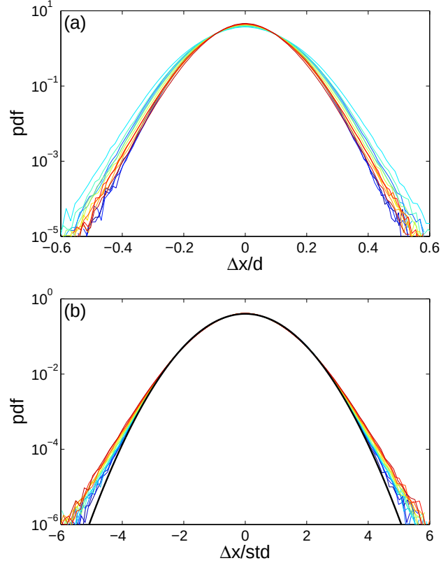
Figure 5.2: (a) The empirical distributions of one-step one-dimensional increments for 14 samples (in units of the disk diameter, d = 4 mm). (b) The empirical distributions of rescaled one-step increments for 14 samples. Thick black curve shows the standard Gaussian density e^{-x^2/2}/\sqrt{2\pi} . Color of thin curves changes from dark blue for the lowest packing fraction \phi to dark red for the highest one.
