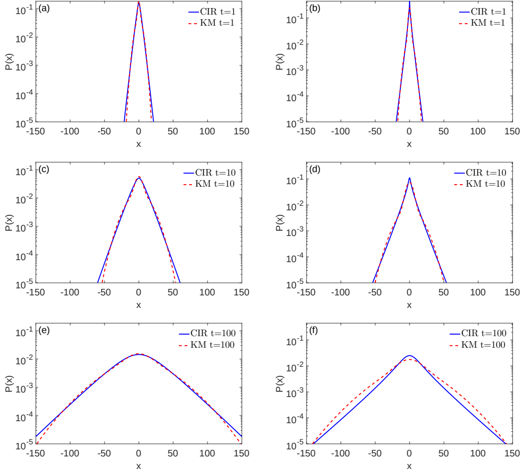
Figure 4.9: Distribution of displacements for the Karger model (dashed lines) and our model (solid lines) at time t = 1 (top), t = 10 (middle), t = 100 (bottom). We choose the parameters for the Karger model and deduce \bar{D} = p_1 D_1 + p_2 D_2 and \sigma = \sqrt{\bar{D}\eta/\tau} . Left column. Parameters of the Karger model are p_1 = 1/2 , p_2 = 1/2 , D_1 = 1 and D_2 = 10 and \tau = 10 , leading to \nu \approx 1.5 . Right column. Parameters of the Karger model are p_1 = 4/5 , p_2 = 1/5 , D_1 = 1 and D_2 = 10 and \tau = 10 , leading to \nu \approx 0.6 .
