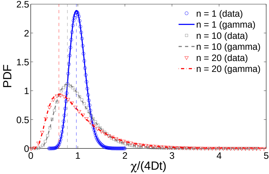
Figure 5.7: Probability density functions of the rescaled TAMSD, \chi_{n,N}/(4Dt) , for the sample with the lowest packing fraction, with N = 100 , t = n\delta , and n = 1 (blue circle), n = 10 (gray squares), and n = 20 (red triangles). Lines show the generalized gamma distribution p(z) from Eq. (5.5) whose parameters were obtained from the first three moments (see the text): a = 3.27 , b = 0.03 , \nu = 28.13 ( n = 1 ), a = 1.94 , b = 0.27 , \nu = 1.34 ( n = 10 ), and a = 1.03 , b = 0.58 , \nu = 0.31 ( n = 20 ). The modes of these distributions are shown by vertical dashed lines: 0.97 ( n = 1 ), 0.78 ( n = 10 ), and 0.60 ( n = 20 ), whereas the mean is fixed to be 1 by rescaling.
