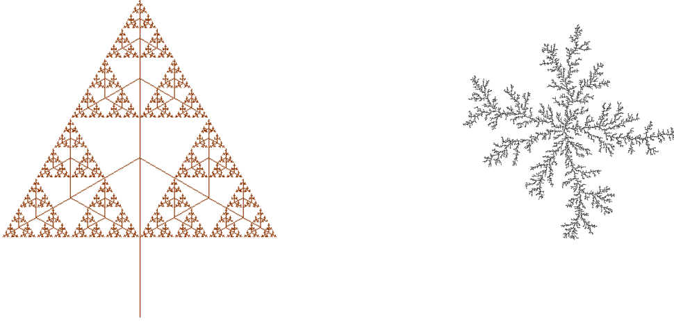
Figure 1.2: Two examples where the Alexander-Orbach relation does not hold. Left. A fractal tree at the sixth generation with three new branches at each generation. Right. A diffusion limited aggregation cluster simulated on a square lattice with 10000 aggregated particles [133, 287].
