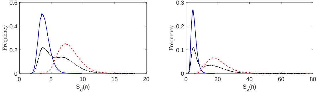
Figure 3.3: Distribution of S_d(n) ( Left ) S_v(n) ( Right ) for one trajectory of N = 10^6 steps of planar Brownian motion with diffusion coefficient D = 1/2 (blue curve) and D = 2 (dashed red curve) as well as an intermittent Brownian motion alternating the two previous diffusion coefficients (dashed black curve) with mean phase duration \lambda = 100 calculated for \Delta = 10 .
