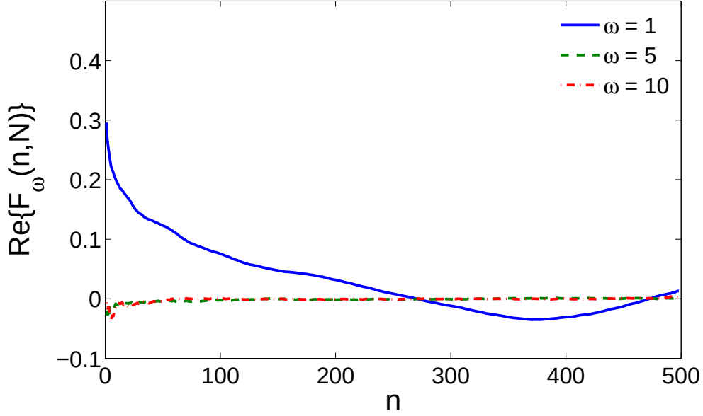
Figure 2.15: The real part of the ergodicity estimator as a function of n for a single fGn trajectory with N = 500 , H = 0.9 , and \sigma = 1 . At \omega = 1 (solid line), the estimator deviates from zero that may wrongly suggest nonergodic behavior. Increasing \omega , one can eliminate this false conclusion.
