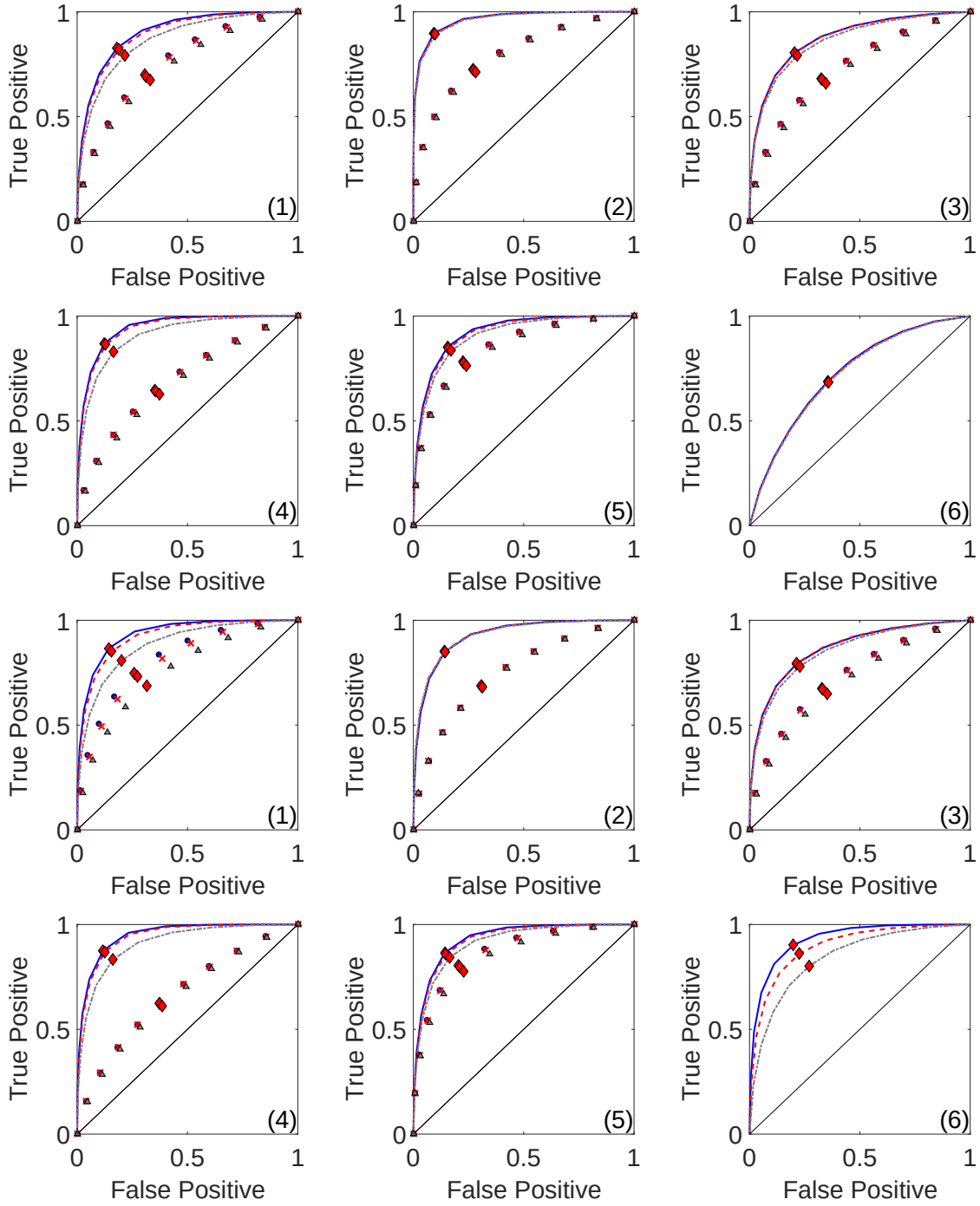
Figure 3.11: Effect of the threshold on the recognition quality for six models (following the enumeration at the beginning of Sec. 3.3), for the diameter-based discriminator (top 6 plots) and the volume-based discriminator (bottom 6 plots). The left upper corner and the right lower corner correspond to the threshold at the minimal and the maximal values, whereas diamonds indicate the mean value S_d (or S_v ) used as the threshold throughout the chapter. Legend of six curves on each plot is the same as in Figs. 3.2, 3.4, 3.5, 3.6, 3.7, 3.8 for the recognition score (three levels of noise and two sets of model parameters, except for the Model 6).
