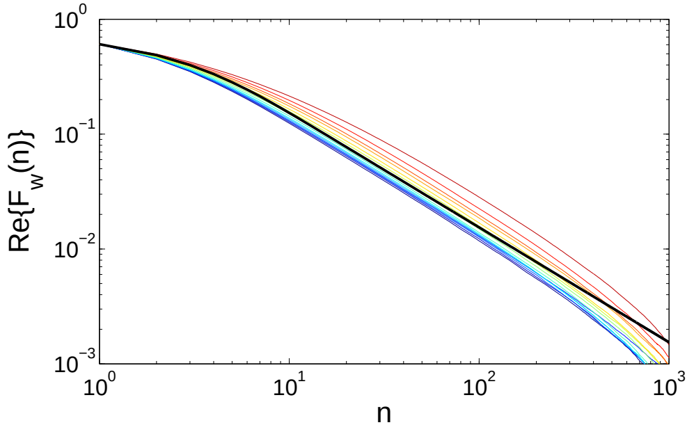
Figure 5.3: The real part of the ergodicity estimator, \text{Re}\{\hat{F}_\omega(n)\} (with \omega = 1/\sigma ), averaged over trajectories in each of 14 samples (thin lines). Color of thin curves changes from dark blue for the lowest packing fraction \phi to dark red for the highest one. Thick black line shows the mean value of this estimator for Brownian motion.
