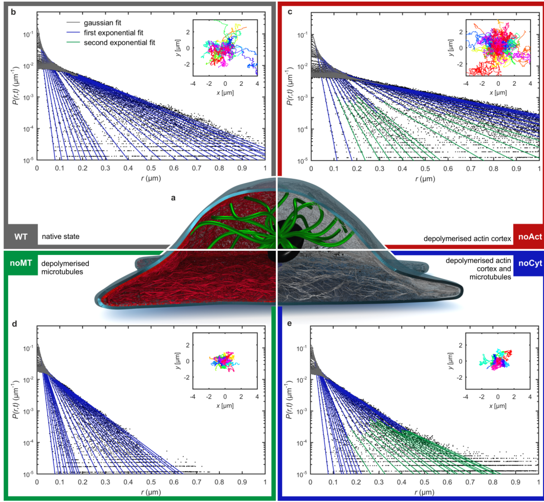
Figure 5.10: Probability density of increments of four different cytoskeleton states: (a) illustration of a cell with partly depolymerized cytoskeleton components (grey: membrane, black: nucleus, green: microtubule organizing center with microtubules, red: actin cortex; (b-e) probability densities of absolute magnitudes of one-dimensional projected increments, P(r, t) , for lag times t = \delta, 2\delta, \dots, 10\delta, 20\delta, \dots, 100\delta with the inverse frame rate \delta = 49 ms for four different cytoskeleton states: (b) wild type (WT), (c) depolymerized actin cortex (noAct), (d) depolymerized microtubules (noMT) and (e) both depolymerizations (noCyt); solid lines show the fit of a Gaussian function (grey) for small increments followed by an exponential fit (blue) and for some lag times in the actin deprived cases (noAct and noCyt) a second exponential fit (green); insets present the acquired trajectories of particle motion displayed in different colors for each trajectory.
