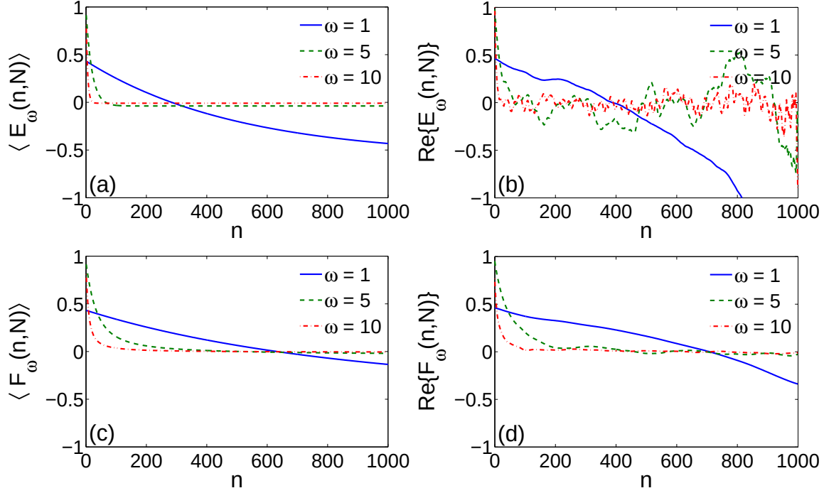
Figure 2.16: The mean mixing (a) and ergodicity (c) estimators as a function of n for a Brownian motion trajectory with N = 1000 and \sigma^2 = 0.04 . At \omega = 1 (solid line), both estimators are not small that may wrongly suggest nonmixing/nonergodic behavior. Increasing \omega , one can eliminate this false conclusion. The same conclusions can be made from the real part of the mixing (b) and ergodicity (d) estimators for a single Brownian motion trajectory with the same parameters.
