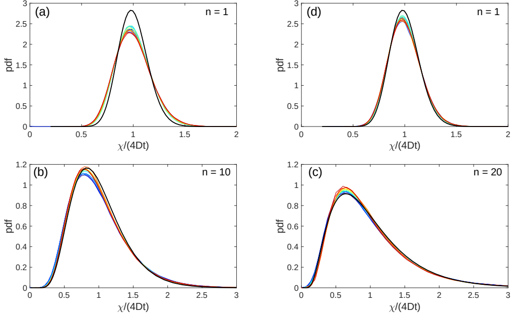
Figure 5.6: (a,b,c) Probability density functions of the rescaled TAMSD, \chi_{n,N}/(4Dt) , with N = 100 , t = n\delta , and n = 1 (a), n = 10 (b), and n = 20 (c), for 14 samples (thin lines), and the theoretical ones for Brownian motion (thick black line). Color of thin curves changes from dark blue for the lowest packing fraction \phi to dark red for the highest one. (d) Probability density functions of the rescaled TAMSD with N = 100 , t = n\delta , and n = 1 , for 14 reshuffled samples.
