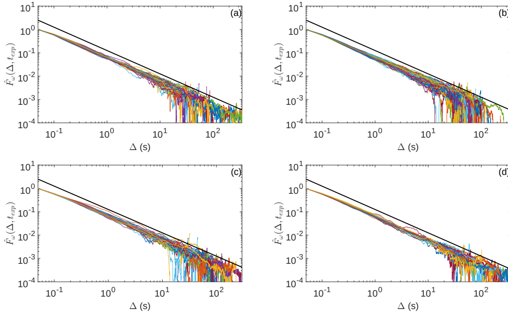
Figure 5.8: The ergodicity estimator \hat{F}_\omega(\Delta, t_{exp}) applied to each trajectory of duration t_{exp} as function of lag time \Delta(s) . The results are displayed for each cytoskeleton state: wild type (a) , depolymerized actin (b) , disrupted microtubules (c) , and deprived of both actin and microtubules (d) . Black lines indicates the \propto 1/\Delta decay of Brownian motion.
