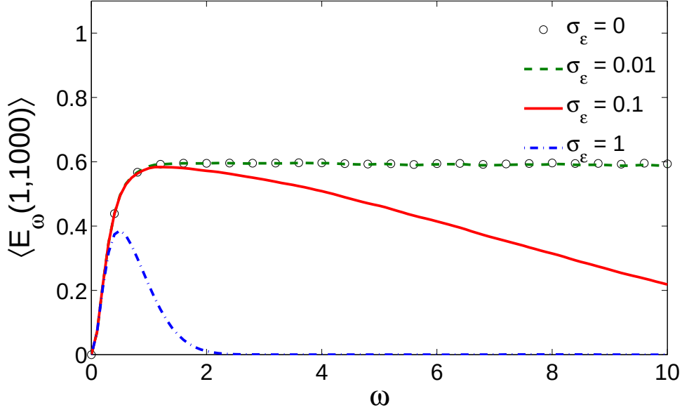
Figure 2.7: The mean mixing estimator \langle \hat{E}_\omega(1, 1000) \rangle as a function of \omega for CTRW with \alpha = 0.7 and \sigma = 1 , and four levels of white Gaussian noise: \sigma_\varepsilon = 0 (circles) and \sigma_\varepsilon = 0.01, 0.1, 1 (lines). Note that the plateau at 0.6 is smaller than the value \alpha = 0.7 expected from Eq. (2.51) because of the finite length effect ( N = 1000 ).
