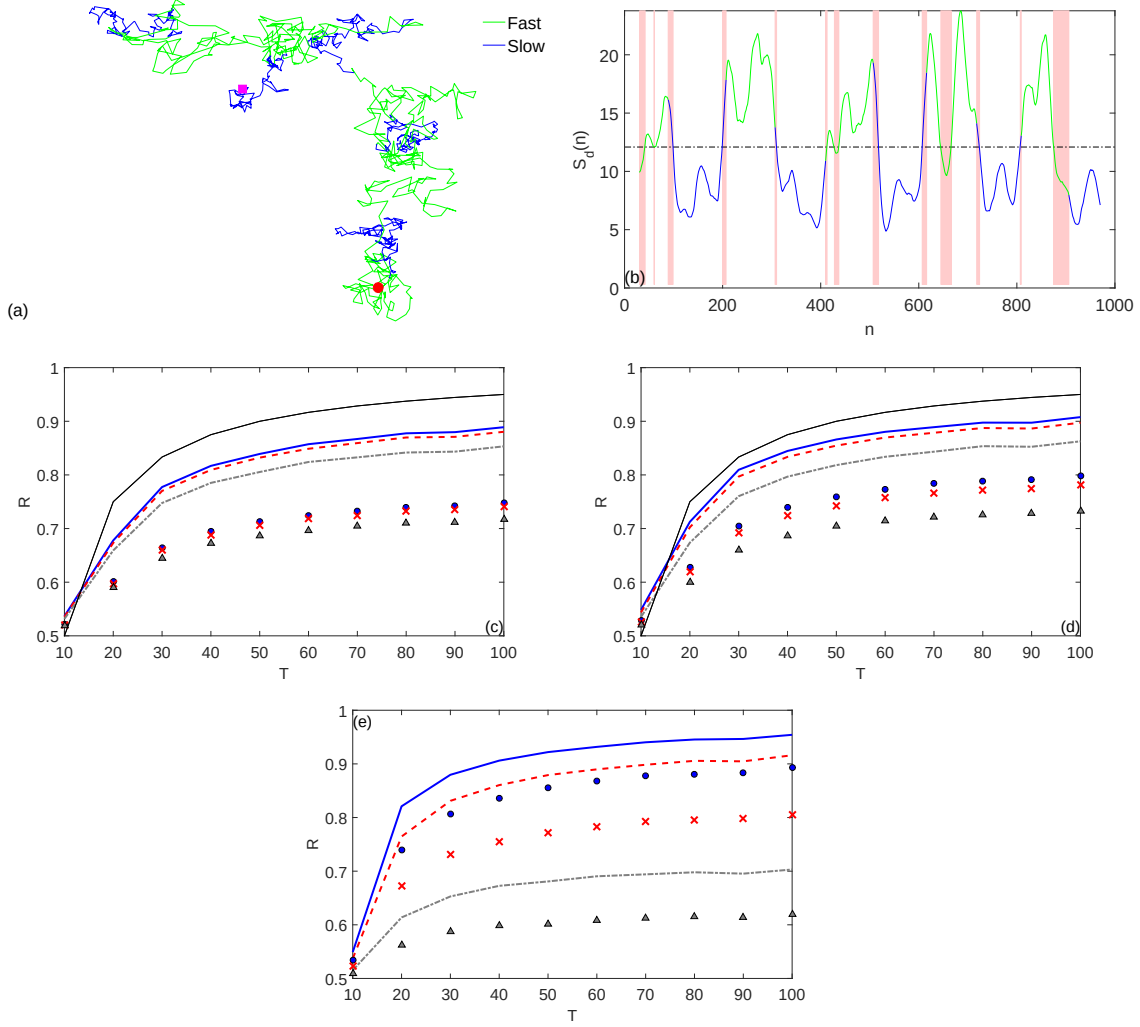
Figure 3.2: Model 1 (a) A single trajectory of planar Brownian motion alternating a “slow” phase ( D_1 = 1/2 , dark blue) and a “fast” phase ( D_2 = 2 , light green), of the mean phase duration T = 100 . Circle and square indicate the starting and ending points. (b) The weighted LCH diameter S_d(n) with the window size \Delta = 10 , applied to this trajectory. Pink shadow highlights the false classification zones. Dashed horizontal line shows the empirical mean S_d over that trajectory. (c,d,e) Recognition score R of the diameter-based discriminator S_d(n) (c), the volume-based discriminator S_v(n) (d), and the TA MSD-based discriminator (e) as a function of the mean phase duration T . Lines show the results for the case D_1 = 1/2 , D_2 = 2 with three noise levels \sigma_n : 0 (blue solid), 0.5\sigma (red dashed), and \sigma (gray dash-dotted) ( \sigma being the empirical standard deviation of increment calculated for each trajectory). Symbols correspond to the case D_1 = 1/2 , D_2 = 1 with the same levels of noise \sigma_n : 0 (circles), 0.5\sigma (crosses), and \sigma (triangles). Thin black solid line shows the hypothetical curve 1 - \Delta/(2T) for qualitative comparison.
