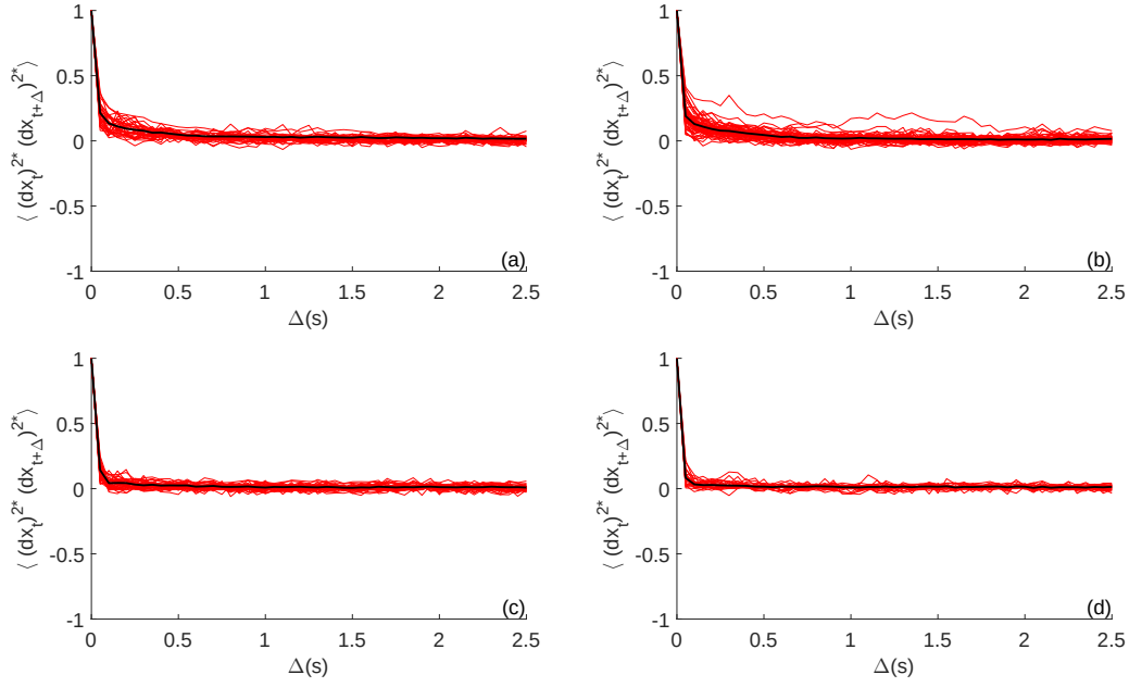
Figure 5.14: Time-averaged autocorrelation function of squared increments for different cytoskeleton states: wild type (a) , depolymerized microtubules (b) , depolymerized actin cortex (c) , and deprived of both actin and microtubules (d) , black lines correspond to the mean value obtained by averaging the autocorrelation for each trajectory in the respective cytoskeleton state, red lines marks the individual TA VACF.
