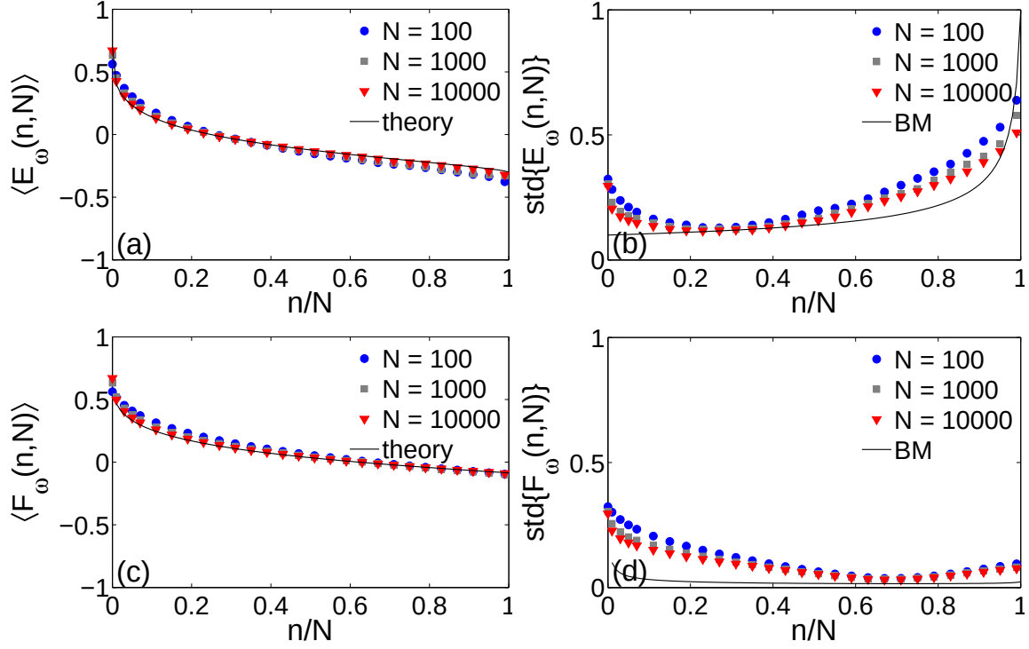
Figure 2.3: The mean ( a,c ) and standard deviation ( b,d ) of the mixing ( a,b ) and ergodicity ( c,d ) estimators at \omega = 10 as a function of n/N for CTRW with \alpha = 0.7 , \sigma = 1 , and three trajectory lengths N = 100, 1000, 10000 (symbols). For comparison, solid line shows the theoretical limits (2.51, 2.52) of the mean estimators for CTRW and the standard deviation for Brownian motion (given by square roots of Eqs. (2.17, 2.18) with N = 100 ).
