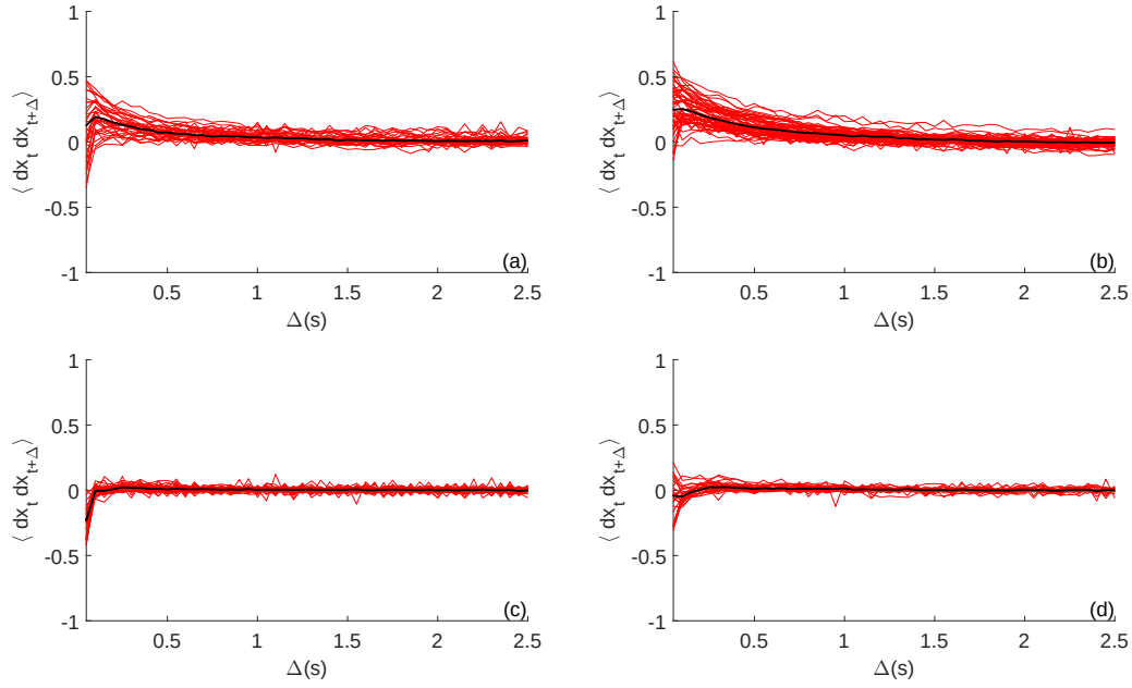
Figure 5.12: Time-averaged velocity auto-correlation function for different cytoskeleton states: Wild Type (a) , depolymerised microtubules (b) , depolymerised actin cortex (c) , and deprived of both actin and microtubules (d) , black lines correspond to the mean value obtained by averaging the velocity auto-correlations for each trajectory in the respective cytoskeleton state, red lines marks the individual TA VACF.
