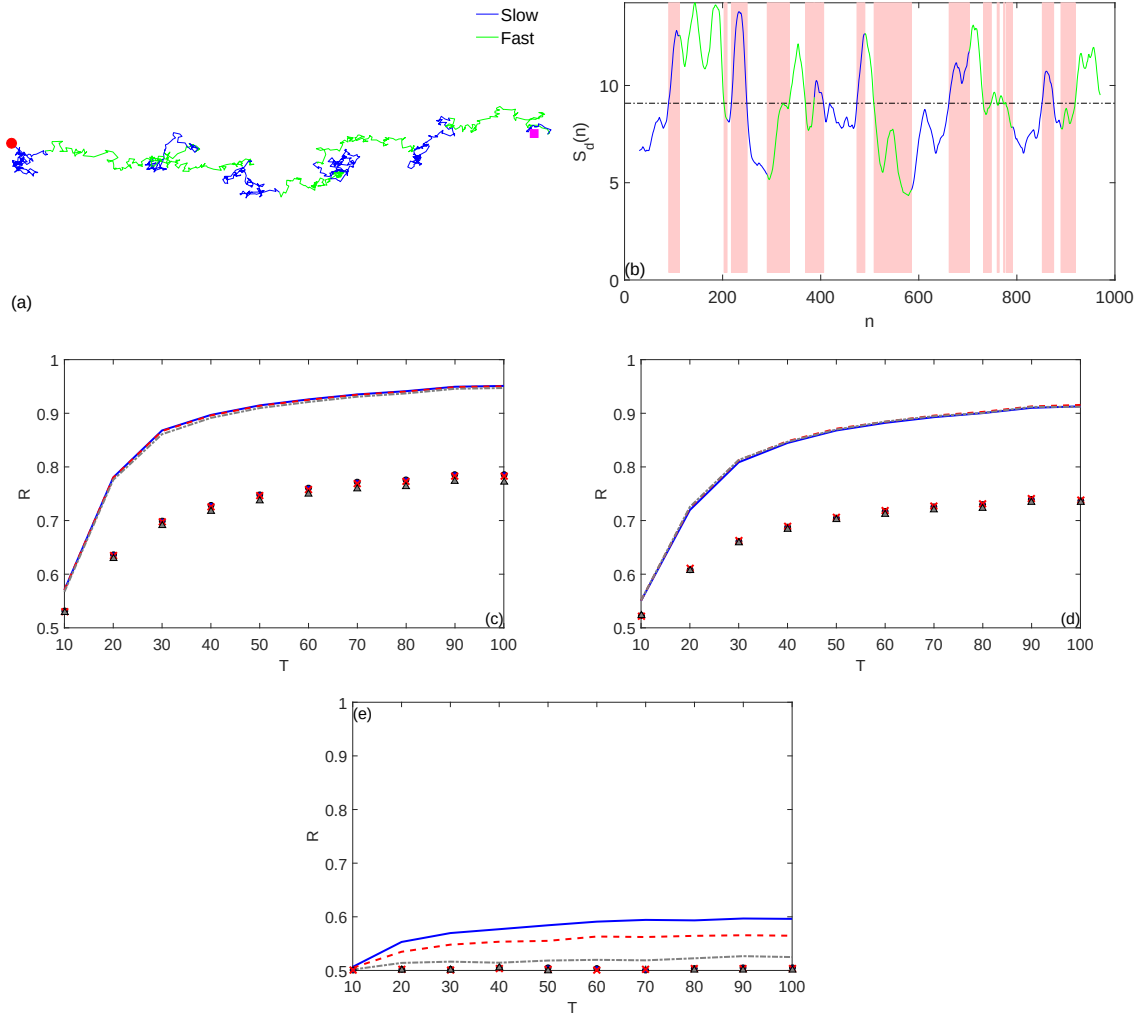
Figure 3.4: Model 2 (a) A single trajectory of an intermittent process alternating a “slow” phase of planar Brownian motion without drift (dark blue) and a “fast” phase with drift ( \mu = 0.5 , light green), of the mean phase duration T = 100 (both phases with D = 1/2 ). Circle and square indicate the starting and ending points. (b) The weighted LCH diameter S_d(n) with the window size \Delta = 10 applied to this trajectory. Pink shadow highlights the false classification zones. Dashed horizontal line shows the empirical mean S_d over that trajectory. (c,d,e) Recognition score R of the diameter-based discriminator S_d(n) (c), the volume-based discriminator S_v(n) (d), and the TA MSD-based discriminator (e) as a function of the mean phase duration T . Lines show the results for the case \mu = 0.5 with three noise levels \sigma_n : 0 (blue solid), 0.5\sigma (red dashed), and \sigma (gray dash-dotted) ( \sigma being the empirical standard deviation of increment calculated for each trajectory). Symbols correspond to the case \mu = 0.1 with the same levels of noise \sigma_n : 0 (circles), 0.5\sigma (crosses), and \sigma (triangles).
