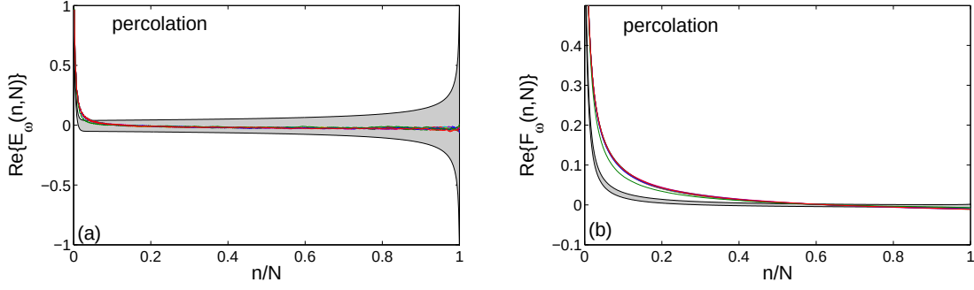
Figure 2.4: The mean mixing (a) and ergodicity (b) estimators at \omega = 1 as a function of n for one coordinate X(n) of two-dimensional random walk of length N = 500 on a critical percolating cluster on a 1000 \times 1000 square lattice, with the lattice step \sigma = 1 . Each curve presents the mean computed by averaging over 1000 trajectories generated on one cluster. The curves obtained for ten random clusters are almost identical. For comparison, light gray shadowed region delimits the mean plus and minus the standard deviation of each estimator computed for Brownian motion according to Eqs. (2.11, 2.12, 2.17, 2.18).
