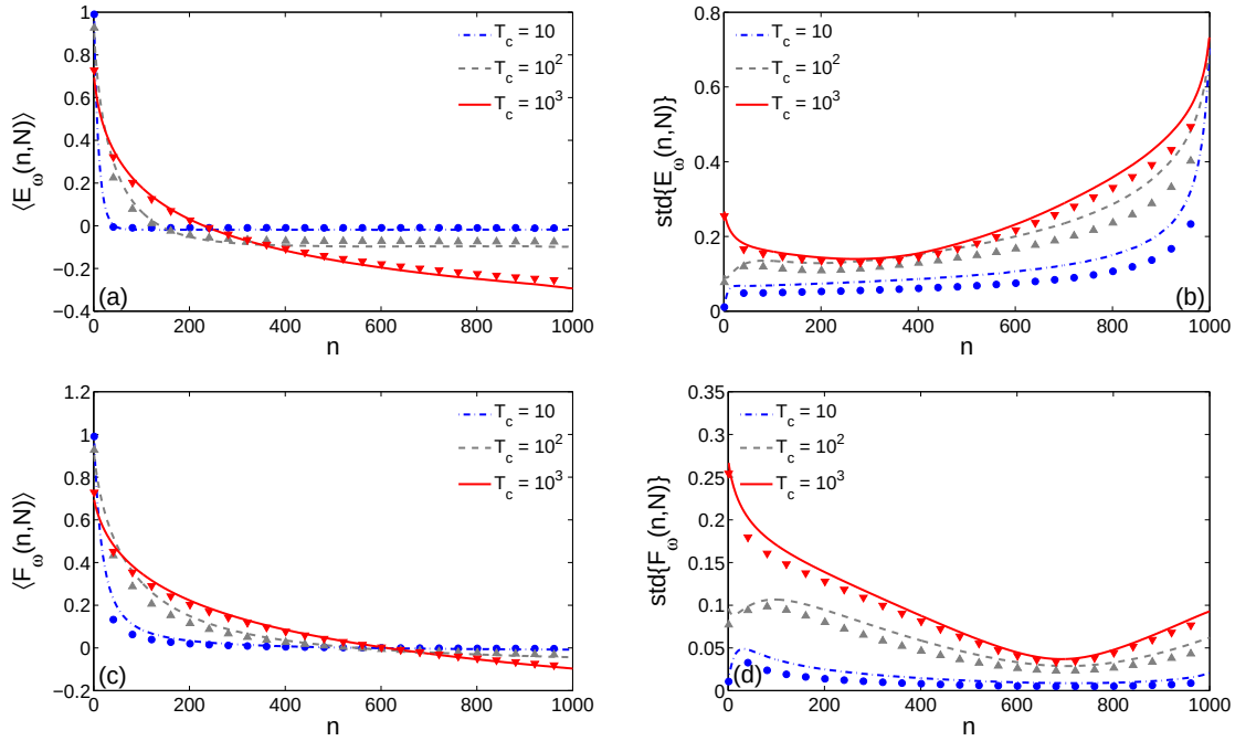
Figure 2.5: The mean ( a,c ) and standard deviation ( b,d ) of the mixing ( a,b ) and ergodicity ( c,d ) estimators at \omega = 1 (lines) and \omega = 10 (symbols) for CTRW with N = 1000 , \alpha = 0.7 , \sigma = 1 , \delta_s = 1 , and exponential cut-off at T_c = 10, 10^2, 10^3 .
