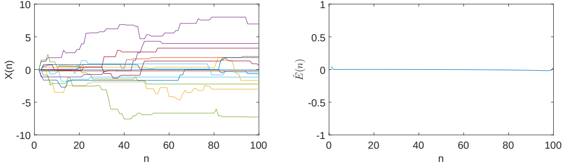
Figure 2.1: Left. Illustration of 15 one-dimensional trajectories of non ergodic CTRW with Gaussian jumps and power law waiting times \phi(t) \propto 1/t^{1-\alpha} where the exponent is \alpha = 0.7 . Right. The corresponding mixing estimator averaged over 10^5 realizations of the CTRW with the same parameters.
