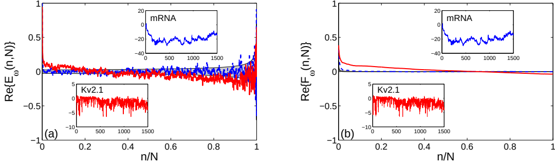
Figure 2.11: The real part of the mixing (a) and ergodicity (b) estimators at \omega = 2 as a function of n for two experimental trajectories of around N = 1500 points: the motion of mRNA molecule inside live E. coli cell [106] and Kv2.1 potassium channel anomalous dynamics in the plasma membrane [280]. Both trajectories (shown in insets) were normalized by the empirical standard deviation of their increments. Light gray shadowed region delimits the typical range of fluctuations of estimators for Brownian motion, i.e., the mean plus and minus the standard deviation.
