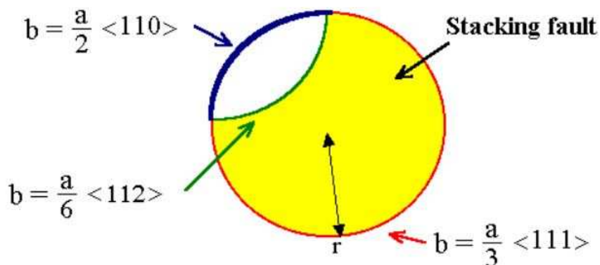
Figure 1.15 – Schematic representation of an unfaulting process involving a Frank, perfect and Shockley dislocations (Foll, 2018).
