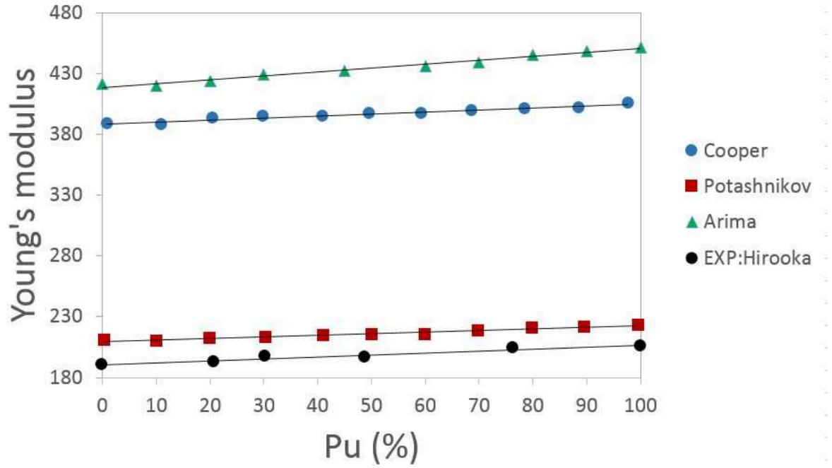
Figure 3.15 – Evolution of monocrystal Young's modulus as a function of the plutonium content calculated with Arima, Potashnikov, and Cooper potentials and are compared with the experimental values in (Hirooka & Kato, 2018)
