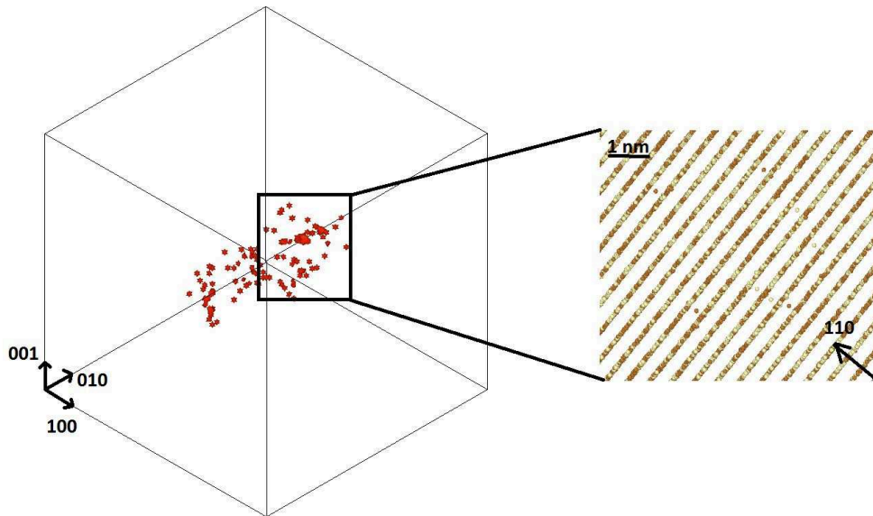
Figure 4.5 – Snapshot of the defect analysis at the end of the cascade initiated with 75 keV PKA for Potashnikov potentials for 50% Pu content. The red zone marked the regions where structure departs from perfect fluorite structure. The insets represent close-up visualisation of the atoms in the main disordered region.
