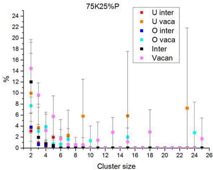
Figure C.2 – Distribution of point defects in cluster (interstitial and vacancy) as a function of their size for Potashnikov potentials calculated from 75 keV PKA cascade and 25% Pu
