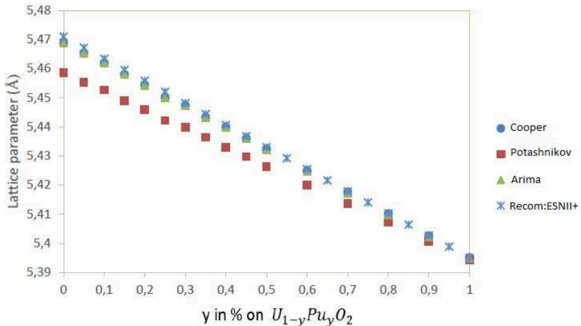
Figure 3.3 – Evolution of the lattice parameter as a function of Pu content at 300 K.
