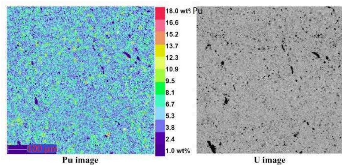
Figure 1.4 – X-ray Mappings of a newly fabricated MOX pellet (KAERI, 2009). The colour level corresponds to wt % of \text{PuO}_2
