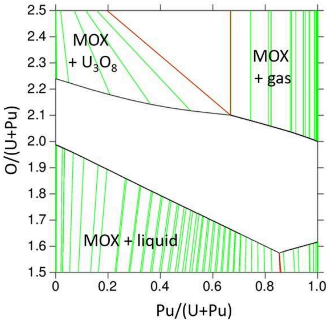
Figure A.2 – Magnified snapshot of O-Pu-U phase diagram as a function of composition and Pu content calculated at 1500 K (Guéneau et al., 2011)
