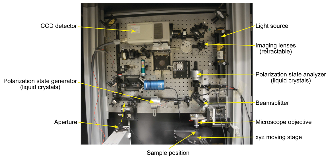
Figure 3.3 – Angle-resolved Mueller matrix polarimetry set-up.
