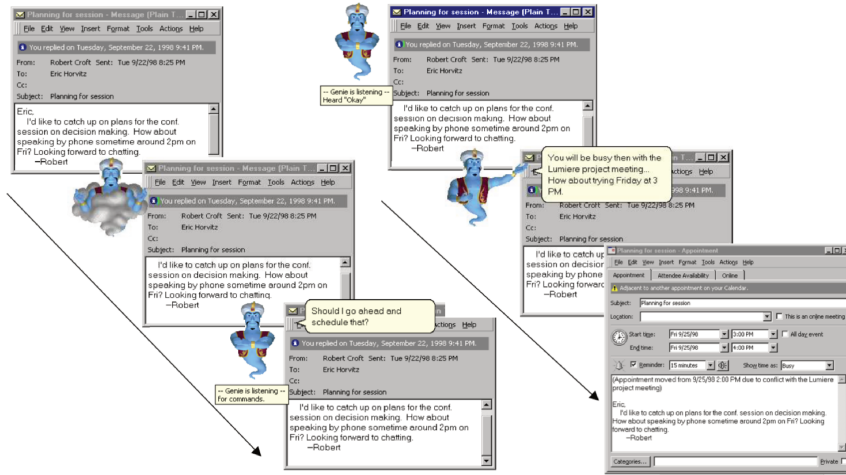
Figure 61: Lookout: procedures that harness probability and utility guide Lookout's actions to assist users with accessing their calendar and composing appointments, based on a background analysis of email being reviewed. Taken from [101].
