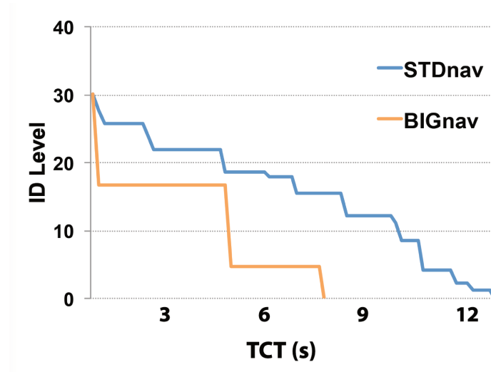
Figure 40: Time plot of the decrease in ID in the STDnav and BIGnav conditions, for two trials with the same other conditions.
