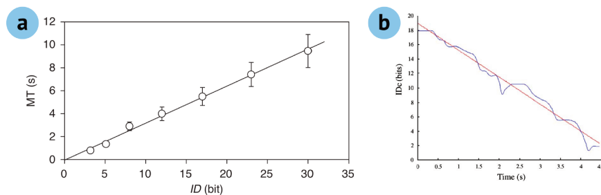
Figure 27: (a) Fitts' law assessed over a selection of IDs ranging beyond 10 bits and (b) Evolution of the current level of ID over a representative target-reaching movement. Taken from [86].
