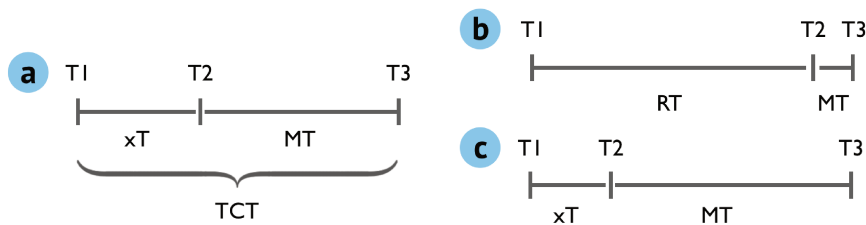
Figure 16: (a) Three time marks in a stimulus-response (S-R) paradigm: S-onset time T_1 , R-onset time T_2 , and R-termination time T_3 . Task completion time (TCT) = T_3 - T_1 , movement time MT = T_3 - T_2 and xT = T_2 - T_1 , which describes the psychological processes (reaction, visual search, decision, etc.) before movement. (b) xT = RT choice reaction time in Hick's experiment [98], while (c) xT involves different mental tasks in the studies listed in Table 1.
