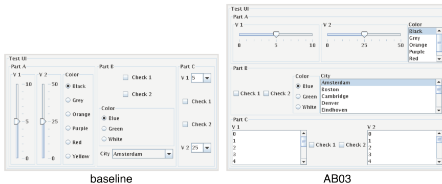
Figure 49: The baseline interface is shown in comparison to interfaces generated automatically by SUPPLE based on two participants' preferences. Participant AB03 preferred lists to combo boxes but preferred them to be short. Taken from [73].
