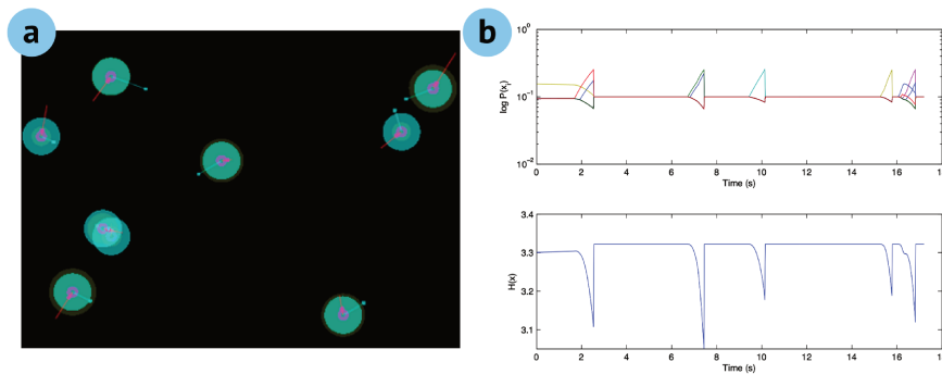
Figure 23: (a) The prototype of [217]. Each agent is shown as a circle with radius proportional to selection probability. The velocity of the objects is shown as an aid to users. (b) Probability time series for 10 objects with a number of correct selection events. Entropy is shown as the blue line below. Figures adapted from [217].
