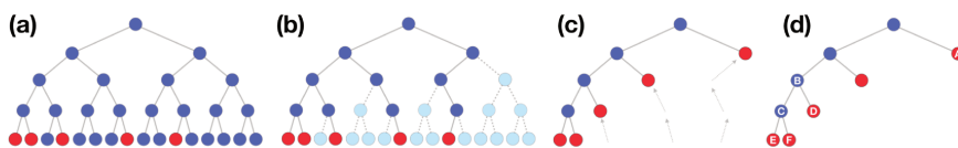
Figure 54: BIGFileFast with a binary tree: (a) Find the n = 5 most probable targets (red nodes); (b) Find their parents up to the root (dark blue nodes) and prune all the non-parent nodes (light blue nodes); (c) recursively replace the parent of a node by its child if it is the only child; (d) if the expected information gain of (A,B) is greater than that of (A,C) , prune branch C and move directly to the next branch (A,D) , skipping E and F.
