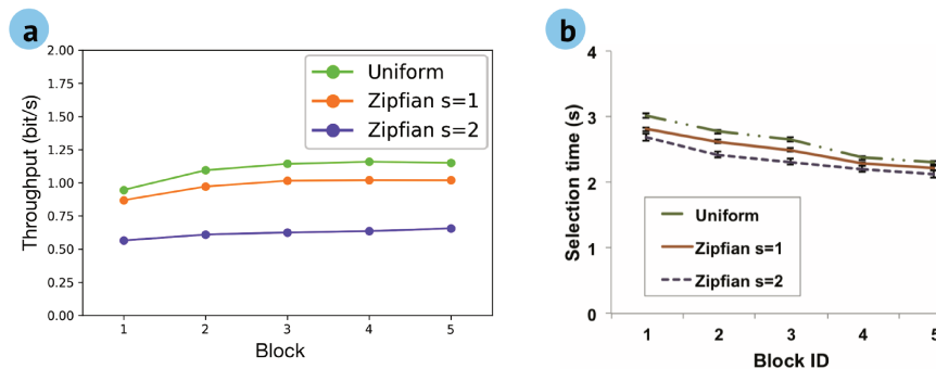
Figure 74: (a) Information-theoretic notion of throughput and (b) selection time (taken from [133]) for 3 distributions across 5 blocks.
