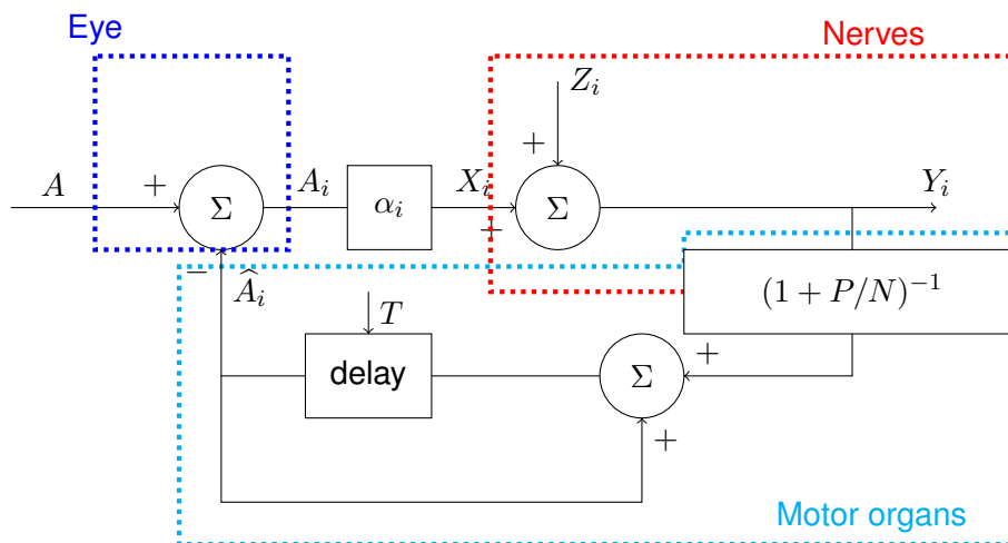
Figure 6.5: Possible implementation of how human perform the aiming task: functions and potential organ groups who can perform these functions.
