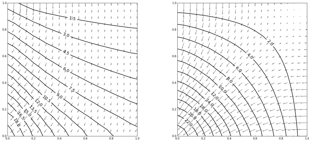
(a) A_{1111}^*(m_1, m_2, 0.5) with A_{1111} = 25.58
