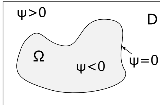
Figure 1.2: Description of a shape with a level-set function \psi
