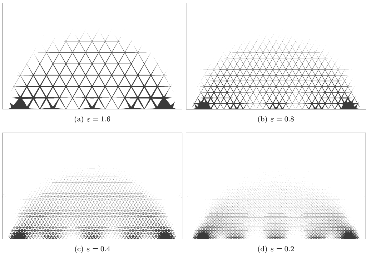
Figure 3.35: Projection of a radial density \theta over a classical honeycomb composite, for several sizes of cell \varepsilon
