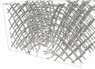
(h) \Omega_{12} \cup \Omega_{23}
