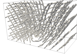
(i) \Omega_{13} \cup \Omega_{23}
