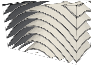
(a) \Omega_1 = \Omega_{1,\varphi,0.2}(m_{reg})
