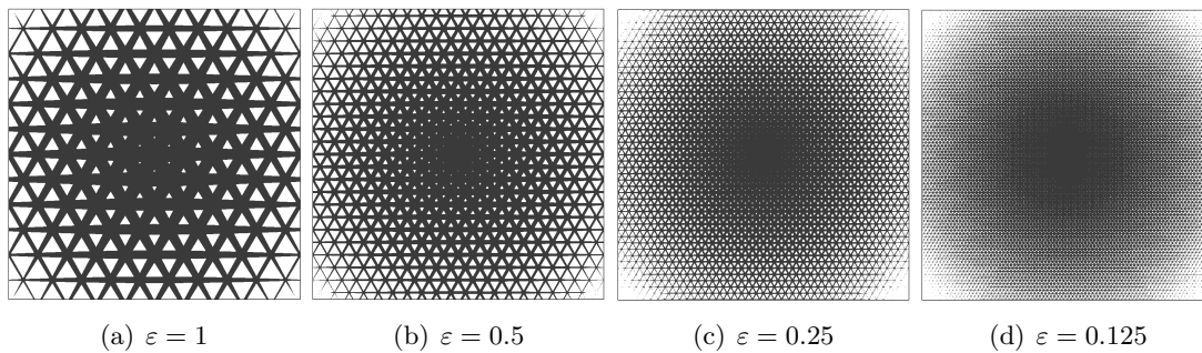
Figure 3.32: Projection of a radial density \theta over a reinforced honeycomb composite, for several sizes of cell \epsilon
