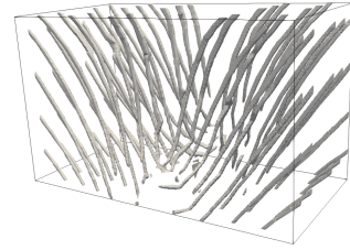
(f) \Omega_{23} = \Omega_2 \cap \Omega_3
