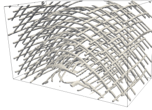
(g) \Omega_{12} \cup \Omega_{13}
