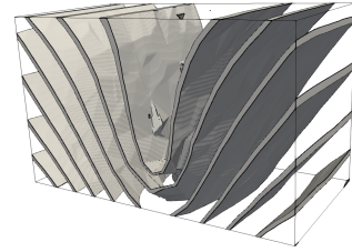
(c) \Omega_3 = \Omega_{3,\varphi,0.2}(m_{reg})
