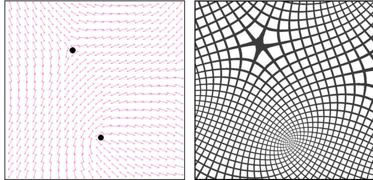
(a) Orientation vector field featuring two singularities (black points) (b) Projection of a regular square grid
