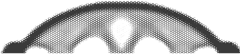
(c) \varepsilon = 1
