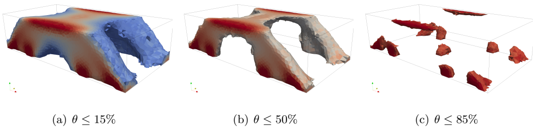
Figure 3.16: Threshold of the domain according to the optimized density \theta for the second test case, in the multiple loads compliance minimization problem
