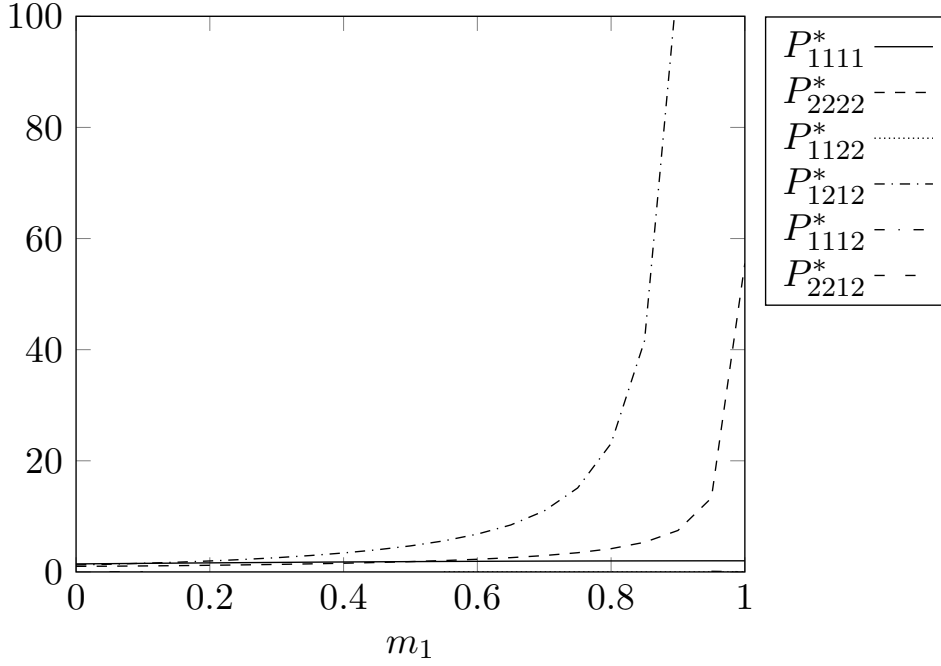
Figure 4.31: P^*(m_1, 0.5)
