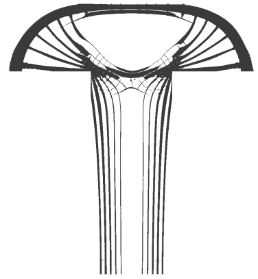
(c) \Omega_\varepsilon(m)
