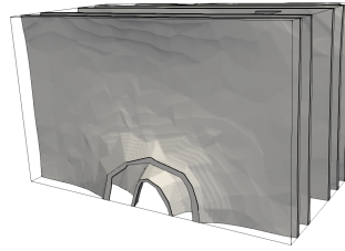
(b) \Omega_2 = \Omega_{2,\varphi,0.2}(m_{reg})
