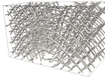
(j) \Omega_{12} \cup \Omega_{13} \cup \Omega_{23}
