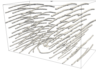
(e) \Omega_{13} = \Omega_1 \cap \Omega_3
