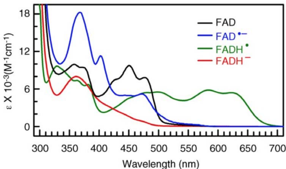
Figure 3.3: Spectra of four different redox states of FAD. 83 FAD here refers to oxidized FAD. The \text{FADH}_2 spectrum, not included here, slightly resembles that of \text{FADH}^- with a more gradual incline and lower extinction in the blue region. The FAD and \text{FAD}^{\bullet-} spectra are from mosquito cryptochrome AgCRY1. The \text{FADH}^{\bullet} and \text{FADH}^- spectra are from E. coli photolyase.
