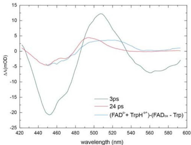
Figure 7.2: DADS of glucose oxidase as reported by Lukacs et al. 100 The 24 ps phase has a spectra similar to that of the 3 ps phase in TrmFO C51A (Fig. 6.11 (a)), with an intense induced absorption peak \sim 490 nm. The 24 ps phase was modelled with the TrpH + spectrum. This model, as claimed by the authors, is "not definitive".
