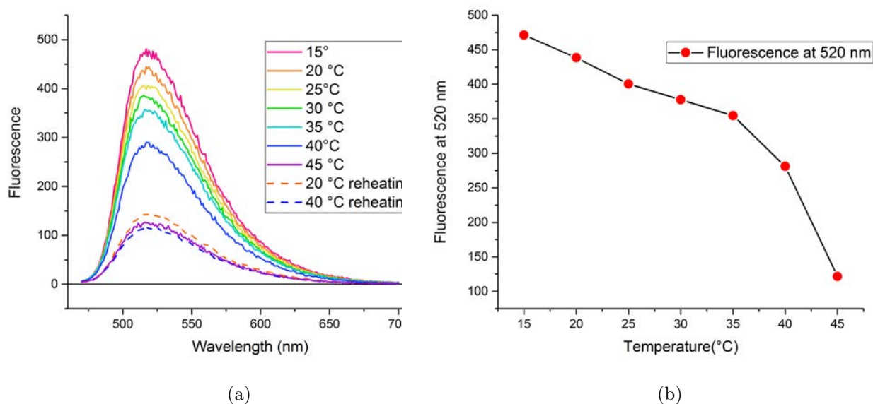
Figure 6.21: (a) Evolution of steady state fluorescence of TrmFO C51A/Y343F with temperature. Spectra are recorded with polarizers in the excitation and emission beam set at magic angle to remove any polarization effects. The change appears irreversible: when lowering the temperature again the fluorescence remained low (20°C and 40°C reheating). (b) Maximum fluorescence of TrmFO C51A/Y343F at 520 nm as a function of temperature.
