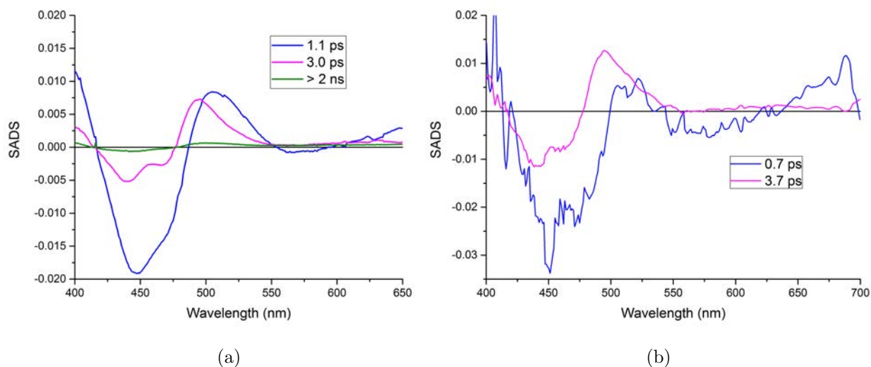
Figure 6.12: (a) Species Associated Difference Spectra (SADS) corresponding to the DAS of Fig. 6.11(a). These spectra correspond to a model in which the DAS are interpreted in terms of a model A \rightarrow B \rightarrow C . The difference spectrum A corresponds to the initially formed state, here FAD^* \text{ minus } FAD_{ox} ; B an intermediate state formed in 1.1 ps and C a final state formed in 3.0 ps. As the final spectrum of C is very small, the spectrum of B (3.0 ps SADS) is very similar to the 3.0 ps DAS discussed in the text and assigned to FAD^- \text{ TyrOH}^+ \text{ minus } FAD_{ox} . The 1.1 ps SADS contains bleaching features in the FAD_{ox} absorption region and further negative absorption above 550 nm which is assigned to stimulated emission. Furthermore, the induced absorption features around 400 nm and 520 nm are assigned to excited state absorption. The larger bleaching in the 1.1 ps SADS with respect to the 3.0 ps SADS indicates that the 3.0 ps phase corresponds to only part of the initially excited FAD, presumably because a substantial part of the product state formed in 1.1 ps recombines to the ground state on a timescale faster than its formation. Precise quantification of the yield of the product state is complicated by the compensating excited state absorption (1.1 ps SADS) and FAD^- (3.0 ps SADS, see Fig. 6.13) bands superimposing the ground state absorption region. We estimate this yield at roughly 20-40% C. (b) DAS of TrmFO C51S. The fast 0.7 ps phase has poorer signal to noise than the 3 ps phase (see Section 5). Only the fast components of decay have been shown in this figure.
