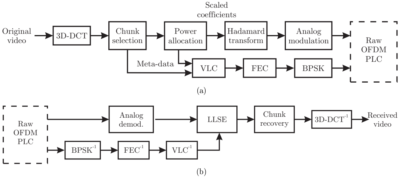
Figure 2.3: SoftCast transmitter (a) and receiver (b)
