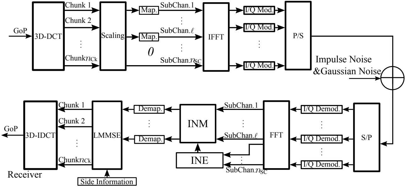
Figure 5.2: Modified SoftCast-based LVC (with discarded chunks), transmission, and decoding architecture (with impulse noise correction)
