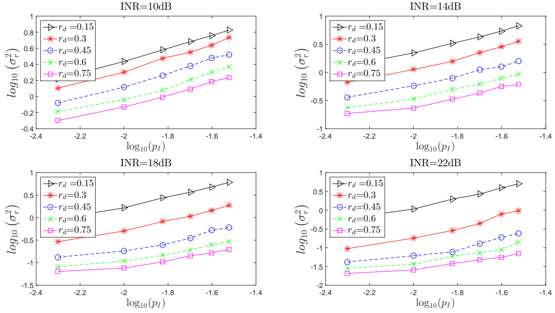
Figure 5.7: \log_{10}(\sigma_r^2) as a function of \log_{10}(p_I) for different values of the INR in dB and of r_d
