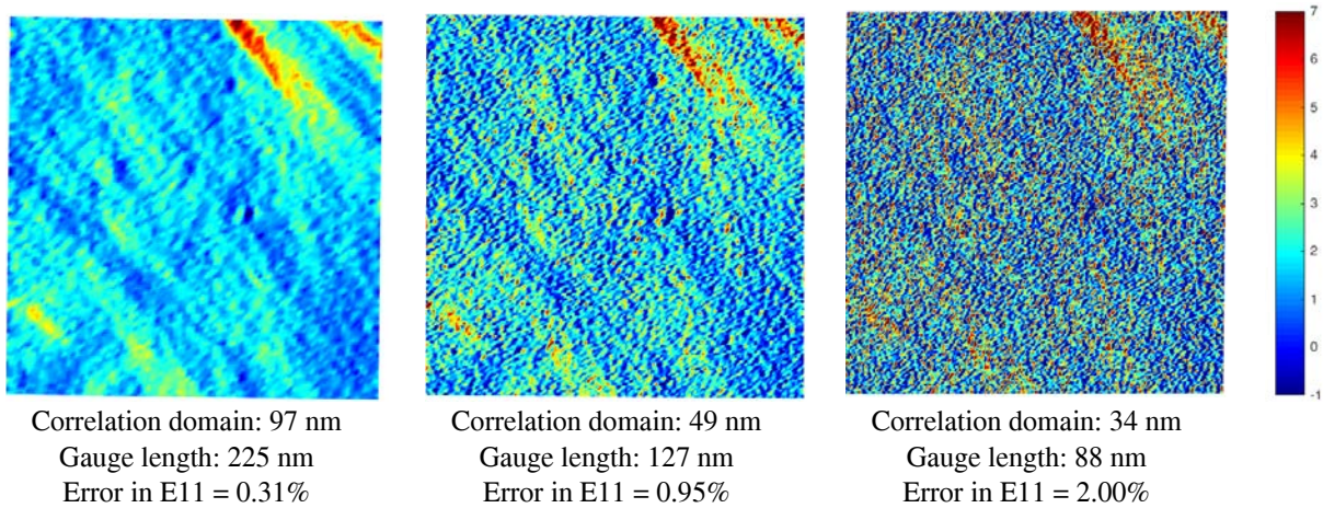
Figure 4.9: Effect of correlation domain size on the computed axial plastic strain field in a 10 \times 10 \mu m^2 area.
