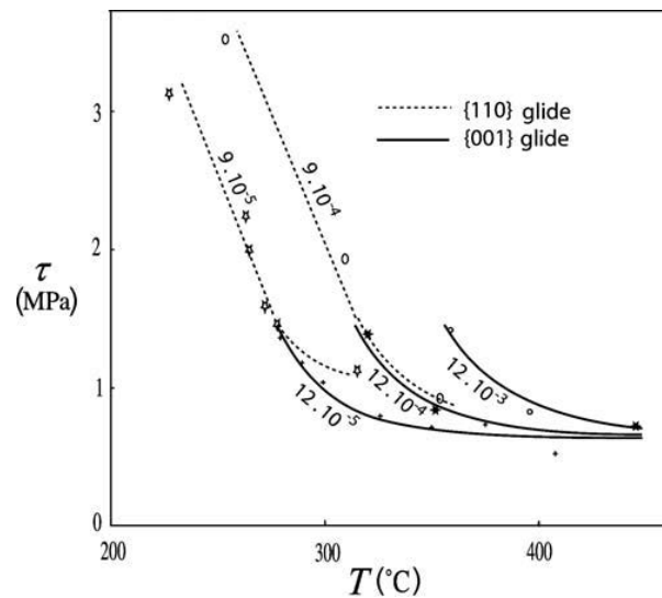
Figure 4.105: CRSS for the activation of non-octahedral slip in \{110\} and \{001\} planes in Al [21].
