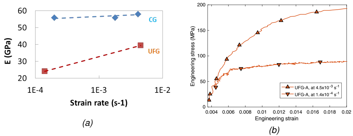
Figure 3.19: (a) Young's modulus as a function of strain rate at 200^\circ C and (b) a zoom of engineering stress-strain plot at 200^\circ C for UFG material.
