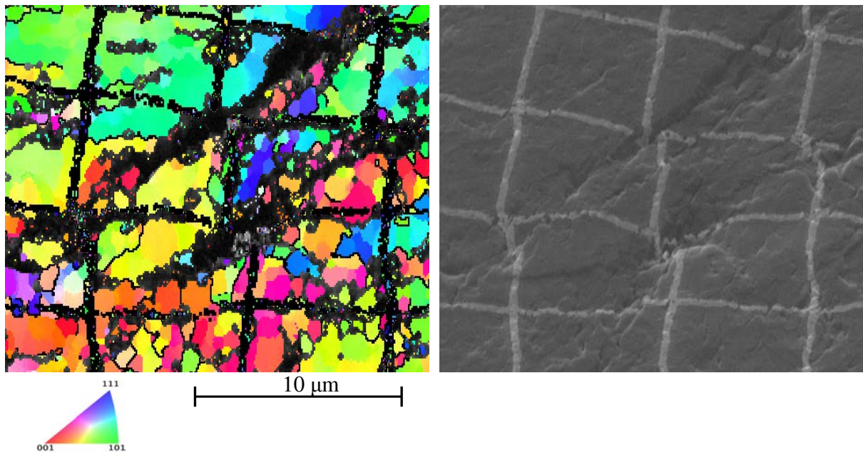
Figure 4.89: Post fracture IPF-Y map of the UFG material strained until 49.8% at 1.4 \times 10^{-4} \text{ s}^{-1} at 200° C
