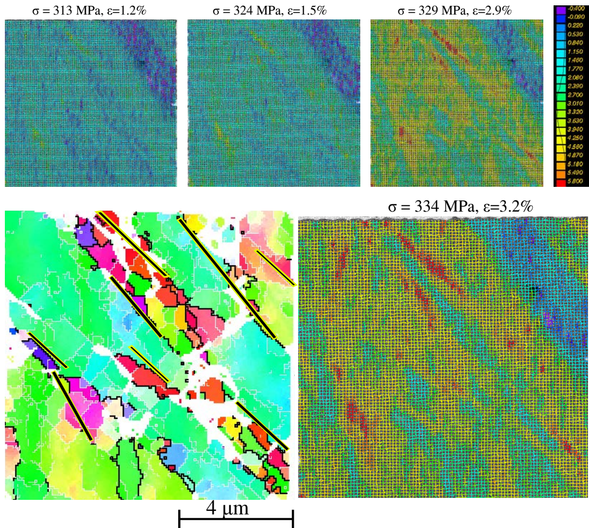
Figure 4.34: Micro-scale strain fields of 10 \times 10 \mu\text{m} area for UFG material tested at 5.8 \times 10^{-5} \text{ s}^{-1} at RT
