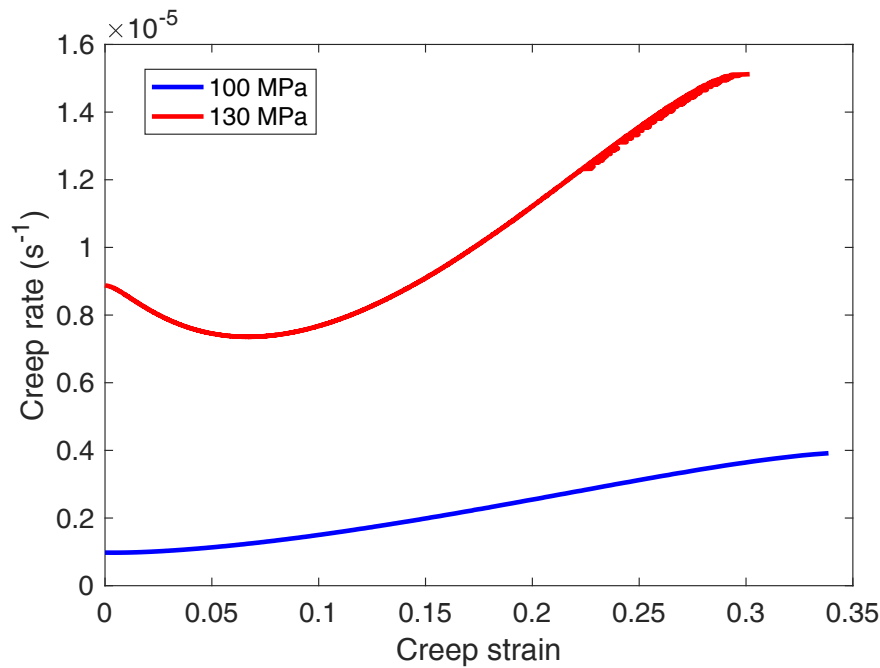
Figure 3.A.3: Evolution of creep rate with strain at 200°C
