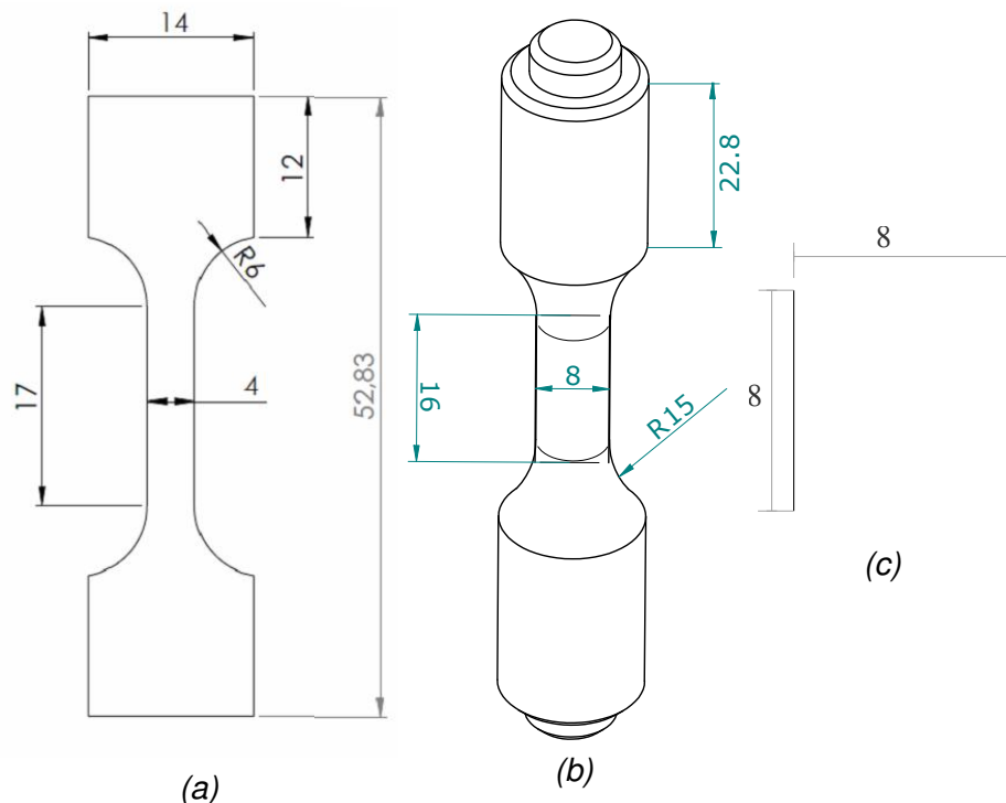
Figure 2.21: Specimen geometries for experimentation: (a) Flat dog-bone shaped specimen for tensile testing, (b) cylindrical specimens for fatigue and (c) cylindrical specimens for relaxation tests in compression (All the units are in mm).
