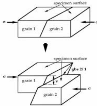
Figure 1.27: Out-of-plane component of GBS [71]
