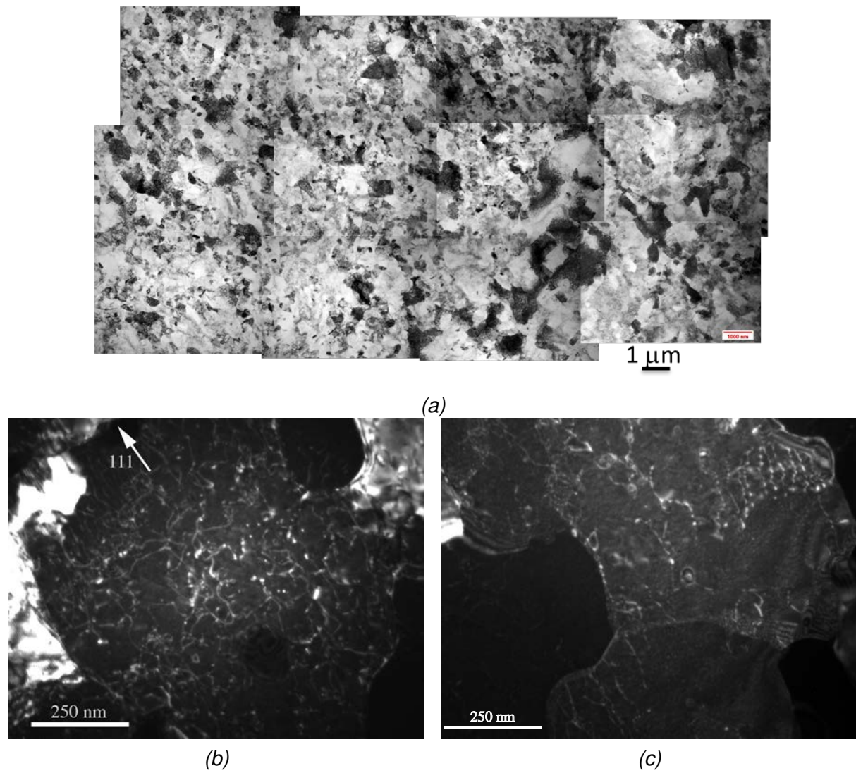
Figure 6.12: TEM observations of UFG LCF samples at \varepsilon_p = \pm 8 \times 10^{-3}
