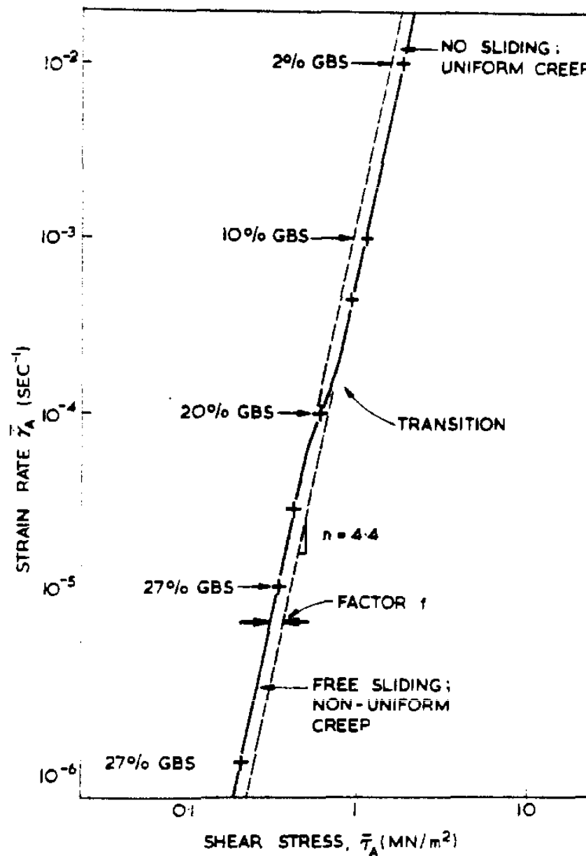
Figure 5.6: Creep rate evolution with applied stress predicted by Crossman & Ashby [3].
