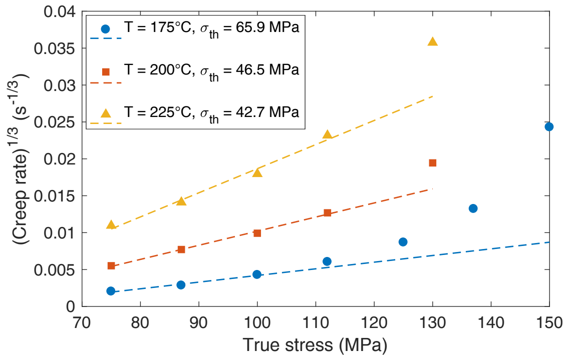
Figure 3.A.6: Plot of \dot{\epsilon}^{1/n} vs. \sigma to calculate threshold stress at n = 3 .
