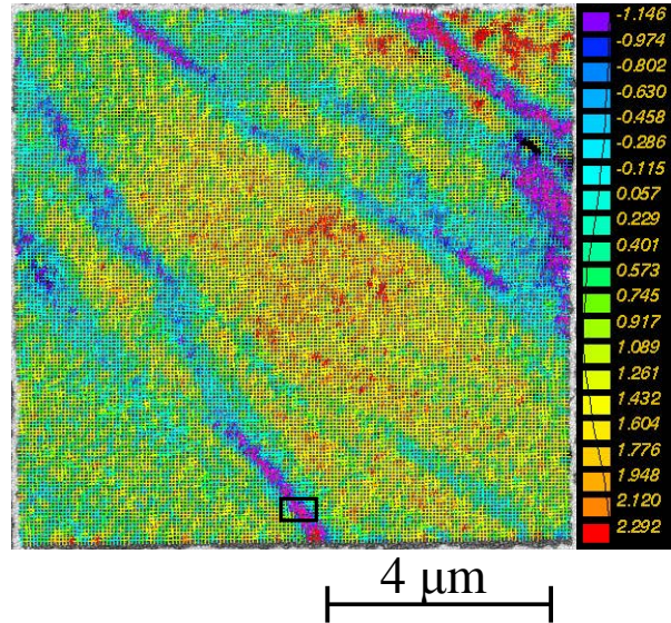
Figure 4.31: Rigid body rotation map (in degrees) at \sigma = 334 MPa, \epsilon = 2.4\% in UFG-A material tested at 5.8 \times 10^{-5} \text{ s}^{-1} at RT
