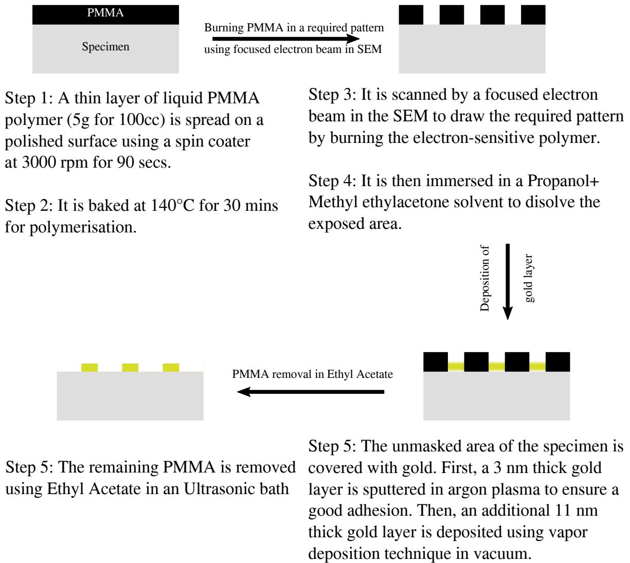
Figure 4.1: Procedure for patterning by electron beam lithography.
