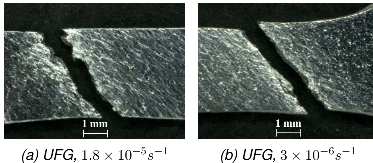
Figure 3.14: Optical images of the fractured samples at 100^\circ \text{C}
