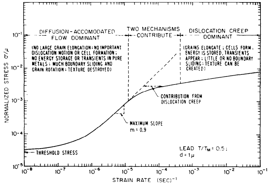
Figure 5.3: Evolution of the flow stress of a polycrystal with strain rate predicted by Ashby and Verral's model [2].
