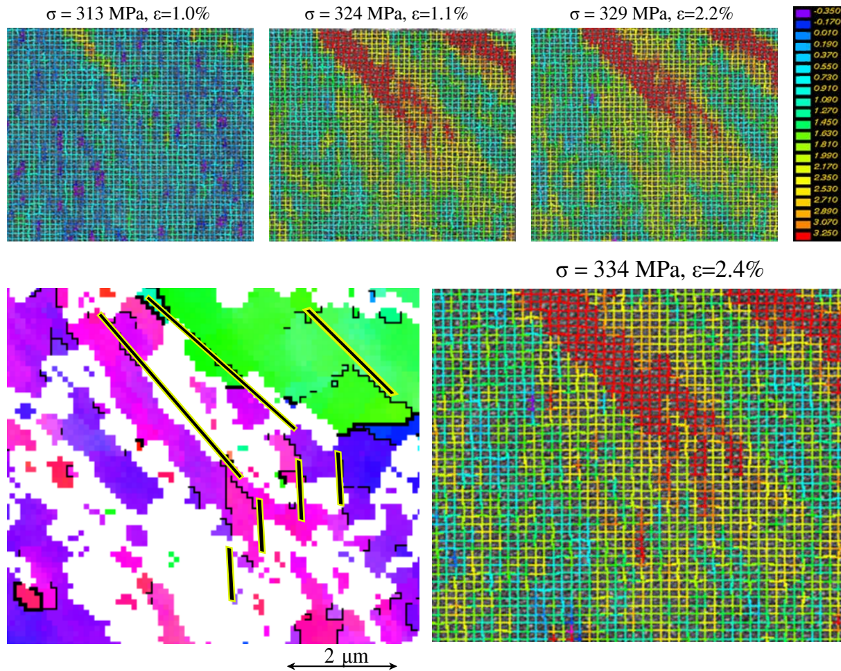
Figure 4.33: Micro-scale strain fields of 5 \times 4.5 \mu\text{m} area for UFG material at 5.8 \times 10^{-5} \text{ s}^{-1} , RT
