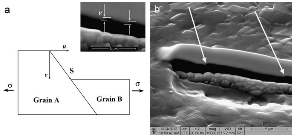
Figure 1.30: Vertical offsets (steps) on grain boundaries produced by GBS on a FIB cross section in UFG Al after tension [73].
