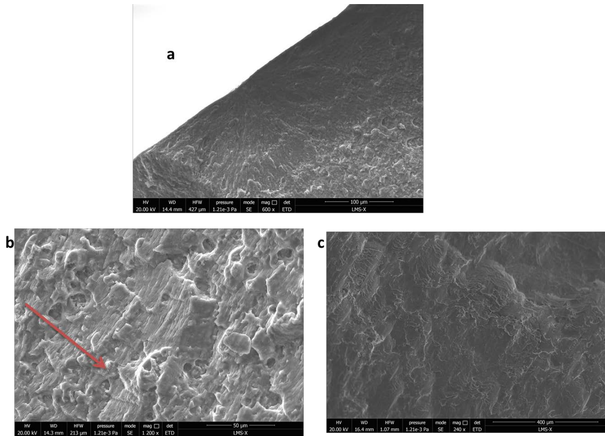
Figure 6.19: Fracture surface of a UFG sample submitted to a stress-controlled push-pull test at \pm 200\text{ MPa} ( N_f = 45438 cycles). a) one of the semi-circular cracks initiated from the surface, b) striation-like features (the arrow indicates the crack growth direction) and c) heavily mated slanted zone
