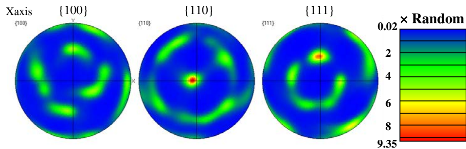
Figure 2.34: Pole figures of UFG-B material.
