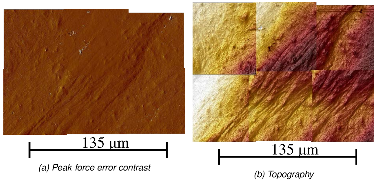
Figure 4.48: AFM imaging in "peak force tapping" mode of as-ECAP UFG specimen deformed by 4.6% at 5.8 \times 10^{-5} \text{ s}^{-1} at RT
