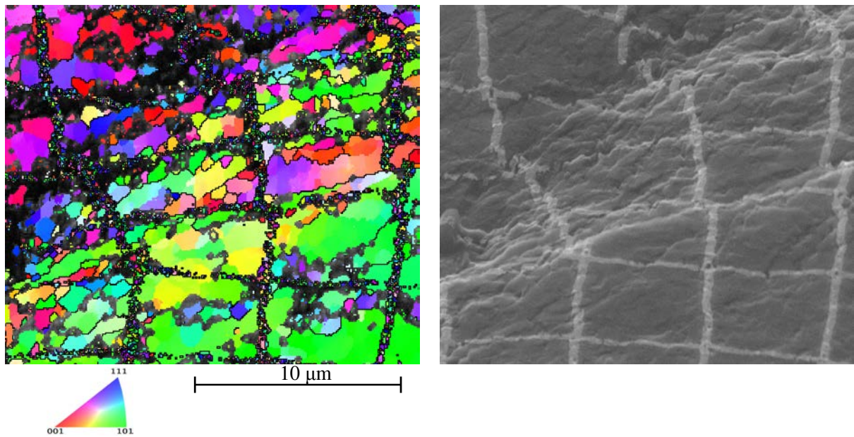
Figure 4.90: Post fracture IPF-Y map of the UFG material strained until 49.8% at 1.4 \times 10^{-4} \text{ s}^{-1} at 200° C
