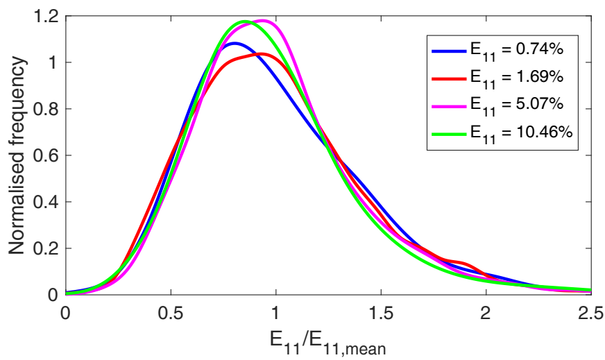
Figure 4.16: Histograms of normalised axial strain at different steps in CG material strained at 5.8 \times 10^{-5} \text{ s}^{-1} at RT
