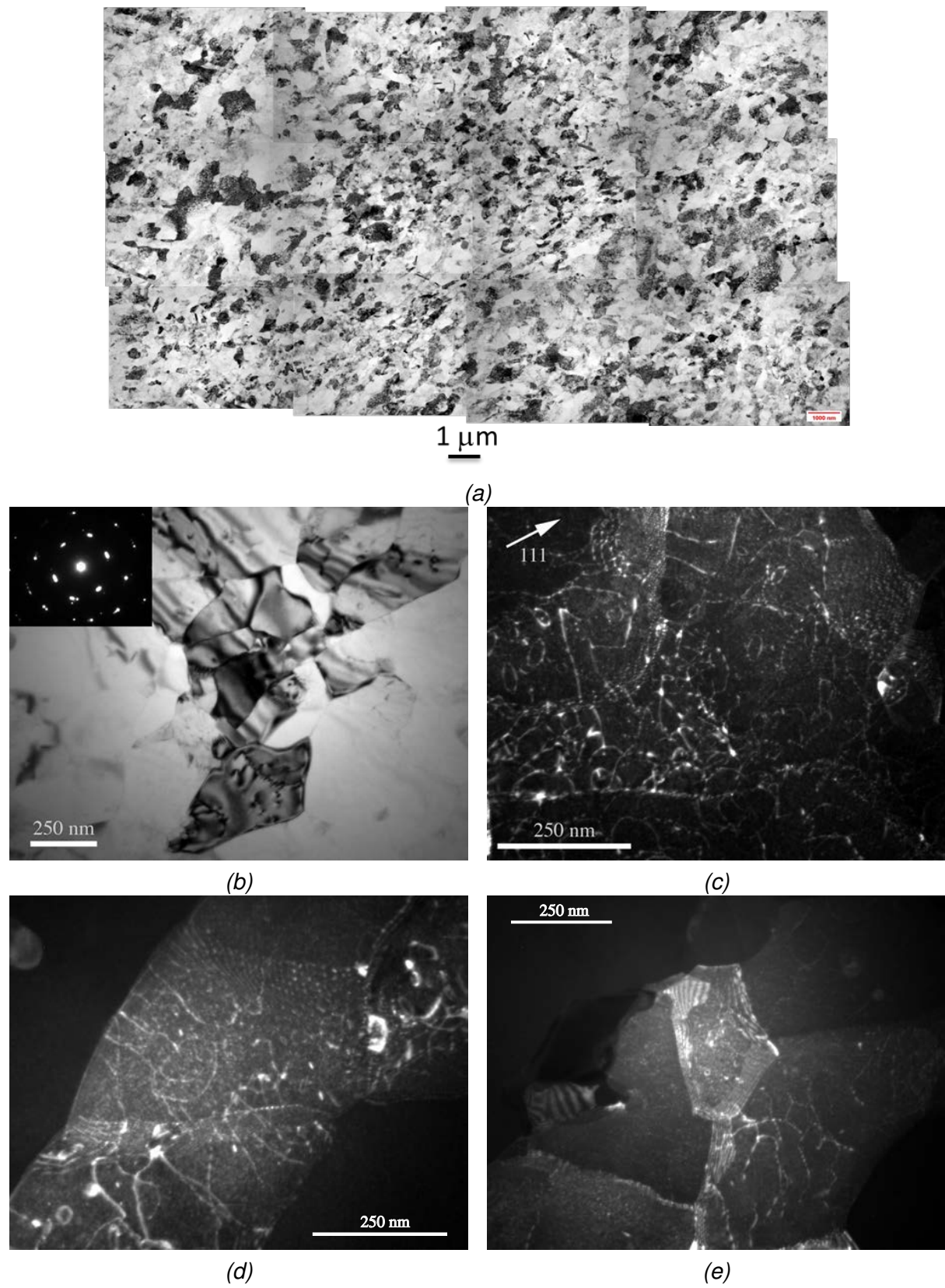
Figure 6.10: TEM observations of UFG LCF samples at \varepsilon_p = \pm 2 \times 10^{-3}
