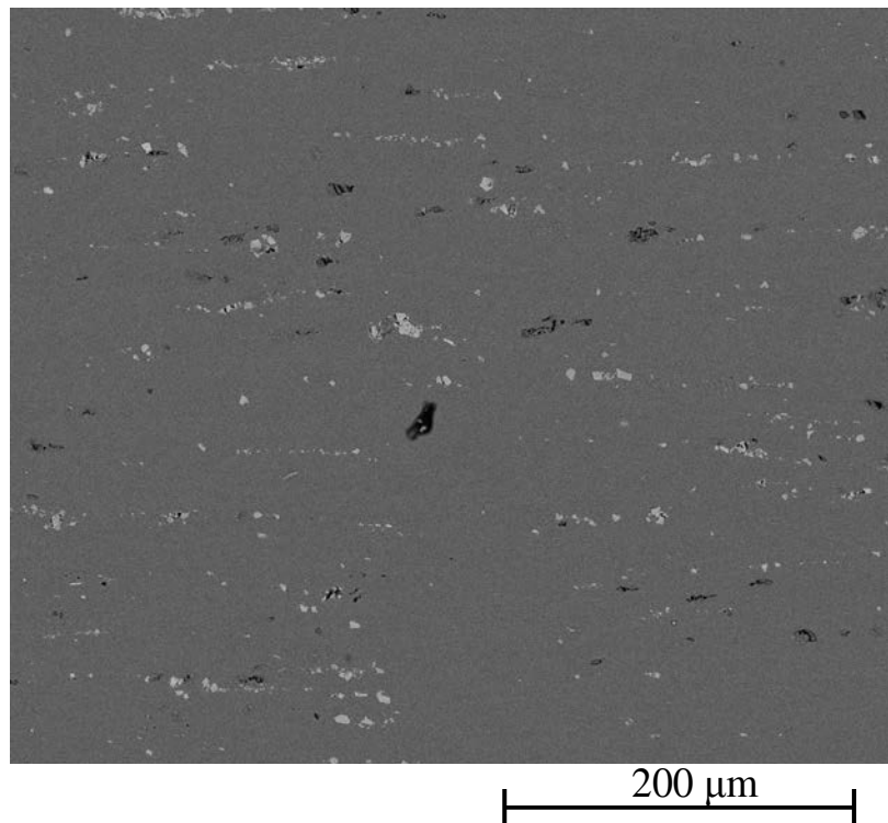
Figure 2.29: BSE image of the longitudinal section of UFG-B material with extrusion axis along the horizontal line.
