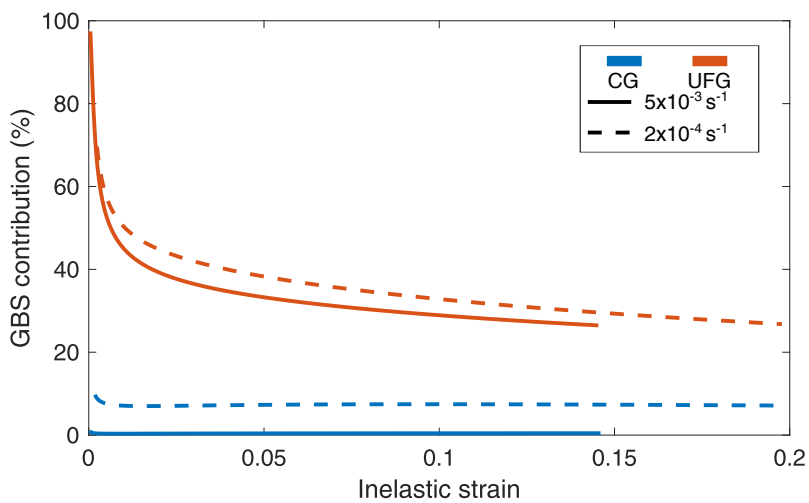
Figure 5.31: Effect of the strain and the strain rate on the contribution of GBS to the global inelastic strain during the simulated tensile tests at (a) 100°C and (b) 200°C
