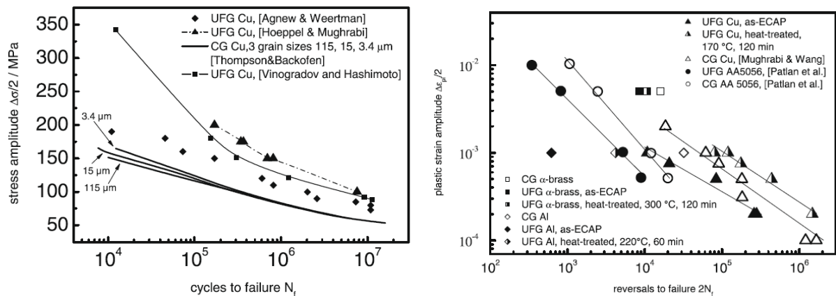
Figure 1.20: Wöhler (S-N) curve (left) and Coffin-Manson curve (right) for various CG and UFG materials [55].
