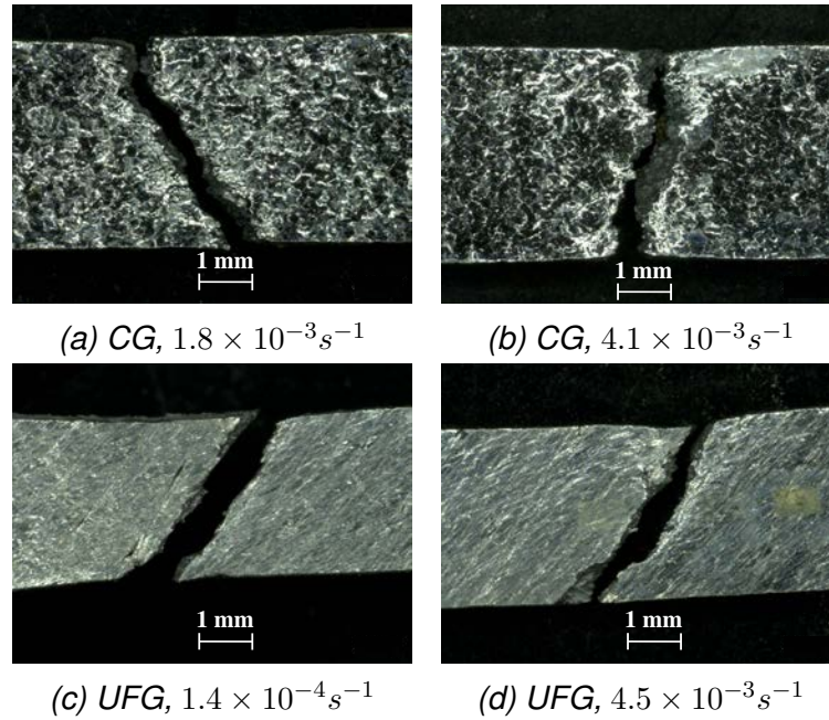
Figure 3.20: Optical images of the fractured samples at 200^\circ C
