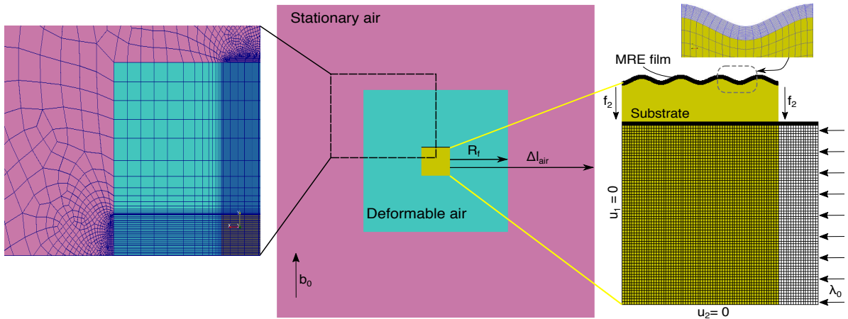
Figure III.2: Mesh of the film/substrate/air system. All regions are meshed with quadrilateral bilinear, 4-node isoparametric, (magneto)mechanical elements. A structured mesh with deformable elements (blue) is defined by the distance R_f from the solid boundary. The rest of the air region, defined by distance \Delta L_{air} from the solid boundary, is unstructured and stationary (purple).
