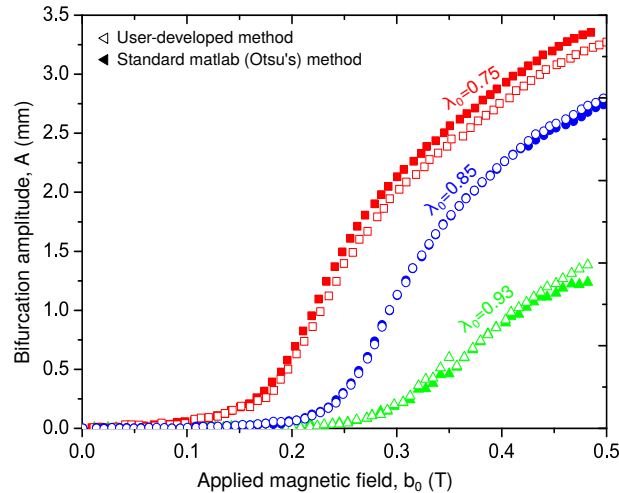
Figure II.9: Measurements of the experimental bifurcation amplitude A as a function of the magnetic field b_0 under three compressive pre-stretch ratios \lambda_0 = 0.75, 0.85, 0.93 . The bifurcation amplitude is assessed from the wrinkled film deflection profile, detected from the experimental images by means of the standard Matlab binarization (Otsu's) method and a user-developed method. For \lambda_0 = 0.75, 0.85 , the bifurcation curve corresponding to the user-defined method is obtained by detection of the film/air interface. For \lambda_0 = 0.93 , the relevant curve is obtained by detection of the film/substrate interface.
