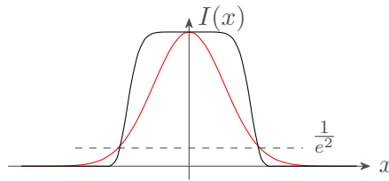
Figure 1.3: A Gaussian (red) and a top-hat (black) beam with the same 1/e^2 beam width.
