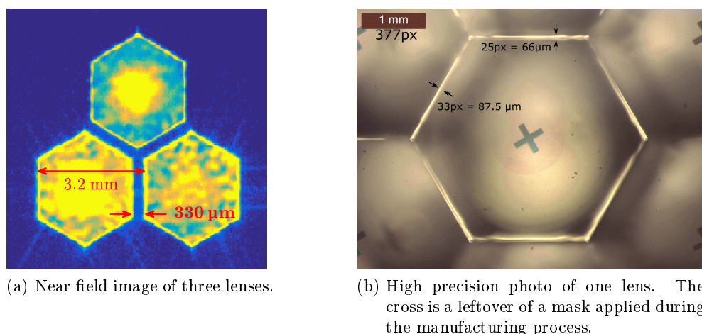
Figure 4.16: Estimations of the gap between the microlenses.
