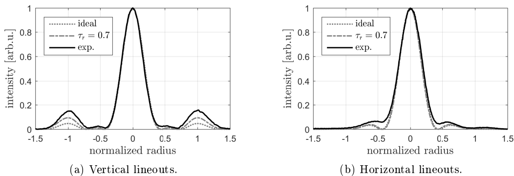
Figure 4.22: Lineouts of (gray, dotted) an ideal far field, (gray, dashed) a far field with reduced microlens fill factor, and (black, solid) the measured far field. The peak intensities of all lineouts are normalized to one.
