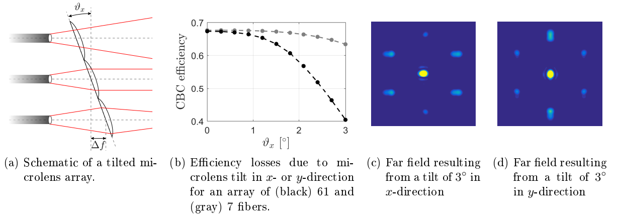
Figure 3.16: Microlens tilt.
