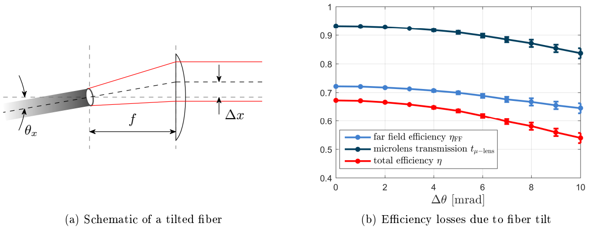
Figure 3.6: Fiber tilt.
