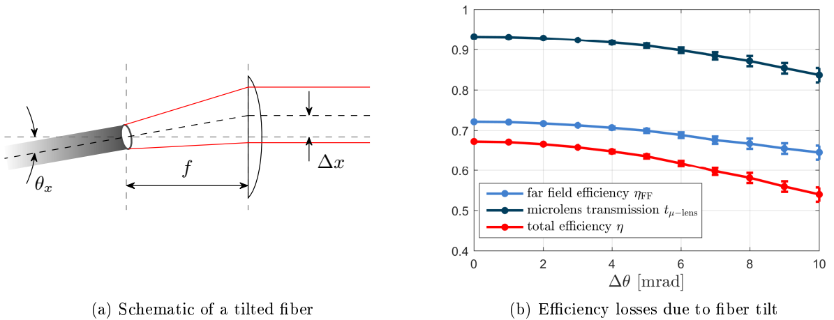
Figure 3.6: Fiber tilt.
