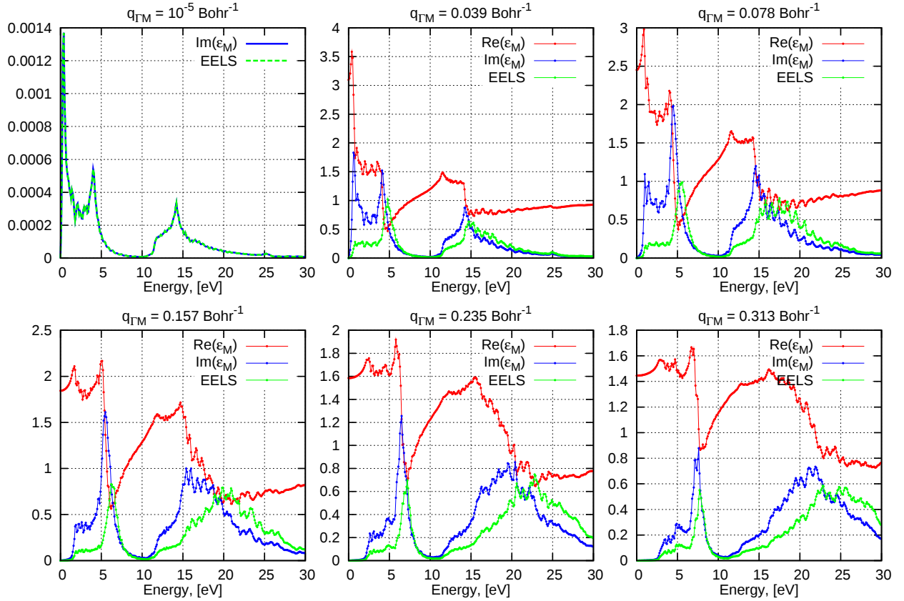
Figure 6.7: Real (red lines) and Imaginary (blue lines) parts of \varepsilon_M and EELS (green lines) for one graphene layer in R4 supercell for different \bar{q} ranging from 10^{-5} , 0.039, 0.078 for the top and 0.157, 0.235, 0.313 \text{Bohr}^{-1} for the bottom plots from left to right. (The first graph is calculated for vanishing \bar{q} : \text{Re}(\varepsilon_M) is not shown and is equal to 1). The local field effects are only along z ( npwmat_xy = 1 ; npwmat_z = 71 ). The calculations are done with the cutoff proposed by Novko et al [57].
