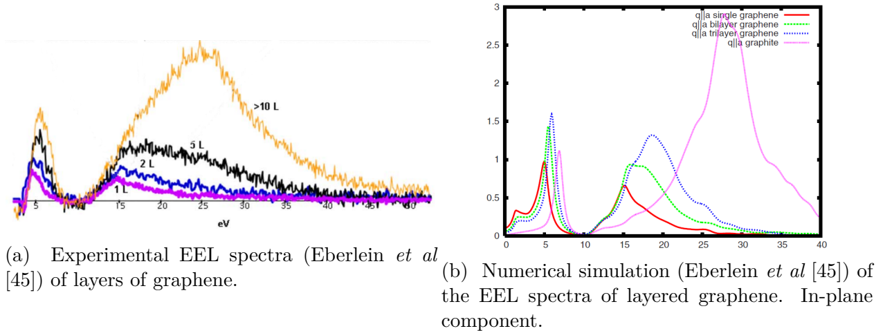
Figure 5.5: Eberlein EELS experiment (left) and numerical modeling (right). [45]
