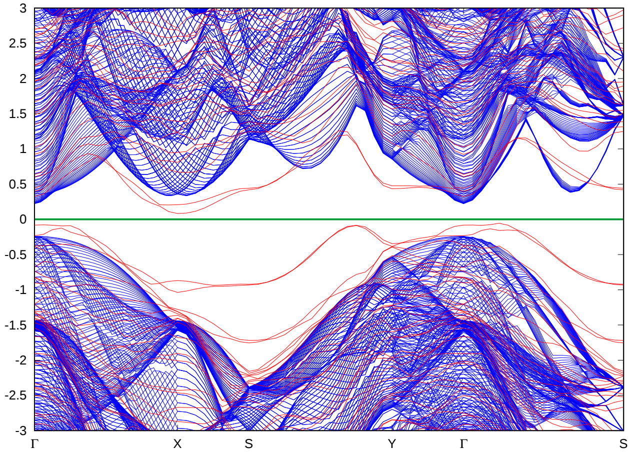
Figure 7.11: Surface states of the 4_4 relaxed slab (red) superposed to the surface projected bulk band structure (blue).
