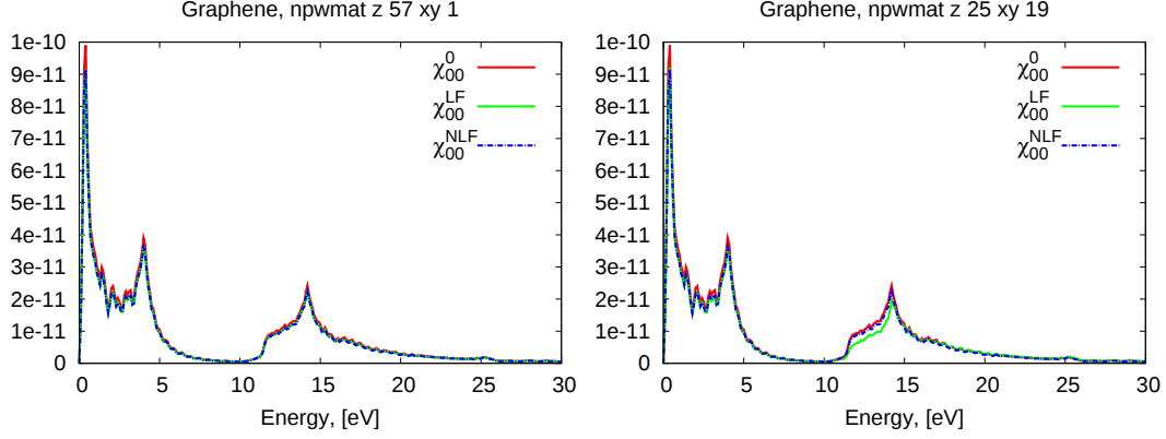
Figure 6.5: Different response functions implied in EELS for \bar{\mathbf{q}} = 10^{-5} \text{ Bohr}^{-1} : (red) \chi_{00}^0 , (blue) \chi_{00}^{NLF} and (green) \chi_{00}^{LF} , with \chi_{00}^{LF} calculated with LF only out-of-plane (left) and with LF in- and out-of-plane (right).
