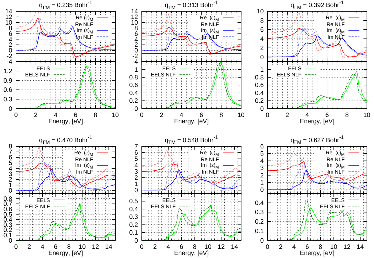
Figure 6.16: Real (red lines) and Imaginary (blue lines) parts of \varepsilon_M and EELS (green lines) for one graphene layer in R5 supercell for different \bar{q} ranging from 0.2 up to 0.7 \text{Bohr}^{-1} . The calculations are done on the (100 \times 100 \times 1) mesh, using slab potential and Selected- G method with ( npwmat_xy = 19; npwmat_z = 7). The corresponding dashed lines are the spectra without LF.
