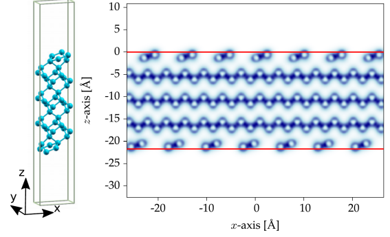
Figure 4.2: Left: Slab of 32 atoms corresponding to the (2x1) surface reconstruction in a supercell. Right: electronic density obtained by DFT calculation. The red lines shows the limit of matter in the supercell.
