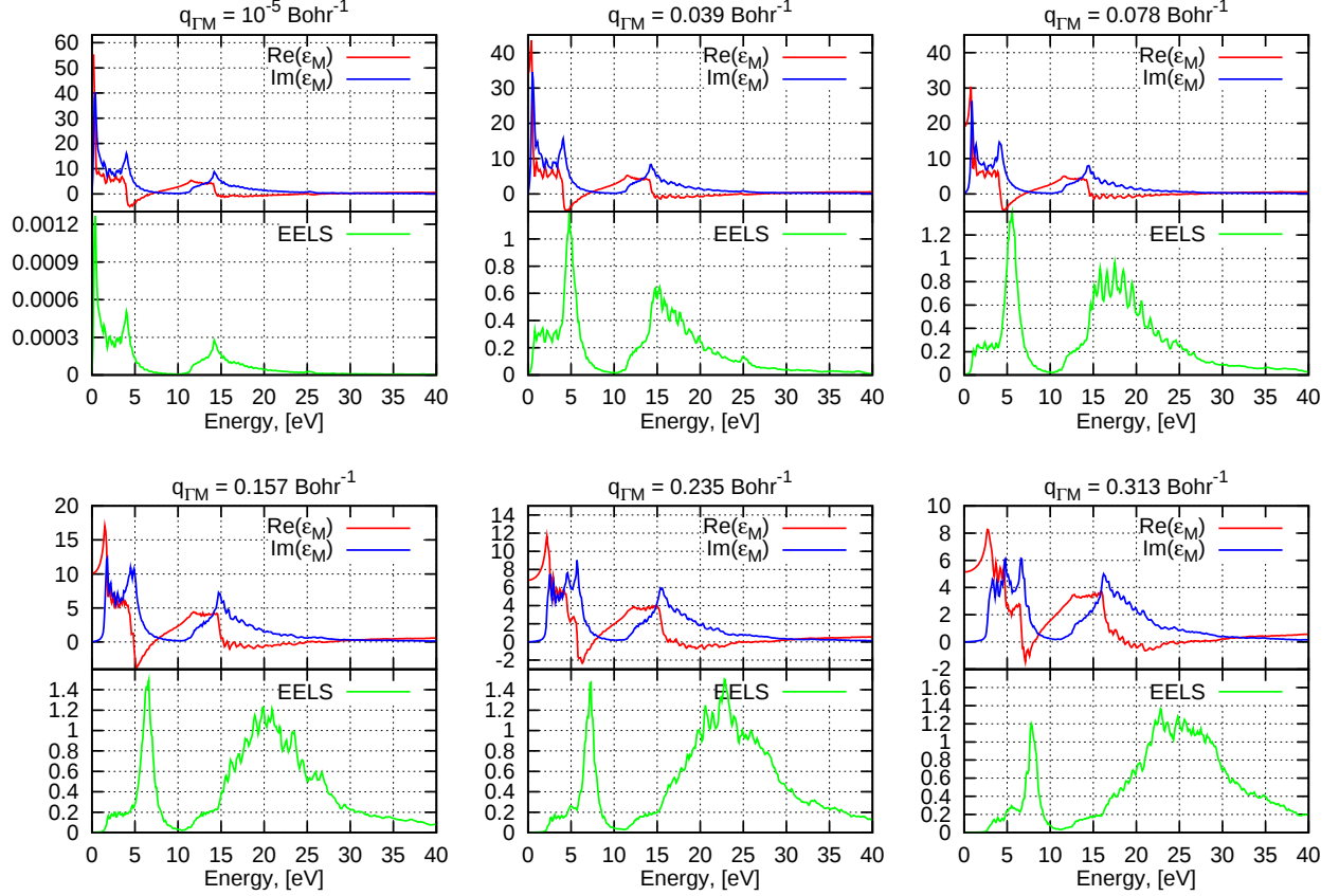
Figure 6.9: Real (red lines) and Imaginary (blue lines) parts of \varepsilon_M and EELS (green lines) for one graphene layer in R4 supercell ( R4 = 25.173 \text{ Bohr} ) for different \bar{\mathbf{q}} ranging from 10^{-5} , 0.039, 0.078 for the top and 0.157, 0.235, 0.313 \text{Bohr}^{-1} for the bottom plots from left to right. (The first graph is calculated for vanishing \bar{\mathbf{q}} ). The calculations are done with slab potential and Selected- G method with ( npwmat_xy = 19; npwmat_z = 7).
