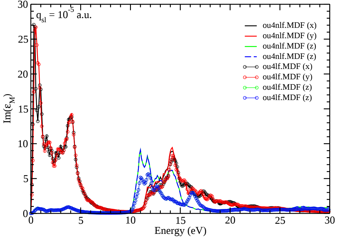
Figure A.10: \text{Im}(\varepsilon_M^{NLF}) [lines without dots (ou4nlf.MDF)] compared with \text{Im}(\varepsilon_M^{LF}) [lines with dots (ou4lf.MDF)] for q_{sl} = 10^{-5} \text{ a.u.} : (black) spectra for q_x component; (red) spectra for q_y component; (green) spectra for q_z component (extracted from linear combination of spectra calculated with q_x and q_x \pm q_z ), and (blue) spectra for q_z component (extracted from linear combination of spectra calculated with q_y and q_y \pm q_z ).
