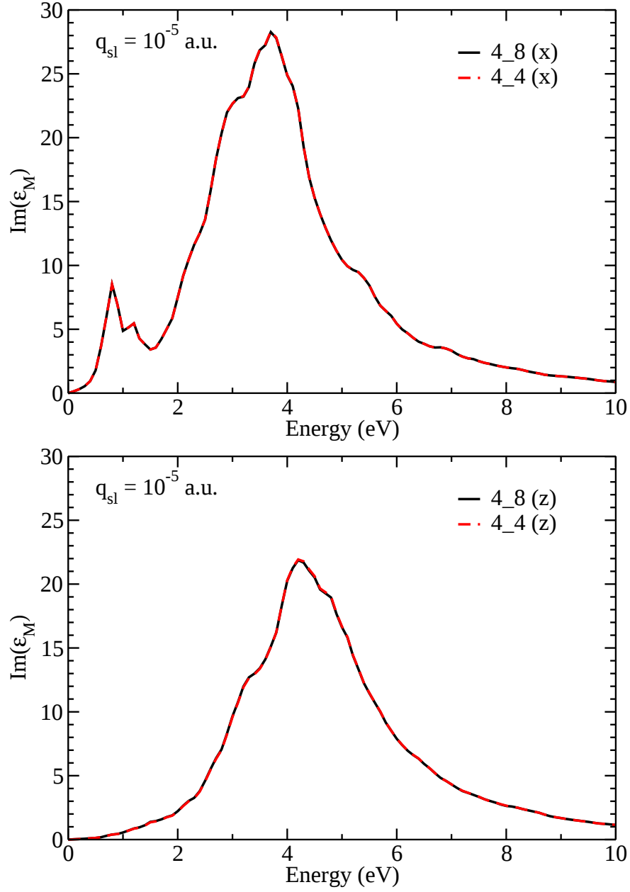
Figure 5.1: Comparison of Im(\epsilon_M) for the 4_4 (black) and of 4_8 (red) supercells. Top: in-plane component. Bottom: out-of-plane component.
