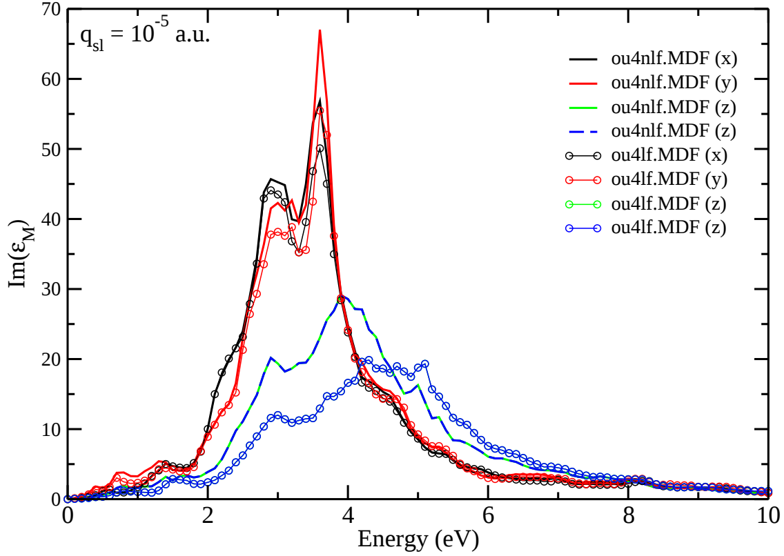
Figure A.2: \text{Im}(\varepsilon_M^{NLF}) [lines without dots (ou4nlf.MDF)] compared with \text{Im}(\varepsilon_M^{LF}) [lines with dots (ou4lf.MDF)] for q_{sl} = 10^{-5} \text{ a.u.} : (black) spectra for q_x component; (red) spectra for q_y component; (green) spectra for q_z component (extracted from linear combination of spectra calculated with q_x and q_x \pm q_z ), and (blue) spectra for q_z component (extracted from linear combination of spectra calculated with q_y and q_y \pm q_z ).
