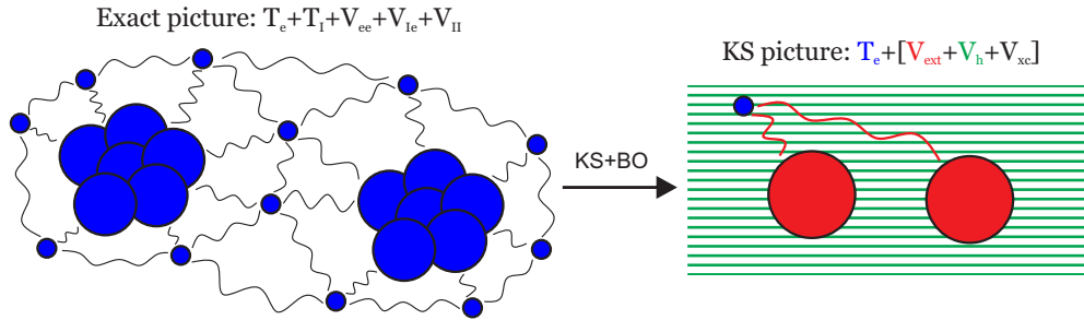
Figure 2.1: Kohn-Sham schematic picture representation.
