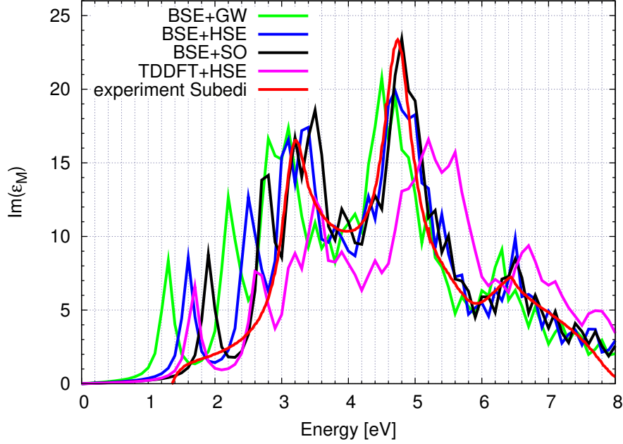
Figure 8.5: InP absorption spectrum calculated within BSE formalism. Green: GW corrections, blue: HSE corrections, black: scissor operator 1 eV. (For memory, TDDFT-LDA+HSE is in magenta). Experiment from experiment from [70] is in red.
