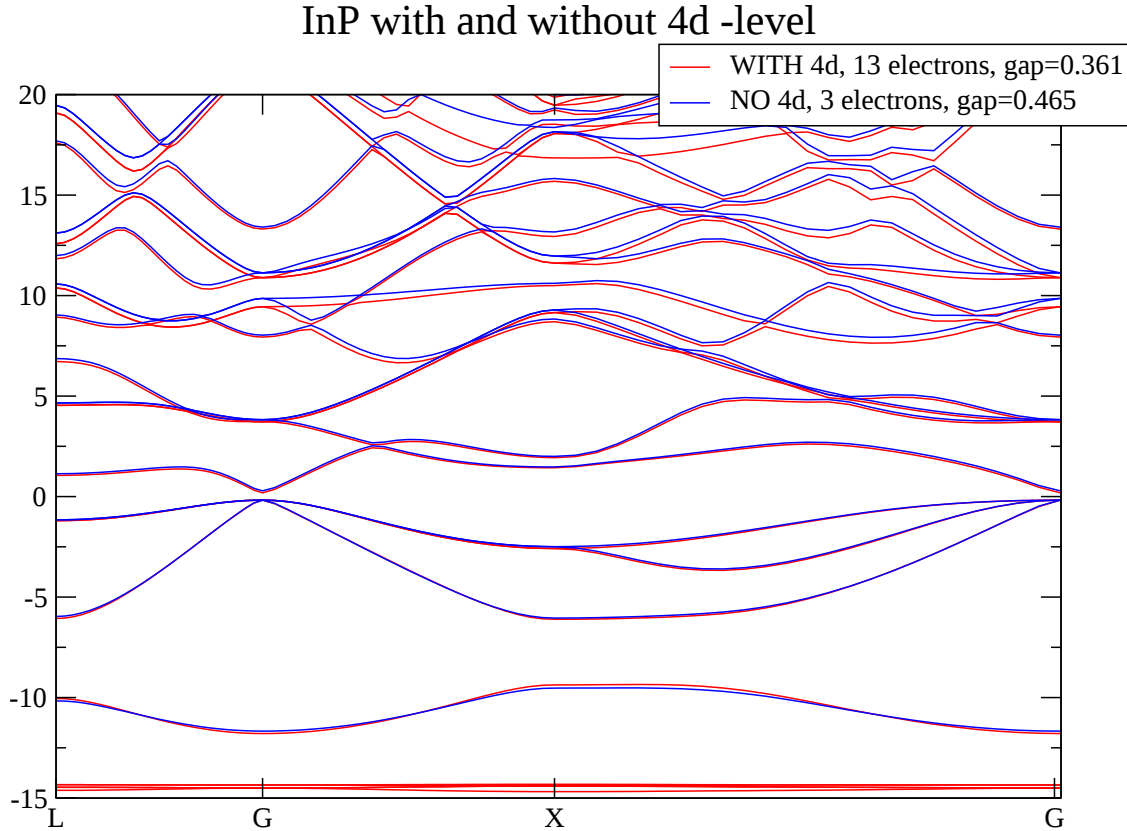
Figure 8.2: InP bulk, with and without 4d level.
