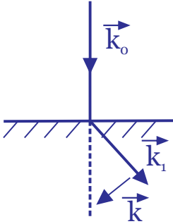
Figure 5.2: The schematic representation of an EELS experiment.
