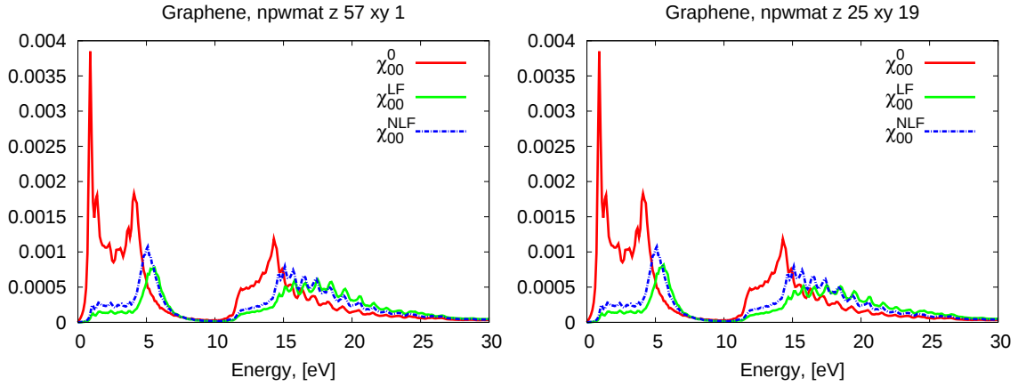
Figure 6.6: Different response functions implied in EELS for \bar{\mathbf{q}} = 0.078 \text{ Bohr}^{-1} : (red) \chi_{00}^0 , (blue) \chi_{00}^{NLF} and (green) \chi_{00}^{LF} , with \chi_{00}^{LF} calculated with LF only out-of-plane (left) and with LF in- and out-of-plane (right).
