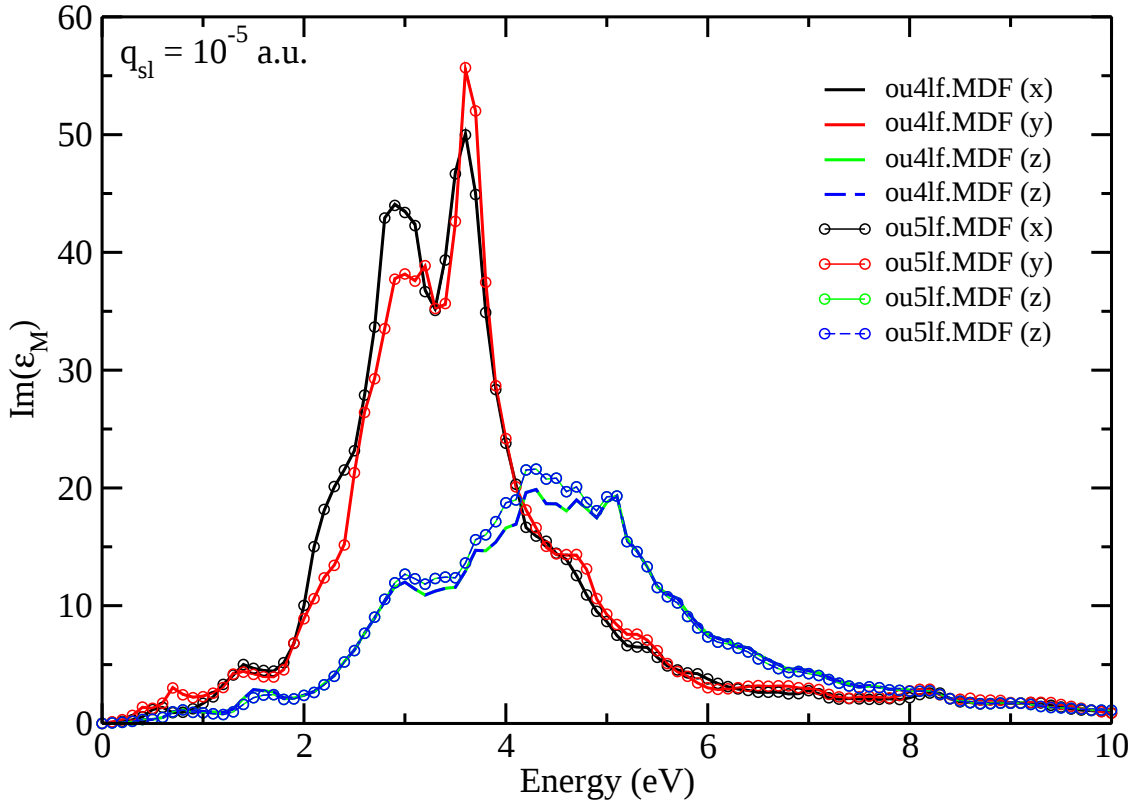
Figure A.3: Comparison of \text{Im}(\varepsilon_M^{LF}) for the slab [lines without dots (ou4lf.MDF)] and the surface [lines with dots (ou5lf.MDF)] q_{sl} = 10^{-5} \text{ a.u.} : (black) spectra for q_x component; (red) spectra for q_y component; (green) spectra for q_z component (extracted from linear combination of spectra calculated with q_x and q_x \pm q_z ), and (blue) spectra for q_z component (extracted from linear combination of spectra calculated with q_y and q_y \pm q_z ).
