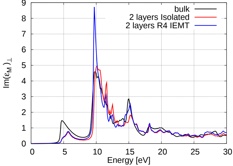
Figure 7.3: out-of-plane component of \text{Im}(\epsilon_M) resulting from IEMT on the 2-layer slab into R4 supercell (blue line) compared to the bulk spectrum (black line) and to the isolated slab (red line). k-point mesh: 40 \times 40 \times 1 for Isolated slab and IEMT ; 40 \times 40 \times 15 for the bulk.
