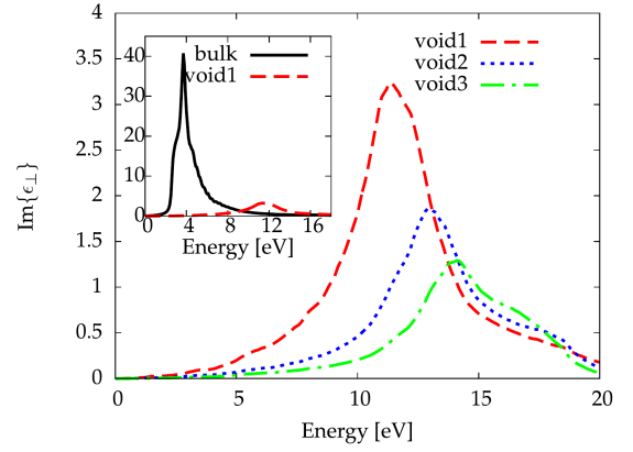
Figure 4.4: Absorption spectra along the z-direction for a silicon surface in RPA for the three different supercells.
