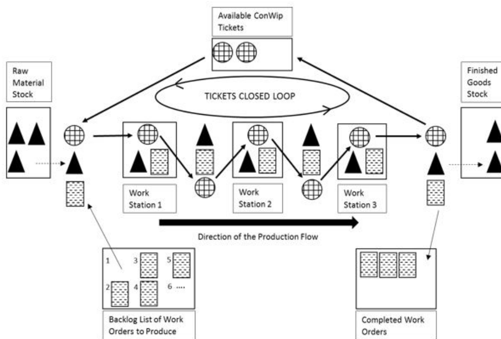
Figure 3. Principe du ConWip
