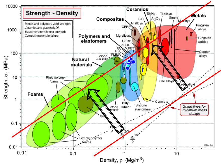
Figure 4.3. Strength, \sigma_f , against Density, \rho
