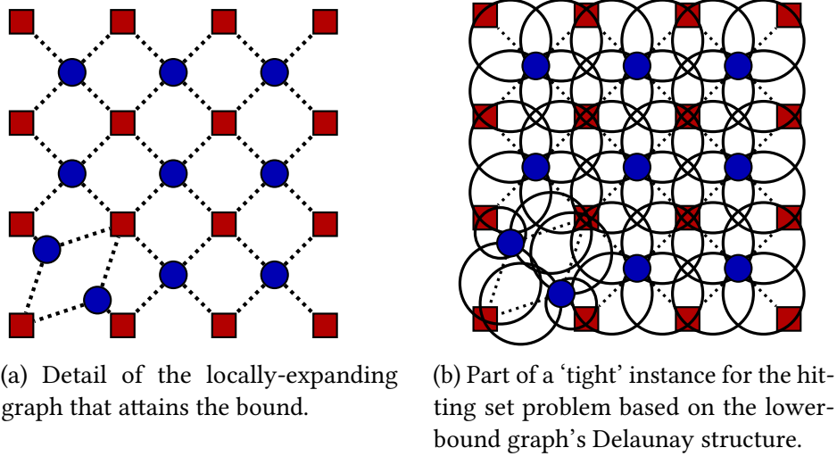
Figure 0.5: Lower bound construction and algorithmic consequences
