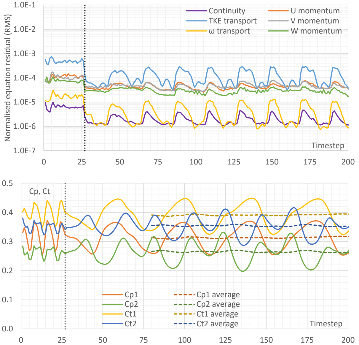
Fig. 35 Exemplary temporal evolution of simulation monitors in a CRSR simulation ( TSR_1 = 3.67 , TSR_2 = 3.45 ); normalised equation residuals (RMS values) for 6 governing equations solved in FRM simulation (top); Cp and Ct for both turbines (dashed line is moving average from last 80 iterations, bottom); the black dotted line denotes the iteration in which \Delta t was changed from n = 1 ( 15^\circ ) to n = 5 ( 3^\circ )
