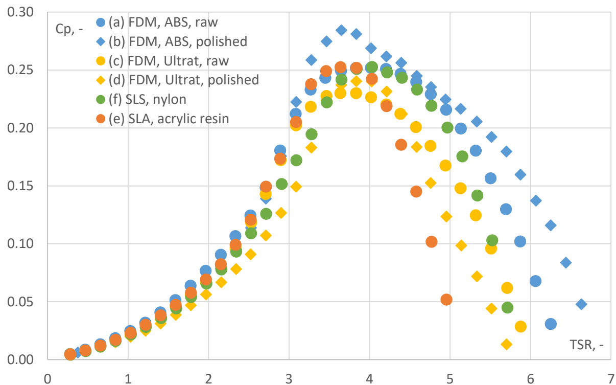
Fig. A2.6 Performance of rotor specimens with blades made of different materials and/or techniques
