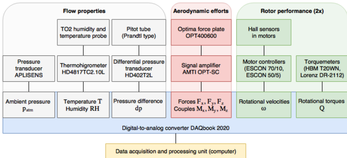
Fig. 21 Wind tunnel measurement apparatus schema
