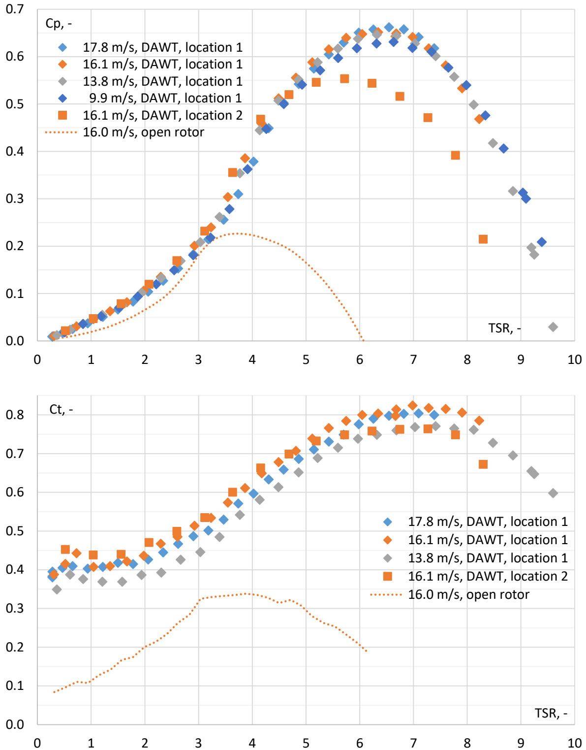
Fig. 26 C_p (TSR) (top) and C_t (TSR) for different relative wind speeds; R1 DAWT (squares, diamonds) in downwind, and open rotor (dotted line) in upwind configuration
