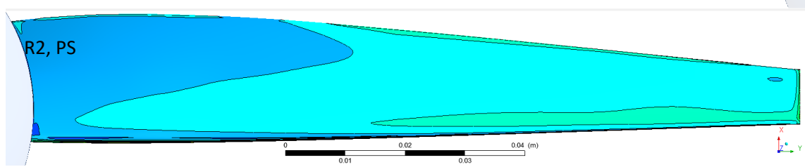
Fig. 36 Y^+ distribution on the surfaces of test stands and diffuser (top) and wind turbine blades (bottom); CRSR, TSR_1 = 3.67 , TSR_2 = 3.45 ; SS – suction side, PS – pressure side; colour code is the same for all images
