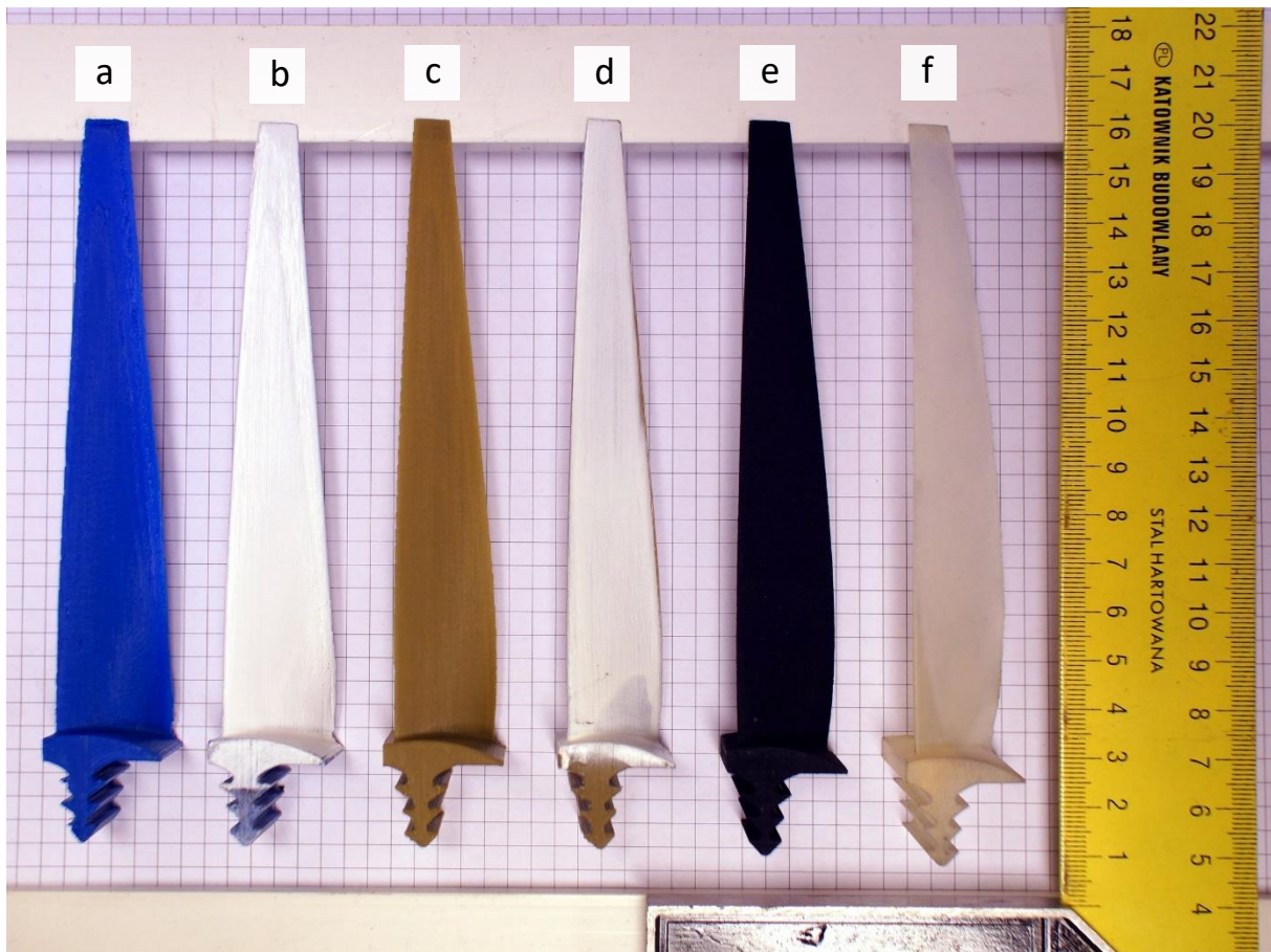
Fig. A2.5 3D-printed blades of various materials: ABS (a, b – before and after surface treatment), Ultrat (c, d – before and after surface treatment), nylon (e), acrylic resin (f)
