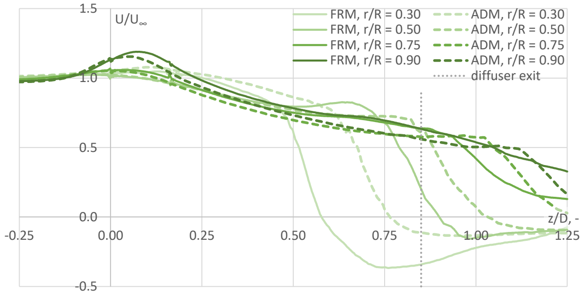
Fig. 69 Streamwise distribution of normalised axial velocity at 4 locations (b); simulation data: FRM (continuous line) and ADM (dotted line); CSR, TSR_1 = TSR_2 = 5.03
