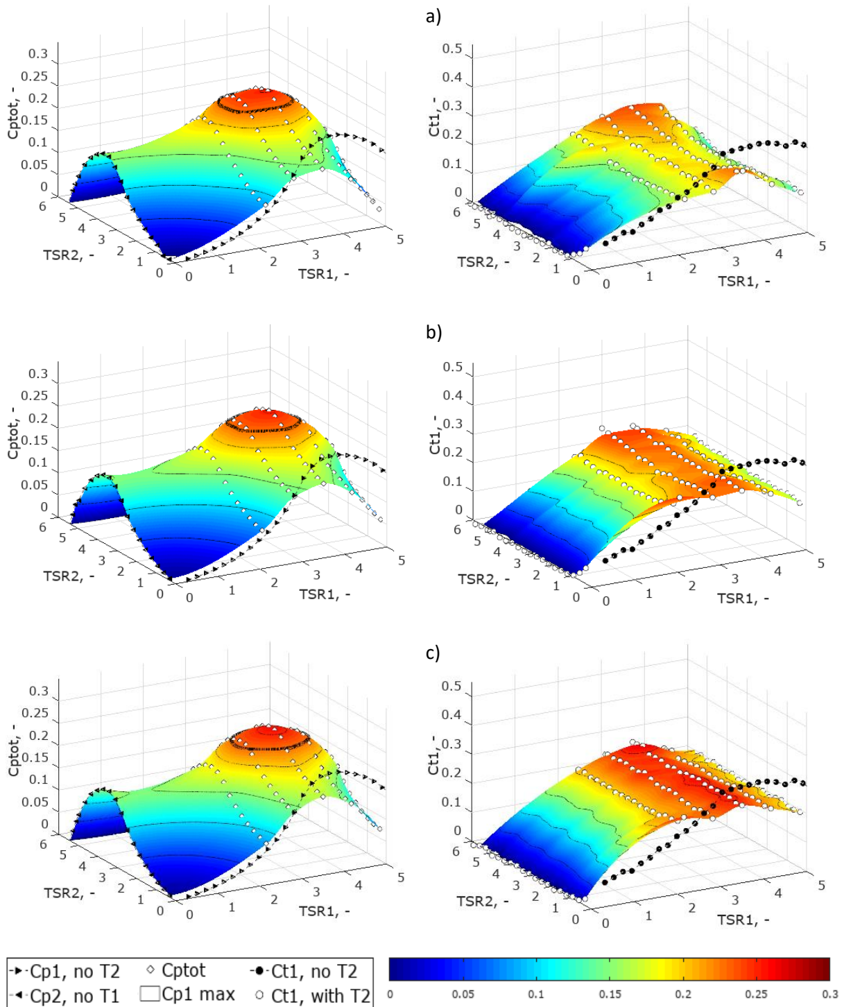
Fig. 28 C_{ptot}(TSR_1, TSR_2) (left) and C_{t1}(TSR_1, TSR_2) (right) for rotors operating in CROR mode; rotor separation distance: 0.1D (a, top), 0.3D (b, middle), 0.625D (c, bottom); black points denote performance when only the considered rotor (either 1 or 2) is examined; thick black line on the C_{ptot} graphs denotes C_p = 0.226 , the maximum recorded C_p of bare rotor
