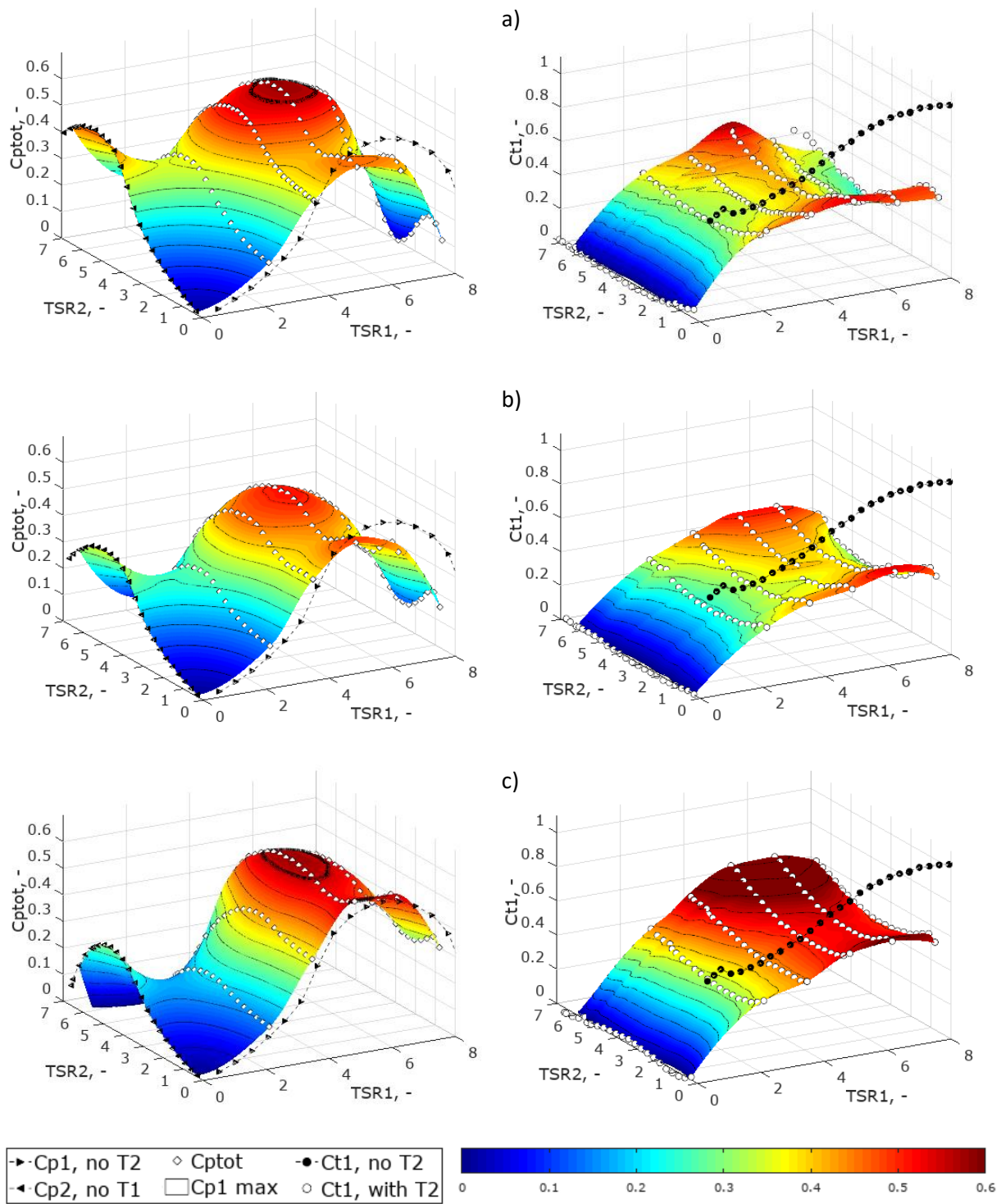
Fig. 30 C_{ptot}(TSR_1, TSR_2) (left) and C_{t1}(TSR_1, TSR_2) (right) for rotors operating in CRSR mode; rotor separation distance: 0.1D (a, top), 0.3D (b, middle), 0.625D (c, bottom); black points denote performance when only the considered rotor (either 1 or 2) is examined; thick black line ( C_{p1} max) on the C_{p1} graph denotes C_p = 0.554 , the maximum recorded C_p for DAWT
