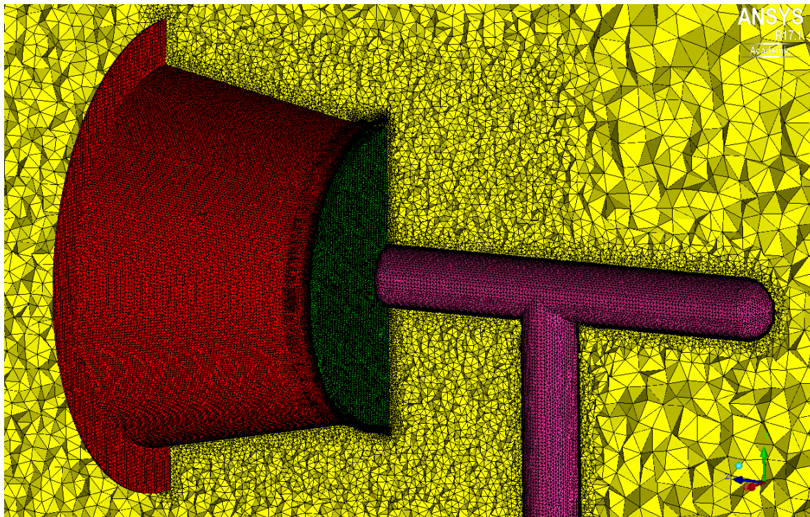
Fig. 32 Vertical section (yellow, x = 0 m) view of the stationary domain mesh in rotor vicinity in DAWT simulations; rotor interface marked green, diffuser marked red, T1 test stand marked pink
