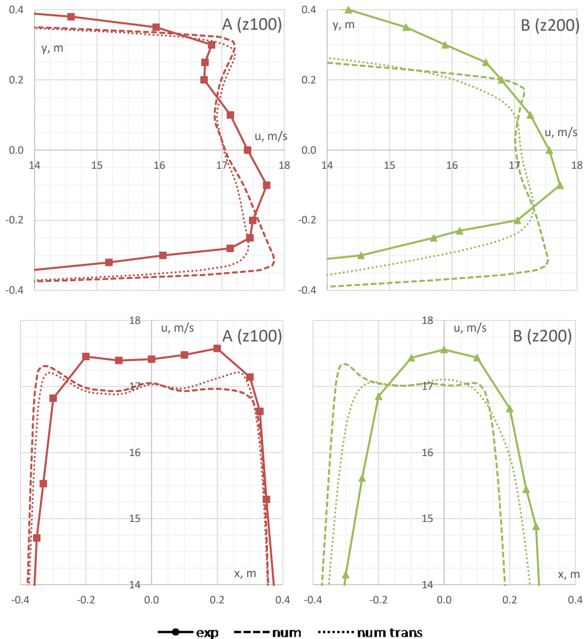
Fig. A1.5 Axial velocity vertical (top) and horizontal (bottom) distribution at locations A ( z=100 ) and B ( z=200 ); continuous line marks experimental data, dashed – numerical steady state, dotted – numerical transient
