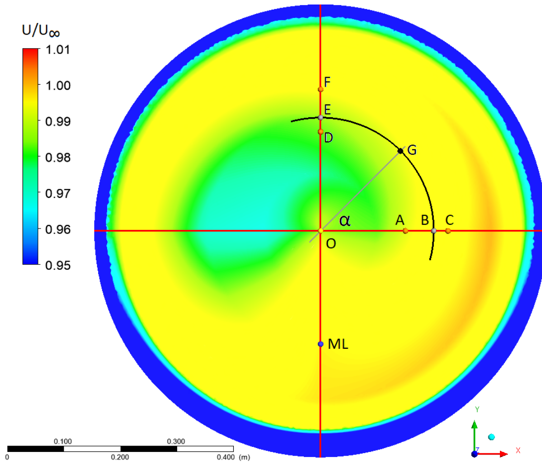
Fig. A1.3 Normalised axial velocity distribution at the test section inlet (interpolation in ANSYS CFX, U_\infty = 15.95 m/s)
