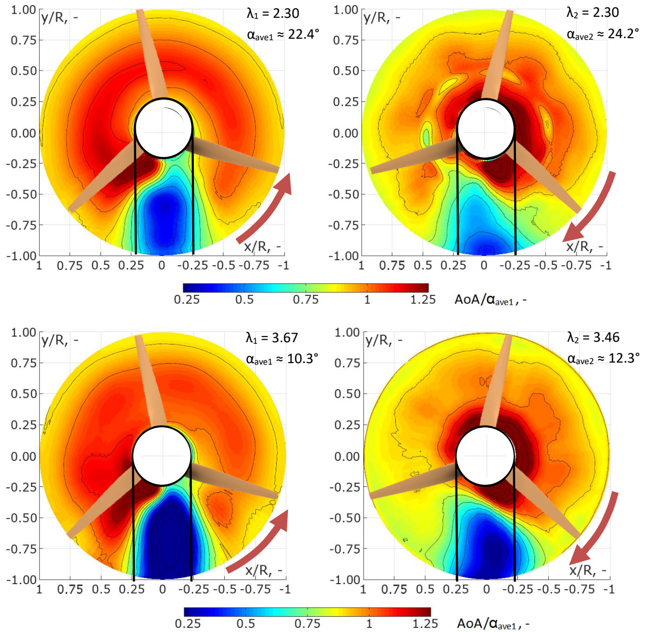
Fig. 46 Normalised AoA distribution in the plane of rotation (PoR) of upstream (left) and downstream (right) rotor in CRSR cases at TSR 2.3 (top) and approximately 3.5 (bottom) as seen from inflow direction (DAWT); red arrows denote the direction of rotation, black lines denote pole location
