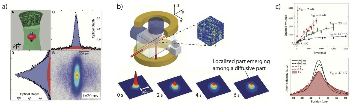
Figure 2.5: Observations of three-dimensional Anderson localization with ultracold atoms in (a) De Marco’s group in Urbana-Champaign [40], (b) atom optics group in Palaiseau [41], and (c) the group of Modugno and Inguscio in Florence [42].
