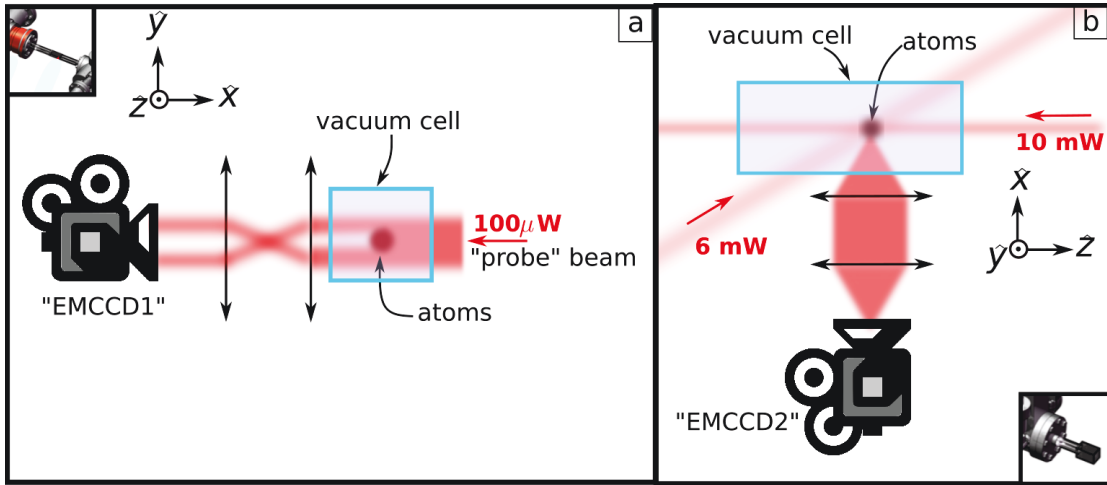
Figure 3.2: (a) Absorption imaging. A resonant probe pulse is sent to the atomic cloud, is partially absorbed, and is collected by camera “EMCCD1”. The information on the cloud is obtained from the quantity of the light absorbed. (b) Fluorescence imaging. Several resonant probes are sent simultaneously to the atomic cloud. The atomic cloud emits fluorescent light which is partially collected by camera “EMCCD2”. The information on the cloud is obtained from the estimation of the fluorescence light.
