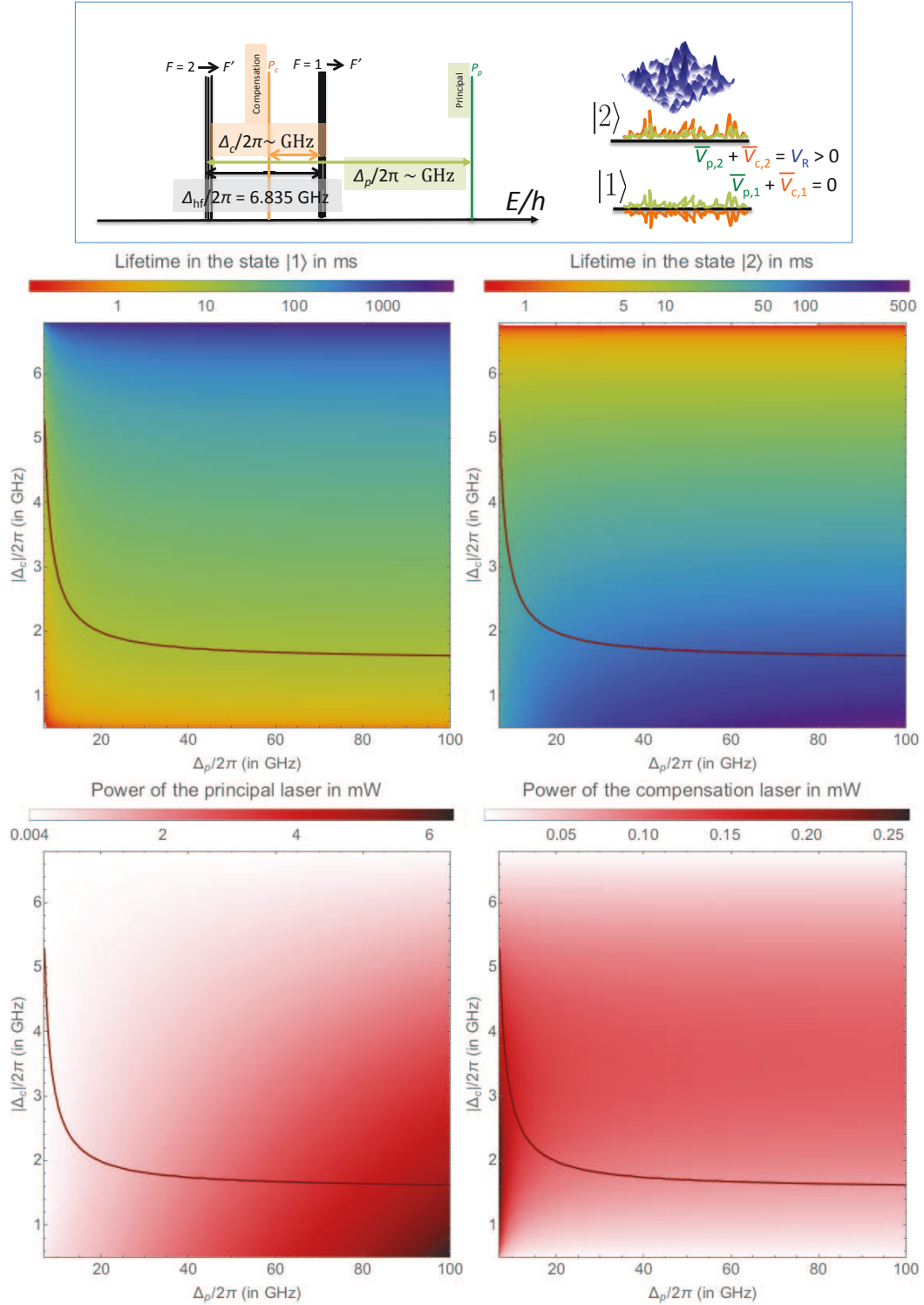
Figure 6.4: Numerical results for repulsive case; V_R/h = 4 \text{ kHz} . First row: schema taken from Fig. 6.2. Second row: Atomic lifetimes in the states |1\rangle (Left) and |2\rangle (Right), shown in logarithmic color scale. The empty area on the left corresponds to \tau_1 \leq 0.1 \text{ ms} ; on the right, \tau_2 \leq 0.5 \text{ ms} . Third row: The required power for the principal laser ( P_p , left) and the compensation laser ( P_c , right). The detunings \Delta_p and |\Delta_c| ( \Delta_c < 0 ) are shown in horizontal and vertical axes respectively. Dark red line corresponds to situation where \tau_1 = 10 \text{ ms} .
