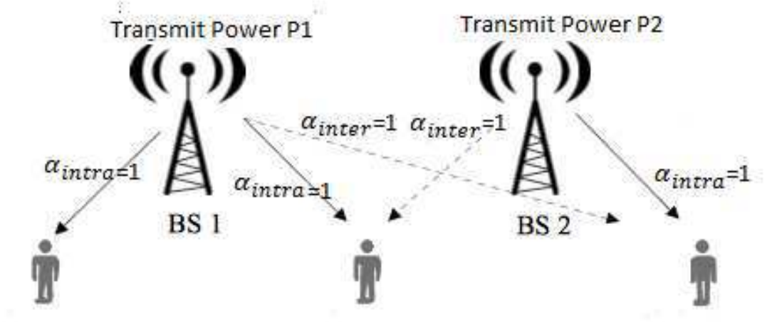
FIGURE 3.4: Figure corresponding to Assumption 3.2
