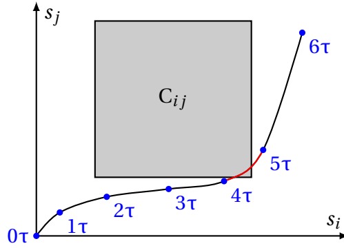
Figure A.2 – Example of corner-cutting phenomenon: all points (corresponding to successive time steps) are outside of the collision region, but the resulting trajectory intersects with C_{ij} . Blue labels indicate the corresponding time instant.
