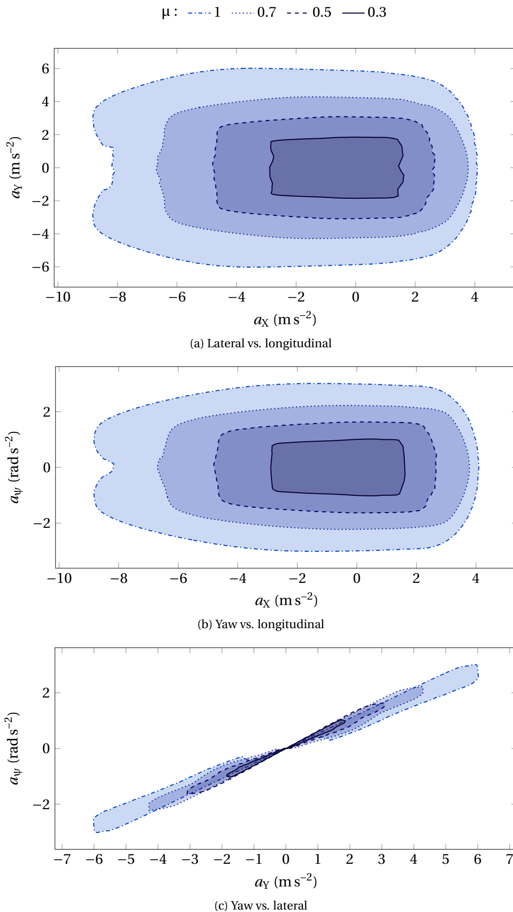
Figure D.6 – Envelope of the sets of feasible accelerations for v_0 = 20 \text{ m s}^{-1} and varying \mu , with 10^5 sampling points
