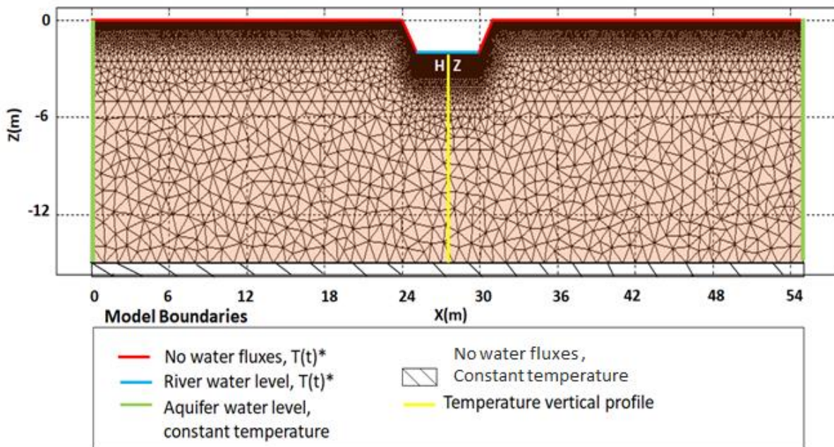
Figure 3.2 : hydro-thermal model mesh and its boundary conditions (*:T(t) time-varying prescribed temperature, calculated based on (Hillel, 1982))
