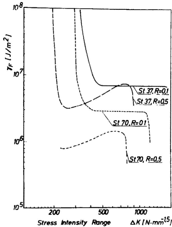
Figure 1.12: Specific plastic work spent to create a unit of fracture surface, [Pippan and Stüwe, 1992].
