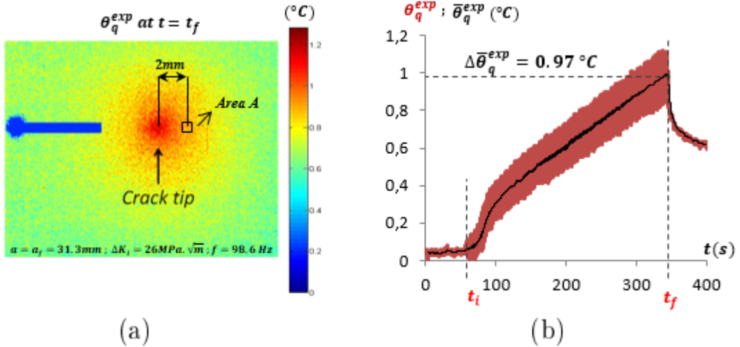
Figure 2.23: (a) Infrared measurement of \theta_q^{exp} at the end of the applied load block of fatigue test T015 . (b) Evolution of \theta_q^{exp} and \bar{\theta}_q^{exp} , spatially averaged in Area A, against time during the whole applied loading block.
