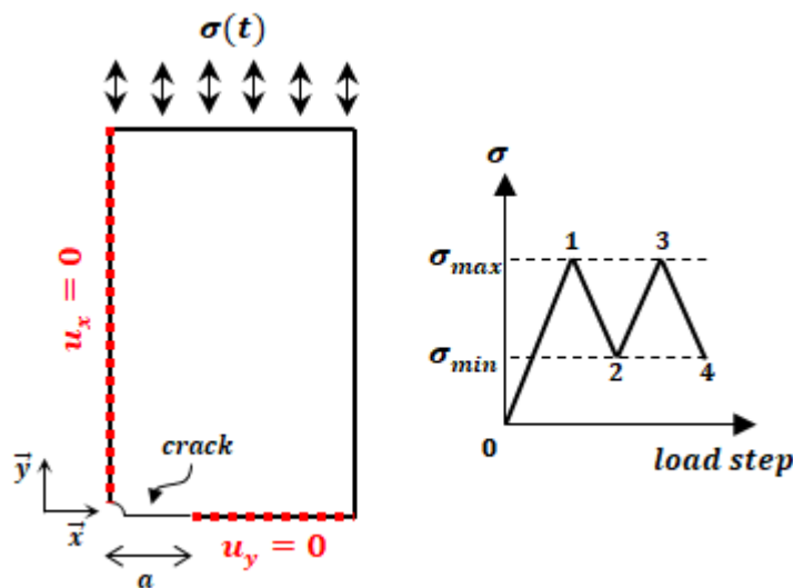
Figure 4.22: Boundary conditions and applied load steps.
