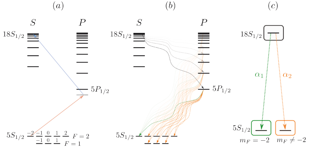
Figure 25 – Desexcitation of the Rydberg states
