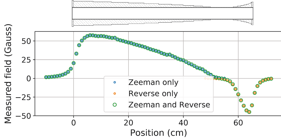
Figure 68 – Typical magnetic field of the Zeeman slower
