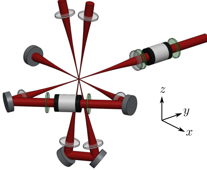
Figure 11 – Bowtie-shaped lattice
