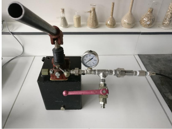
FIGURE 8.13 : Manual water pump.
