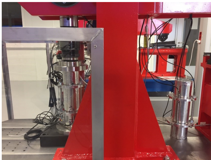
FIGURE 9.18 : Autogenous shrinkage and creep specimens on a big test bench.
