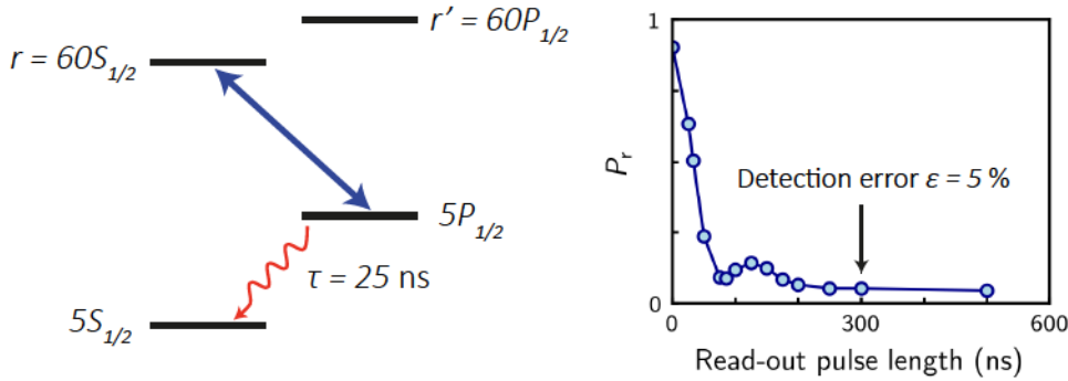
Figure 7.6: Read-out pulse. Left: The 475 nm beam is shone on resonance between a single Rydberg state |r\rangle and the short-lived ( \tau = 25\ \text{ns} ) intermediate 5P_{1/2} level. Right: The strong spontaneous emission leads to an extremely fast damping of the |e\rangle \leftrightarrow |r\rangle Rabi oscillation, as the atom decays to the ground-state. In our experiments, we shine the read-out pulse during 300 ns, 6 times as long as the fitted decay time constant. There remains a \epsilon = 5\% probability not to recapture the atom, which will be considered as an atom in |r'\rangle and thus causes a detection error.
