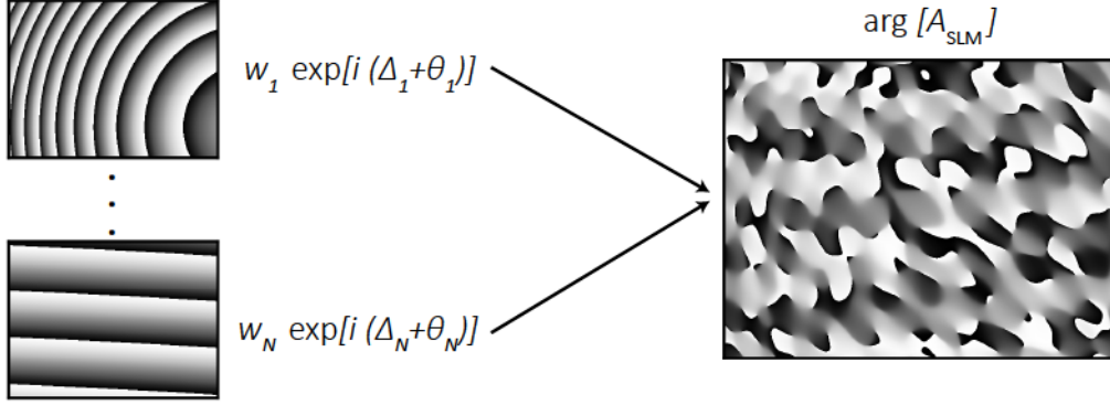
Figure 2.8: Hologram for N traps. N elementary phase patterns \Delta_m are combined to give an interference pattern A_{SLM} , see Eq. (2.6), whose phase \arg[A_{SLM}] is the phase mask displayed on the SLM.
