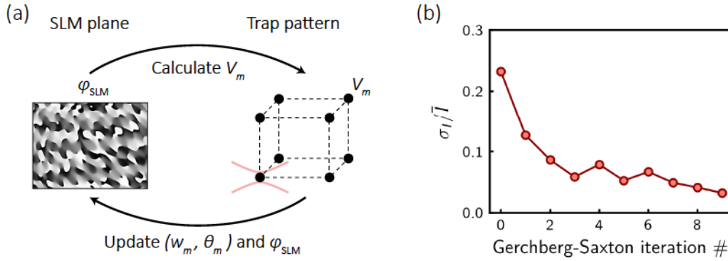
Figure 2.9: Gerchberg-Saxton algorithm. (a) Schematic of the weighted GS algorithm. We only calculate the amplitude of the light field V_m at the trap centers, and not over the entire 3D volume where it is a complicated interference of all the individual tweezers (light red). (b) Relative standard deviation \sigma_I/I of the trap intensities I measured on the camera. It decreases with the number of iterations down to \sigma_I/I \simeq 3\% .
