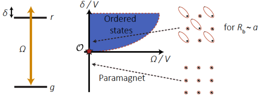
Figure 4.1: Phase diagram of laser-driven Rydberg ensembles. Left: a two-level atom is driven from the ground-state |g\rangle to the Rydberg level |r\rangle . The coupling strength is \Omega and the detuning from the transition is \delta . Middle: Phase diagram in the \Omega - \delta plane for a repulsive van der Waals shift between atoms ( C_6 > 0 ). Above the critical point \mathcal{O} = (0, 0) , there is a crystalline phase where the position of the Rydberg excitations are strongly correlated to minimize the interaction energy. Outside this region, the laser drive dominates the interaction and the many-body ground-state is a paramagnet. In this chapter, we will explore the properties of the system close to the critical point \mathcal{O} . This figure is adapted from Weimer et al. [2008] .
