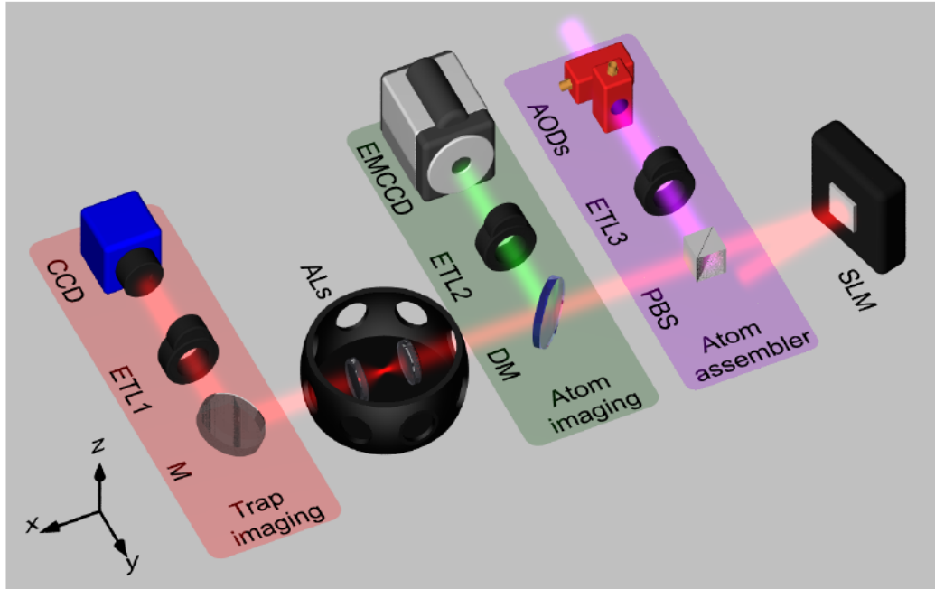
Figure 2.2: Experimental setup for creating ordered 3D structures of single atoms. The aspheric lenses (ALs) in the vacuum chamber focus a collimated beam to create an optical tweezers, which can load a single atom. The spatial light modulator (SLM) imprints a phase mask on the trapping beam duplicating a single tweezers in a 3D array of traps. The trap imaging setup gives an image of the trapping structure and the atom imaging system of the atomic fluorescence. The deflectors (AODs) in the atom assembler part create a moving tweezer used to assemble atom one by one in an ordered atomic pattern. Tunable lenses (ETL) allow to work on different planes of the 3D structures.
