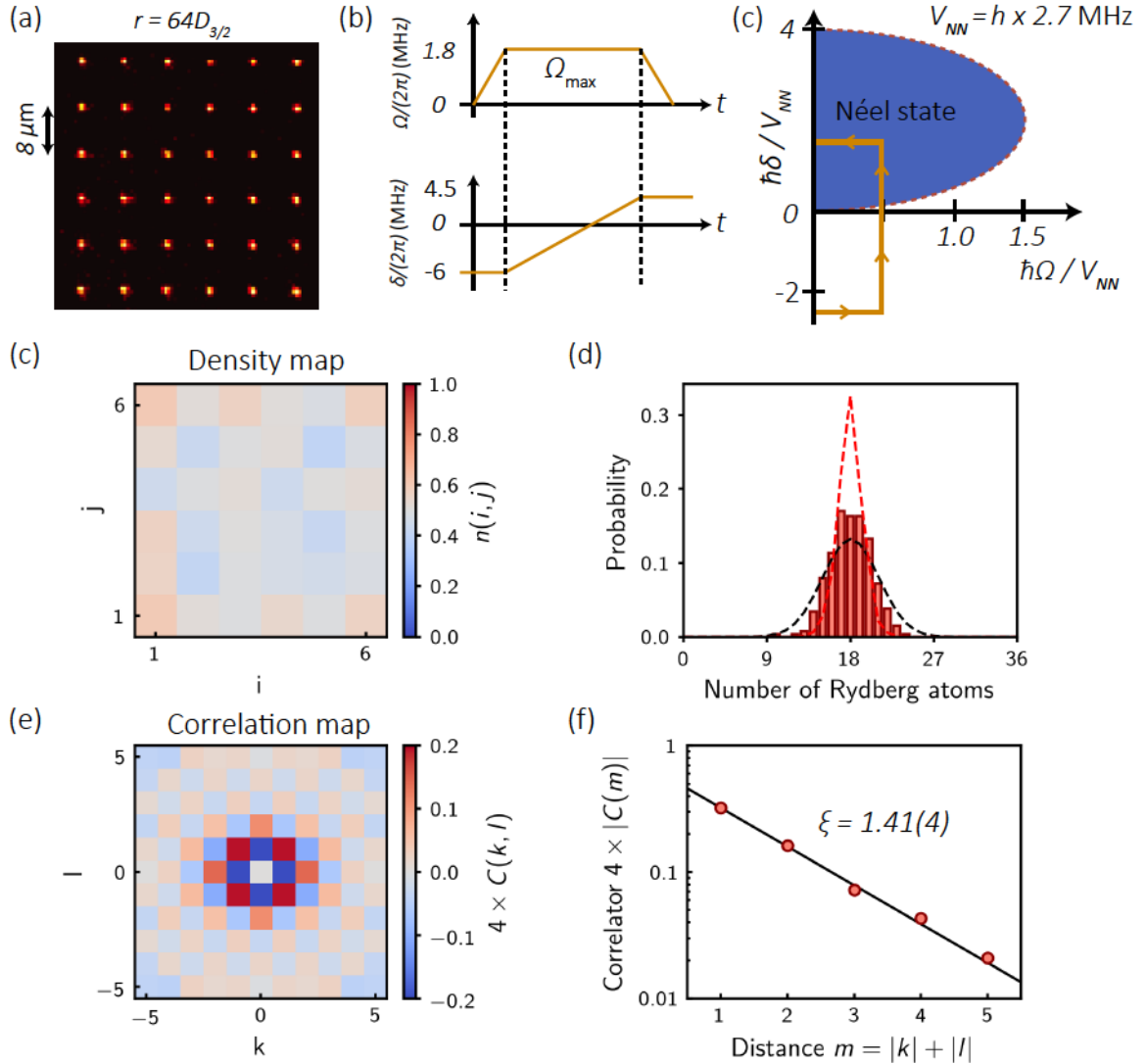
Figure 4.4: Creation of antiferromagnetic-like correlations with an adiabatic sweep. (a) 6 \times 6 atomic array driven to the Rydberg state |r\rangle = |64D_{3/2}, m_J = 3/2\rangle with time-dependent laser drive \Omega(t) and detuning \delta(t) shown in (b). Phase diagram and system trajectory (orange path) ending deep in the crystalline phase. (c) Quasi-homogeneous density map obtained at the end of the sweep. (d) Histogram of the number of Rydberg excitations for 264 experimental runs showing a squeezed distribution around \bar{N}_{\text{exc}} = 18 = N/2 . The dashed line is a binomial distribution that would be expected for independent atoms, the red line is the predicted histogram for the Néel state taking into account detection errors (\varepsilon, \varepsilon') = (4, 4)\% . (e) Measured correlation map 4 \times C(k, l) showing an antiferromagnetic pattern with a sign alternating as (-1)^{|k|+|l|} . For a perfect Néel state, the correlation would be saturated at \pm 1 . (f) Exponential decrease of the absolute value of the correlator with the distance m = |k| + |l| . The extracted correlation length is \xi = 1.41(4) .
