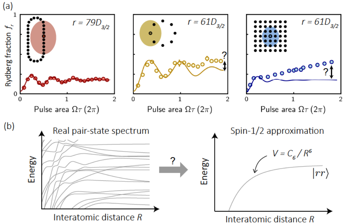
Figure 6.2: Failure of spin-1/2 mapping. (a) Experiments reported in Labuhn et al. [2016]: the excitation lasers are switched on with a strength \Omega for a variable time \tau , the fraction f_r of Rydberg excitations is shown as a function of the pulse area \Omega\tau . Each inset shows the atomic array and the extent of the Rydberg blockade volume. In two cases, the data deviate from numerical simulations of a spin-1/2 model (solid lines). (b) We will show that the deviations originate from the approximation of the real pair-state spectrum (left panel, worst-case scenario) by a single potential curve (right panel).
