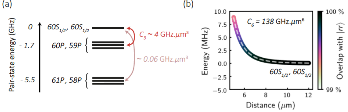
Figure 6.6: nS_{1/2} states: van der Waals regime. (a) Closest pair-states to |rr\rangle = |60S_{1/2}, 60S_{1/2}\rangle and their C_3 coupling. (b) Numerical calculations from the pairinteraction software. The thick colored curve represents the eigenstate energy and its overlap with |rr\rangle , which remains > 99.5\% for R > 5 \mu\text{m} . The dashed curve shows the C_6/R^6 van der Waals scaling.
