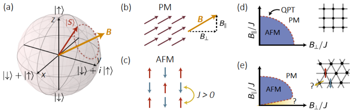
Figure 1.1: Spin-1/2 models. (a) Bloch sphere representation of a spin-1/2 (red arrow) precessing around a magnetic field B (orange arrow). (b) An ensemble of spins aligning along B forming a paramagnet (PM). (c) Anti-ferromagnetic Néel ground-state (AFM) of an Ising Hamiltonian with J > 0 . (d) Phase diagram of the quantum Ising model at zero temperature showing a quantum phase transition (QPT) between a PM and AFM phase. B_{\parallel} and B_{\perp} are the magnetic field components parallel and transverse to the Ising-favored z -axis. (e) A triangular lattice frustrates the anti-ferromagnet constraints and an exotic phase is expected when interaction dominates.
