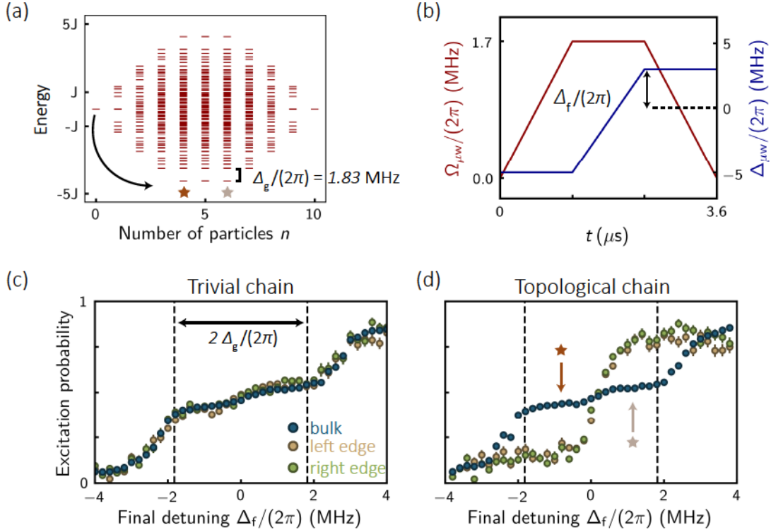
Figure 8.10: Sweeps to half-filling. (a) We aim at preparing one of the four degenerate ground-state of the topological chain with a microwave sweep. (b) Time-dependent microwave coupling strength \Omega_{\mu w}(t) and detuning \Delta_{\mu w}(t) ending at \Delta_f . (c,d) We scan the final detuning \Delta_f and measure the excitation probability of bulk sites (blue) and edge sites (green and brown) for the trivial (c) and topological (d) setup (right). For a sweep ending in the gap (dashed line), the bulk of the chain is half-filled. Bosons are loaded in the edge sites of the topological setup when \Delta_f > 0 .
