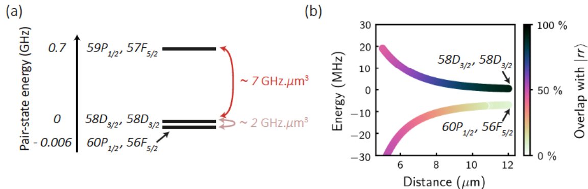
Figure 6.7: 58D_{3/2} states: quasi-resonant regime. (a) The coupling strength to |59P_{1/2}, 57F_{5/2}\rangle is larger than to |60P_{1/2}, 56F_{5/2}\rangle , but the latter is almost resonant with |rr\rangle = |58D_{3/2}, 58D_{3/2}\rangle and thus dominates the interaction. (b) Numerical calculation showing the strong mixing of the two quasi-resonant channels. The interaction energy varies between \sim \sqrt{2}C_3/R^3 at short distances and \sim C_6/R^6 with C_6 = 2C_3^2/\Delta E at large distances.
