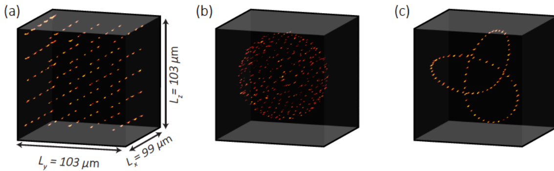
Figure 2.14: Arbitrary 3D trap patterns. Intensity reconstructions of exemplary 3D patterns obtained from a collection of x-stack images taken with the trap CCD camera. The regions of maximum intensity form (a) a 5 \times 5 \times 5 cubic array, (b) a C_{320} fullerene-like structure, and (c) a trefoil knot. The dimensions of the images are (\sim 100 \mu\text{m})^3 .
