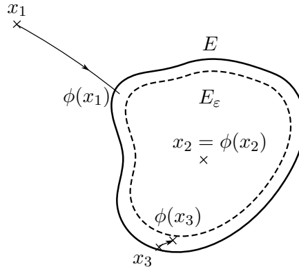
Figure 10.1: Sketch of the construction of the diffeomorphism \phi in Lemma 10.2.1 : one follow the flow \kappa given by Condition \mathfrak{C} for a more or less long time depending on the initial point. E_\varepsilon denotes the set where \phi is the identity. \varepsilon measuring the "width" of E \setminus E_\varepsilon can be chosen sufficiently small for K to be included in E_\varepsilon .
