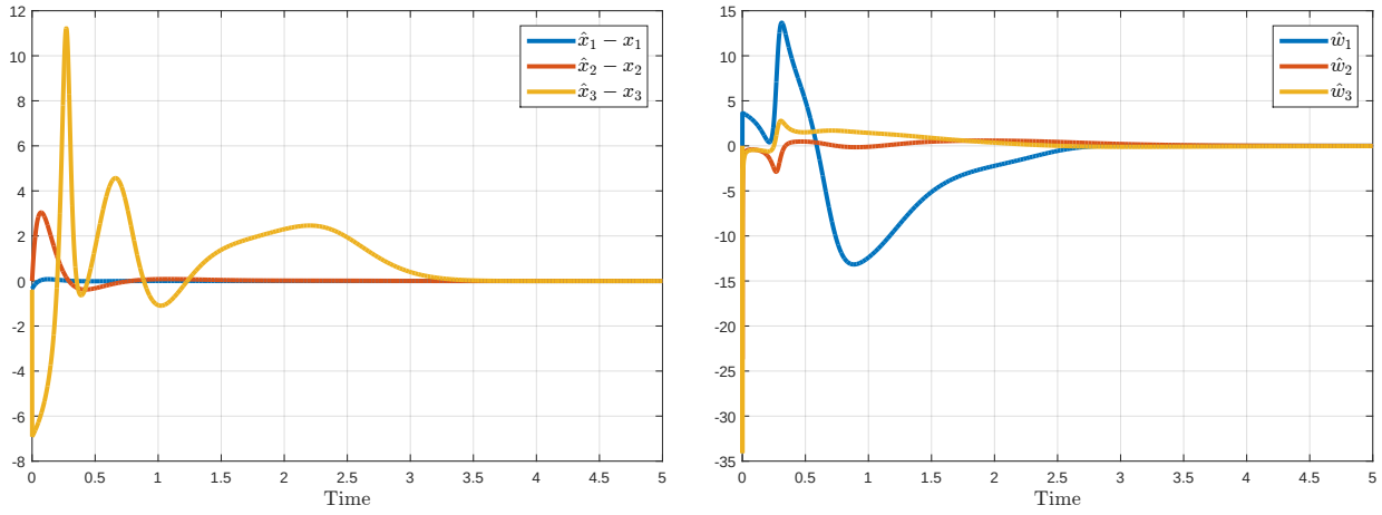
Figure 11.1: High gain observer (11.5) with \hat{x}_1 = \hat{x}_2 = \hat{x}_3 = 0 at the singularity, L = 3 , k_1 = 10 , k_2 = 35 , k_3 = 50 , k_4 = 24 . The simulation was done with a step-variable Euler algorithm.
