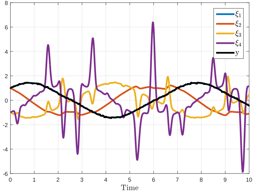
Figure 4.1: Trajectory of System (4.27), with initial condition \xi = (1, 1, -1, -1) , with input u = 5 \sin(10t) and with the noisy measurement y (filtered gaussian noise with standard deviation \sigma = 0.03 and 1st order filtering parameter a = 50 ), used to test the observers.
