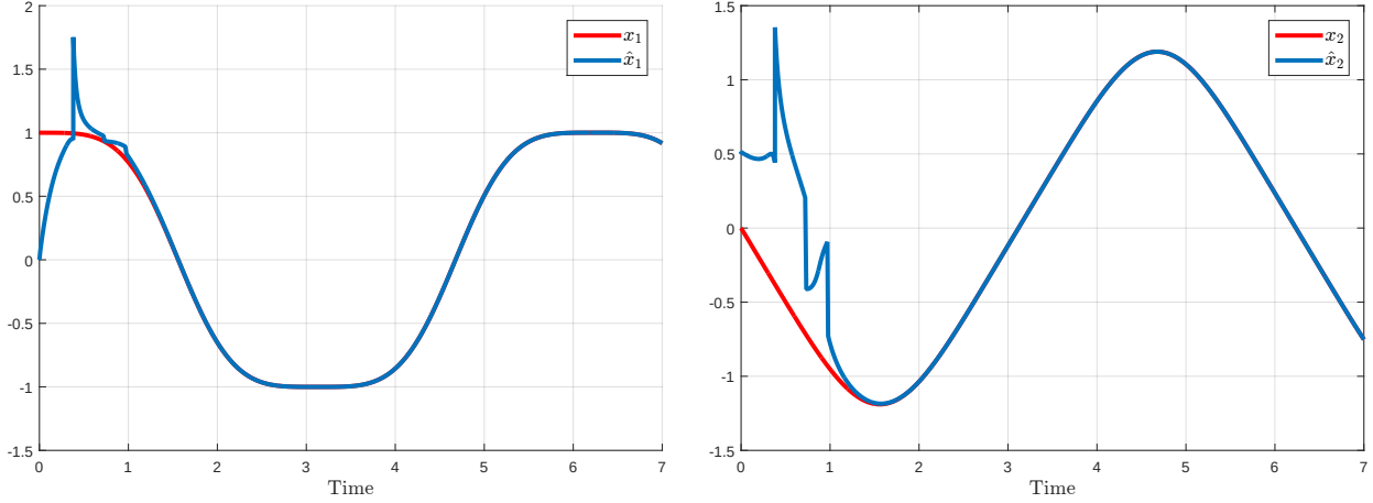
Figure 7.1: Nonlinear Luenberger observer for System (7.19) : dynamics (7.20) and transformations (7.21) (with d_\lambda(t) = \frac{1}{\lambda} and a_\lambda(t) = \frac{1}{\lambda^2} ) for \lambda_1 = 5 , \lambda_2 = 6 , \lambda_3 = 7 . The transformation is inverted by searching numerically the common roots of two polynomials of order 3.
