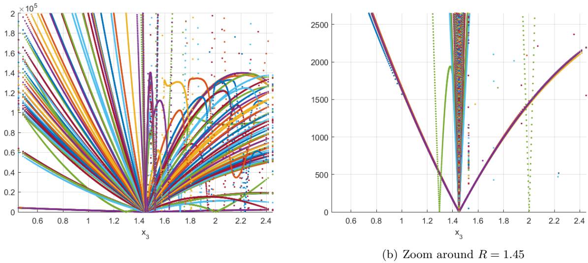
Figure 14.4: Plot of the criteria J(\cdot, t) on the grid with G = 1 at each iteration where \hat{R} is updated, i-e every dt_R = 0.1 .
