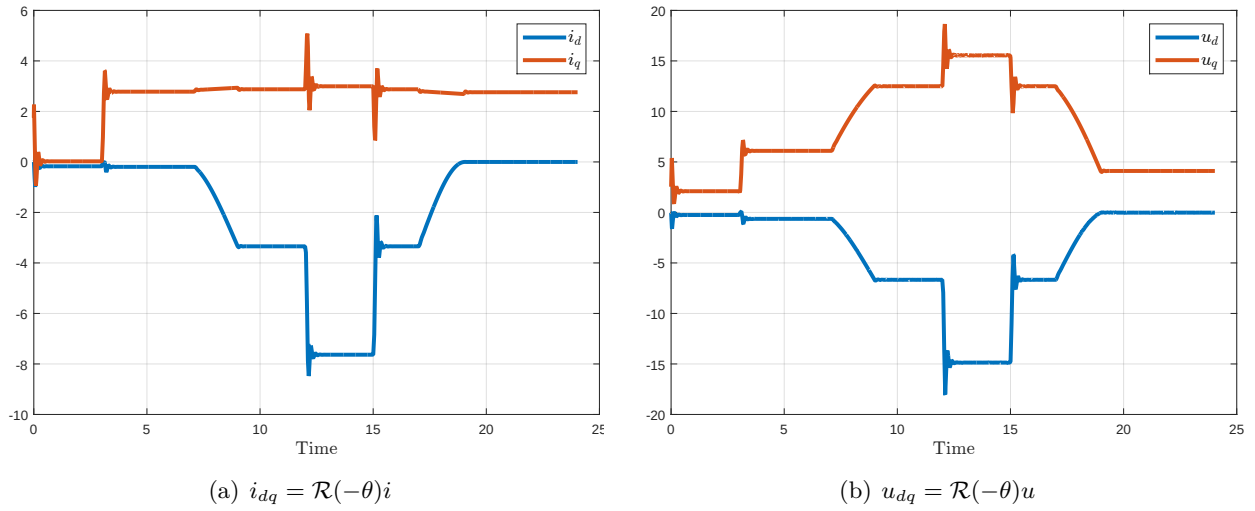
Figure 14.2: Currents and voltages in the rotating frame.
