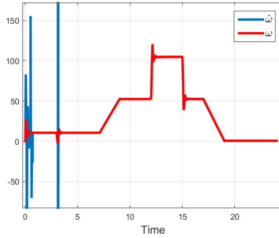
Figure 14.1: Rotation speed \omega = \dot{\theta} and estimated rotation speed \hat{\omega} = \dot{\hat{\theta}} . The estimation algorithm starts at t = 0.5 .
