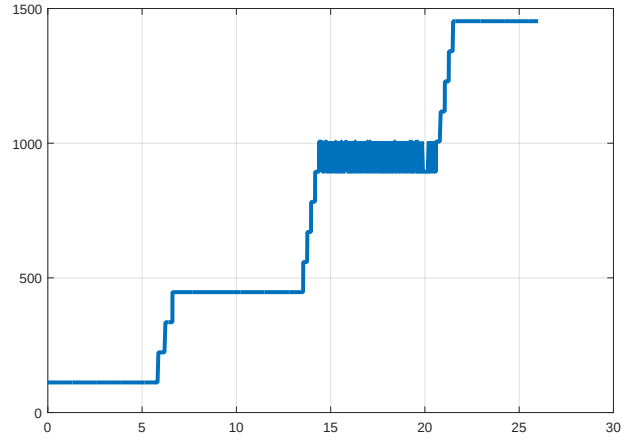
Figure 13.1: Regime of Motor 1 (rpm).
