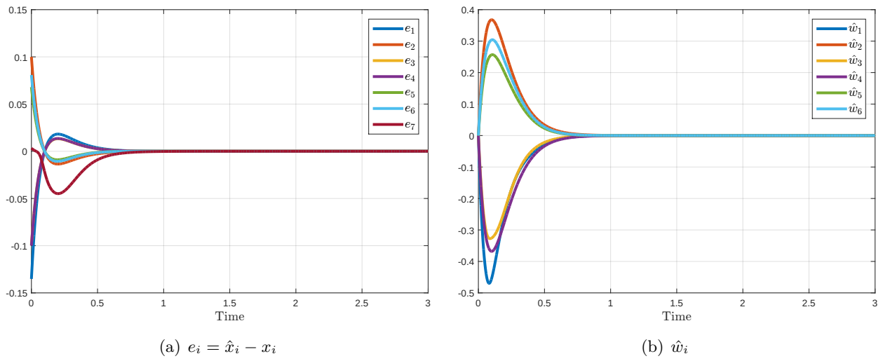
Figure 11.3: Observer (11.23) with L = 10 and k_1 = k_2 = 1 . The simulation was run on Simulink.
