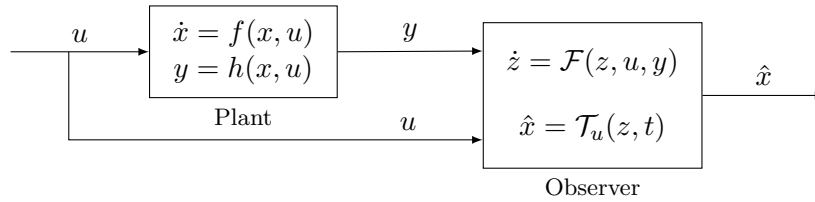
Figure 2.1: Observer : dynamical system estimating the state of a plant from the knowledge of its output and input only.
