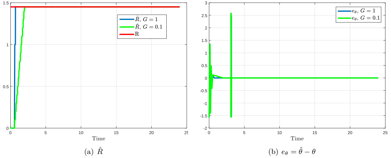
Figure 14.3: Results of the observer algorithm with \lambda_1 = 20 , \lambda_2 = 30 , \lambda_3 = 40 , dt_R = 0.1 , and two grids with amplitude G = 1 and G = 0.1 respectively. The estimation starts at t = 0.5 .
