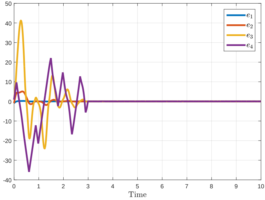
Figure 4.2: Convergence of an homogeneous observer with degree -1 in the absence of noise ( e_i = \hat{\xi}_i - \xi_i )
