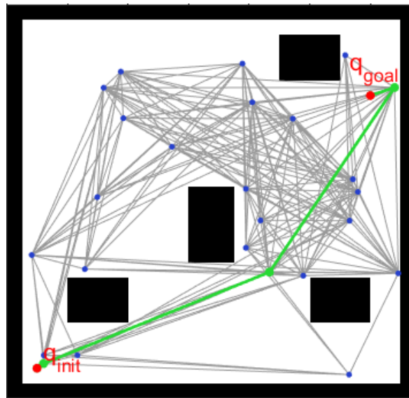
Figure 3.8 – Probabilistic Roadmap Method: the green path joins the initial and final configurations. The expanded graph is shown in grey.
