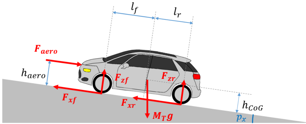
Figure 2.5 – Forces applied on a vehicle.
